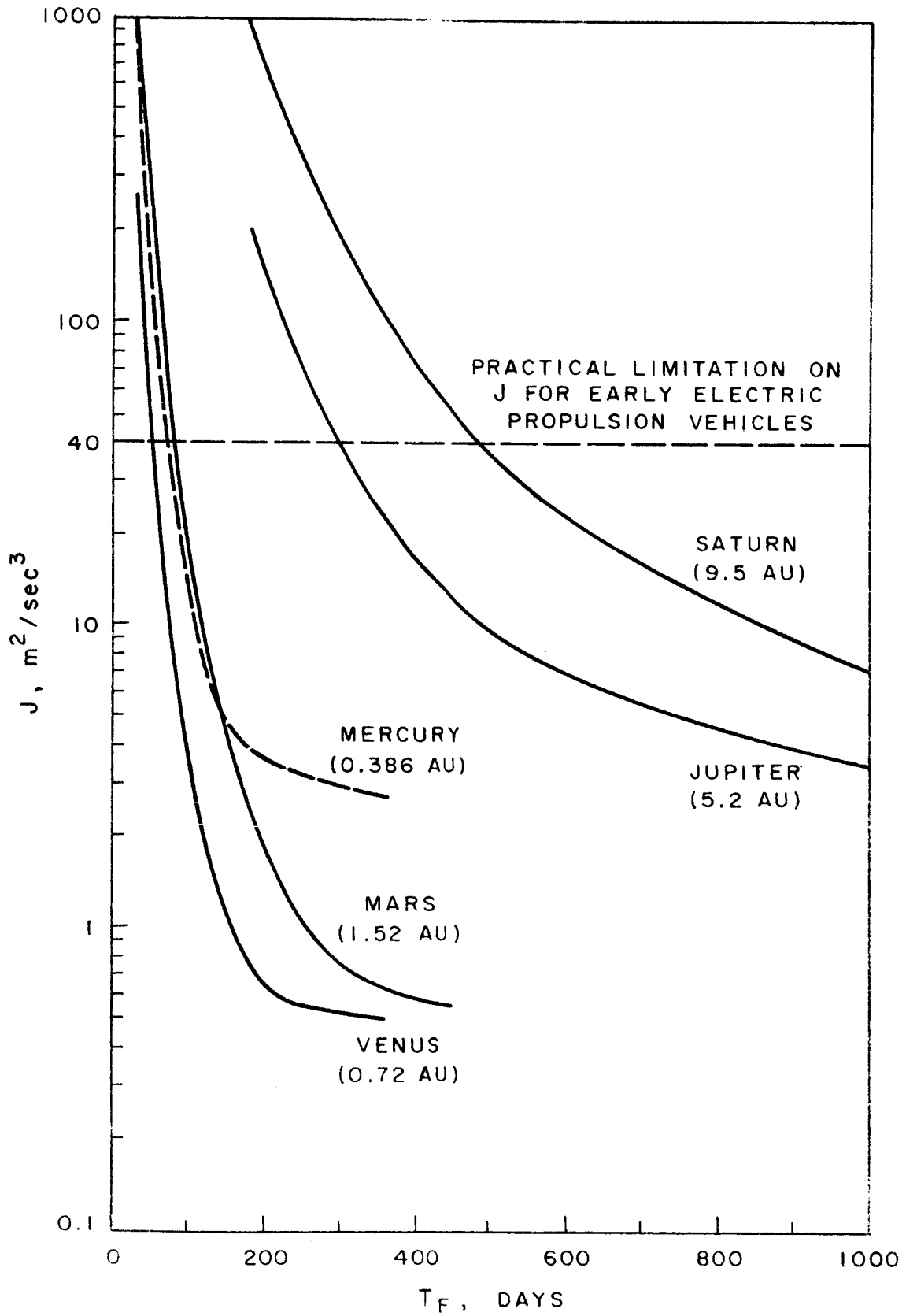
FIGURE 8 EFFECT OF FLIGHT TIME ON J REQUIREMENTS FOR PLANETARY FLY-BY, VARIABLE THRUST MODE
