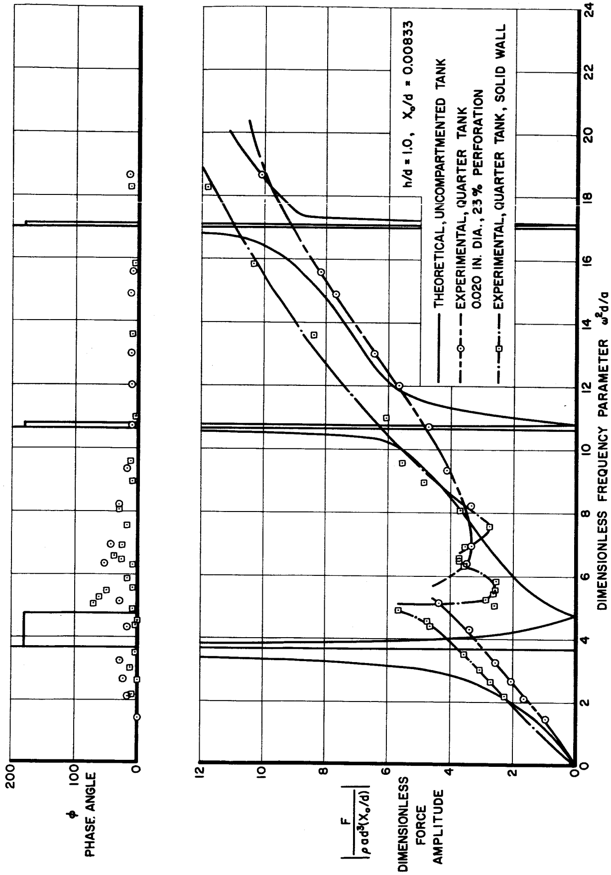
FIGURE 5. TOTAL FORCE RESPONSE FOR A QUARTER TANK WITH PERFORATED SECTOR WALLS
