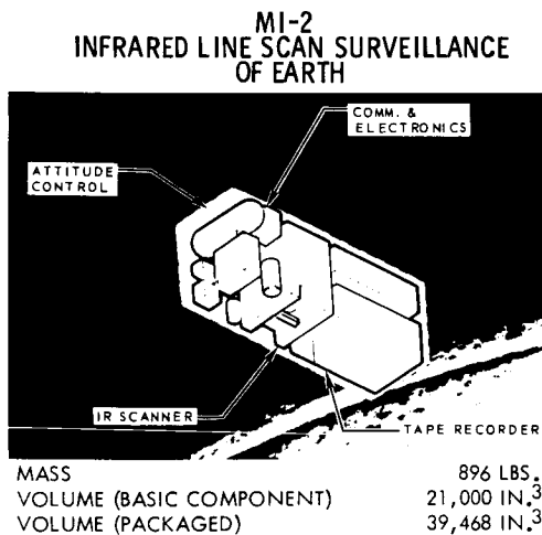
Figure 6-14 EXPERIMENT MI-2 CONFIGURATION
