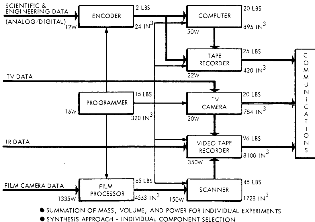
Figure 4-2 DATA AUTOMATION
