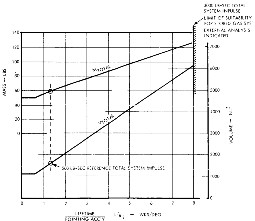
Figure 8-3 ATTITUDE CONTROL SYNTHESIS
