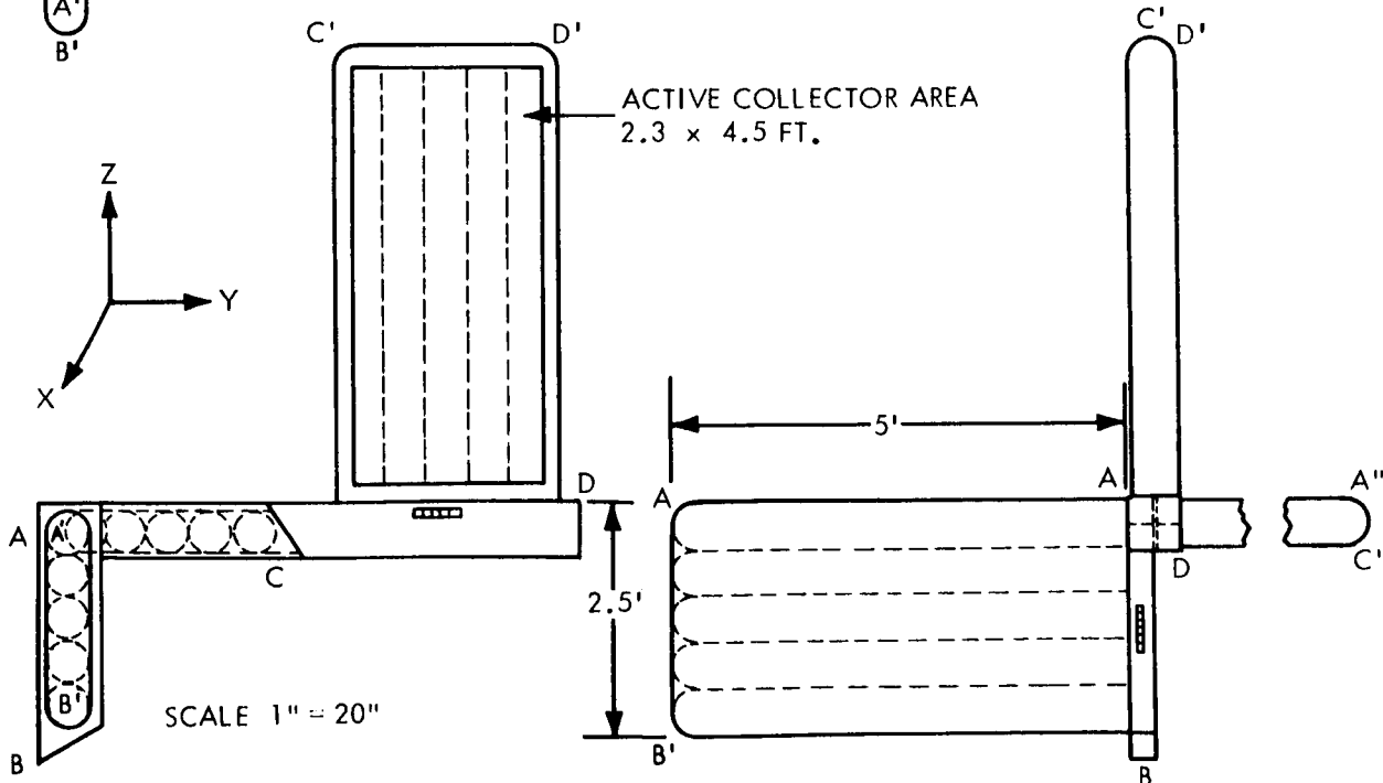
Figure A.1-2 SDT-2 THIN-FILM CADMIUM - SULPHIDE PHOTOVOLTAIC IN-FLIGHT EXPERIMENT PACKAGE
