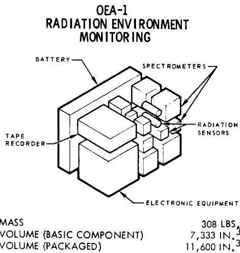
Figure 6-28 EXPERIMENT OEA-1 CONFIGURATION
