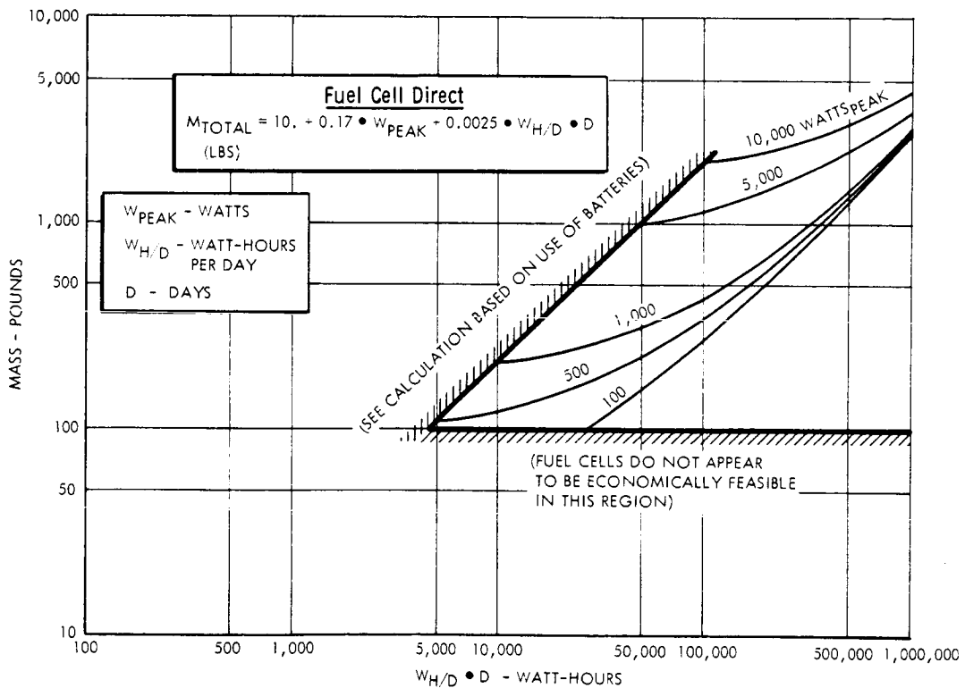
Figure 8-12 ELECTRIC POWER SYSTEM RELATIONSHIPS
