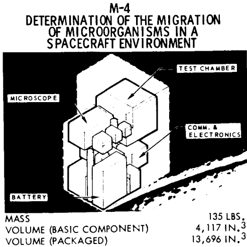
Figure 6-26 EXPERIMENT M-4 CONFIGURATION
