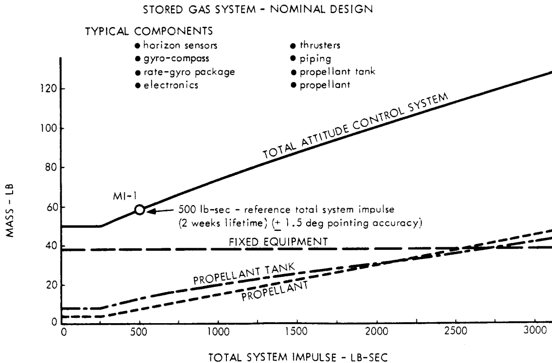
Figure 4-1 ATTITUDE CONTROL
