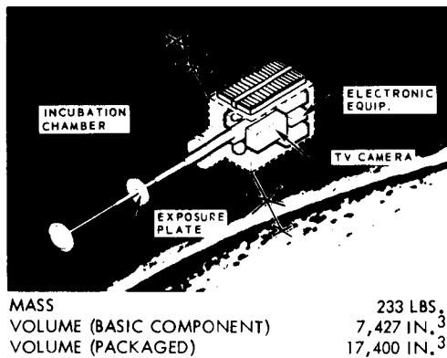
Figure 6-23 EXPERIMENT M-1 CONFIGURATION
