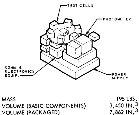
Figure 6-19 EXPERIMENT SLG-2 CONFIGURATION
