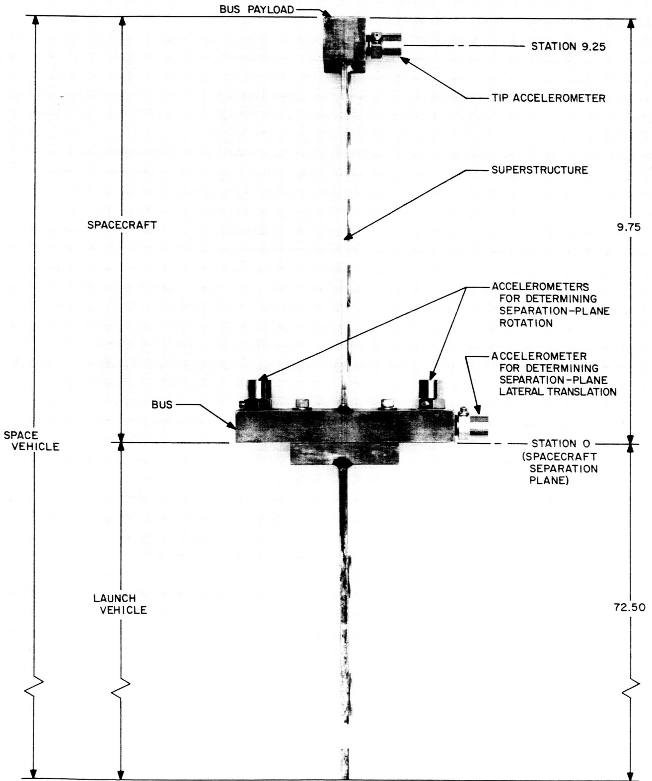
Fig. 2. Structural idealization of a laterally-flexible space vehicle
