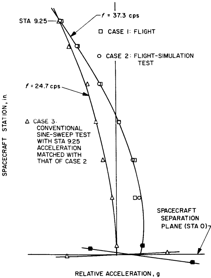
Fig. 9. Spacecraft acceleration distributions in flight and in shake-table tests
