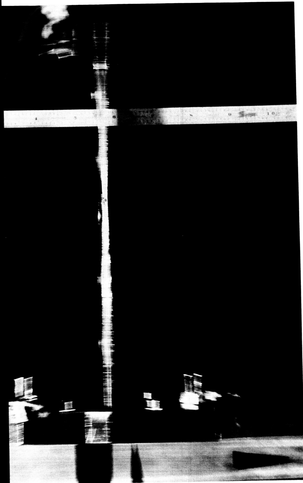
Motion on tuned, rocking shake table adjusted to give separation-plane motions of the 4 th bending mode of the space vehicle, Case 2
