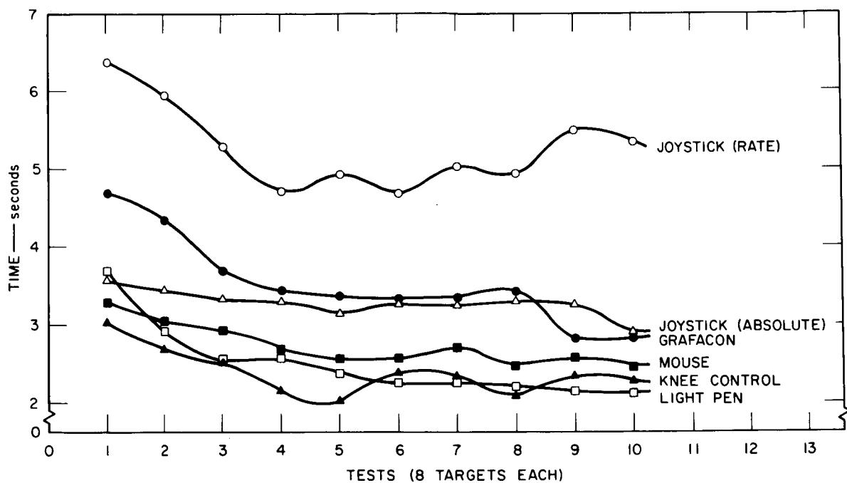
FIG. 12 COMPOSITE LEARNING CURVES
