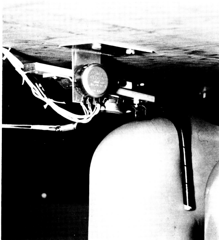
FIG. 15 KNEE CONTROL BUG-POSITIONING DEVICE
