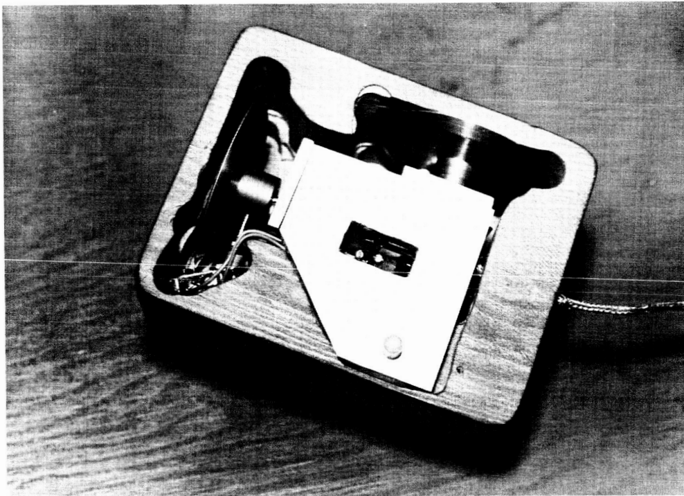
FIG. 14 BOTTOM SIDE OF MOUSE, SHOWING MECHANICAL DETAILS
