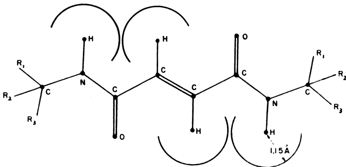
Cisoid Conformation
