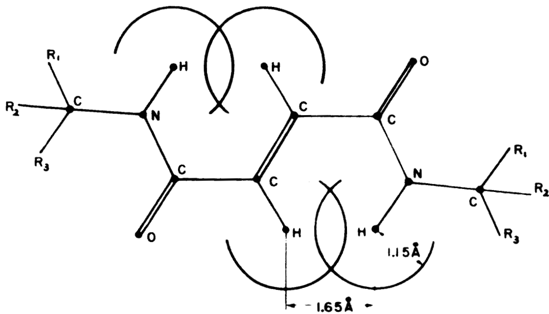
Transoid Conformation
