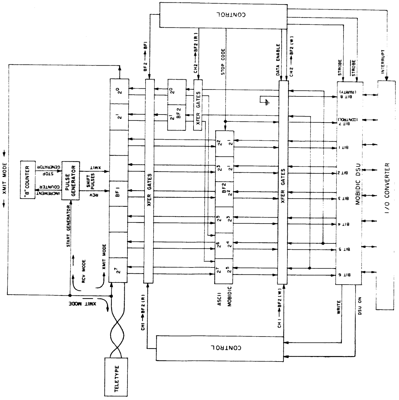
FIGURE 3. MOBIDIC-TELETYPE INTERFACE BLOCK DIAGRAM
