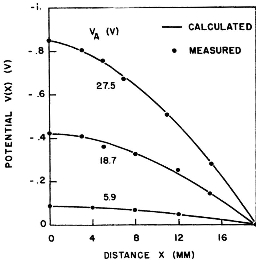
FIGURE 3. Potential Profiles Under Dark, Reverse Biased Condition
