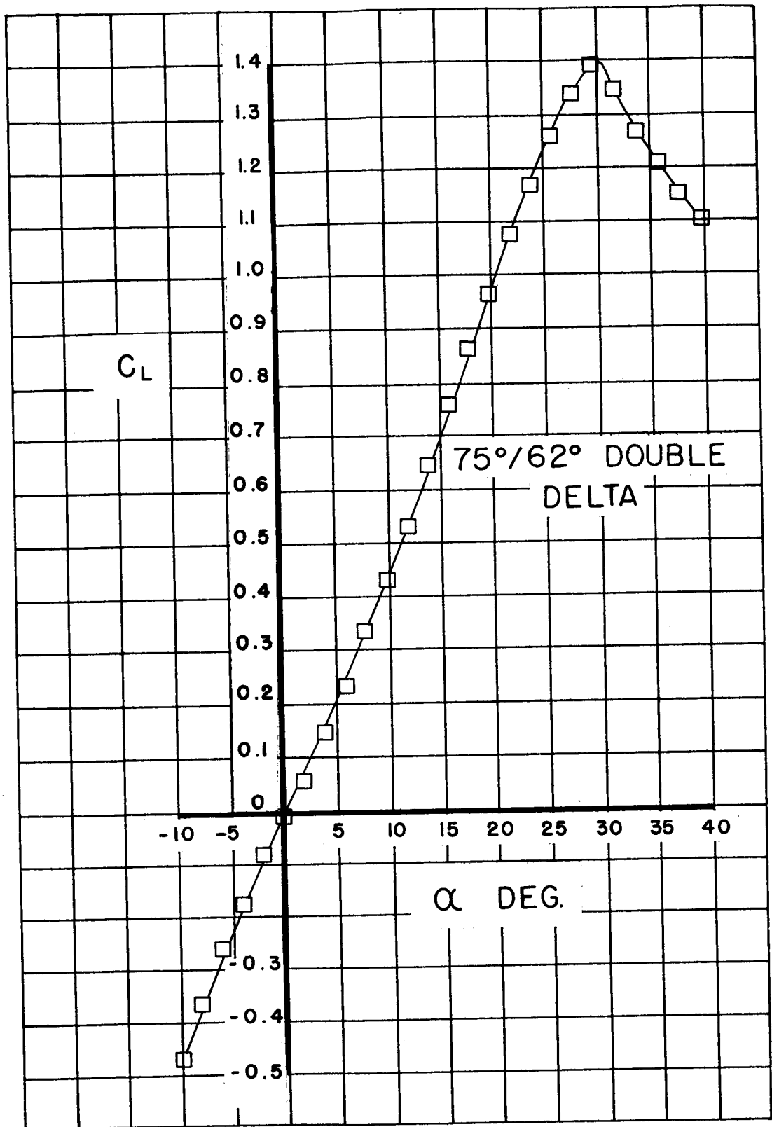
Figure 17a.- C_L vs alpha 75^\circ/62^\circ double-delta wing.
