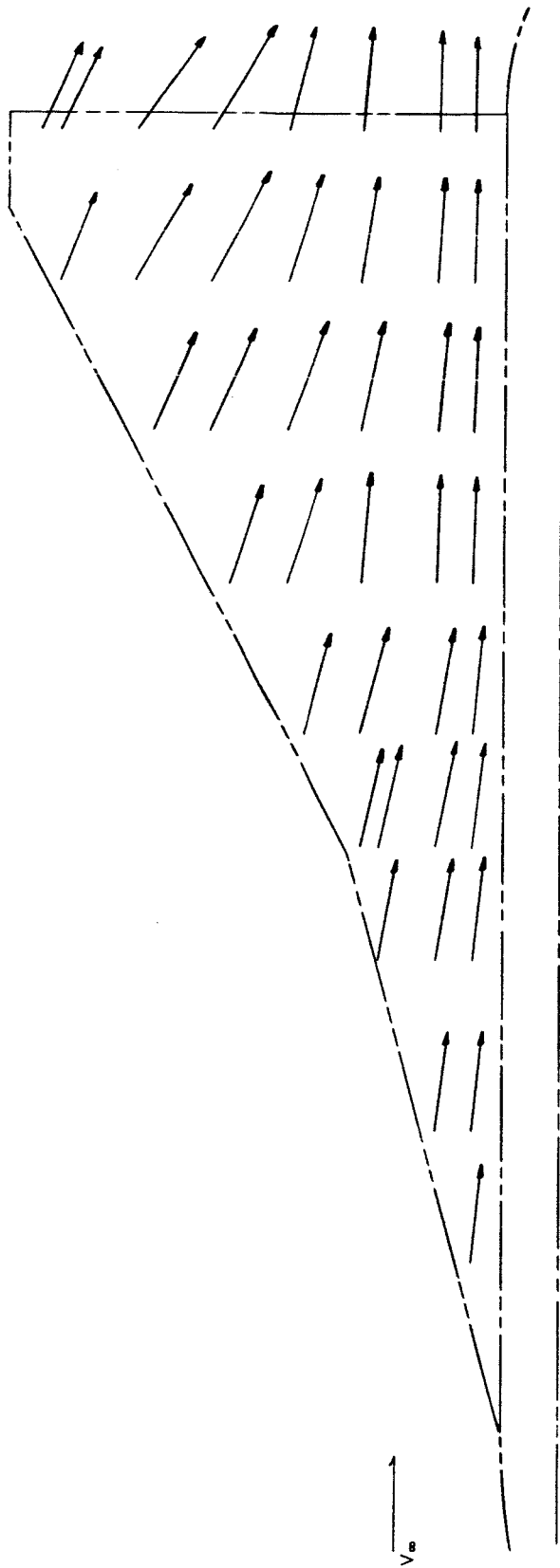
Figure 141.- Upper surface flow field. \alpha = +20^\circ ; z/b = -0.411 .
