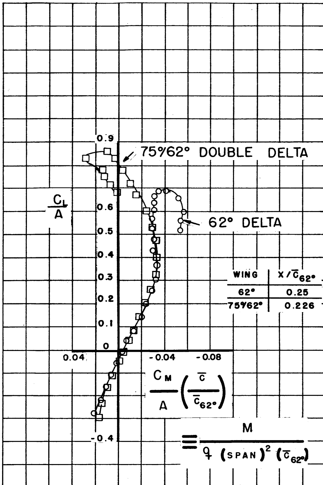
Figure 18c:- C_L/A vs (C_M/A) (\bar{c}/\bar{c}_{62^\circ}) 62° delta and double-delta wings.
