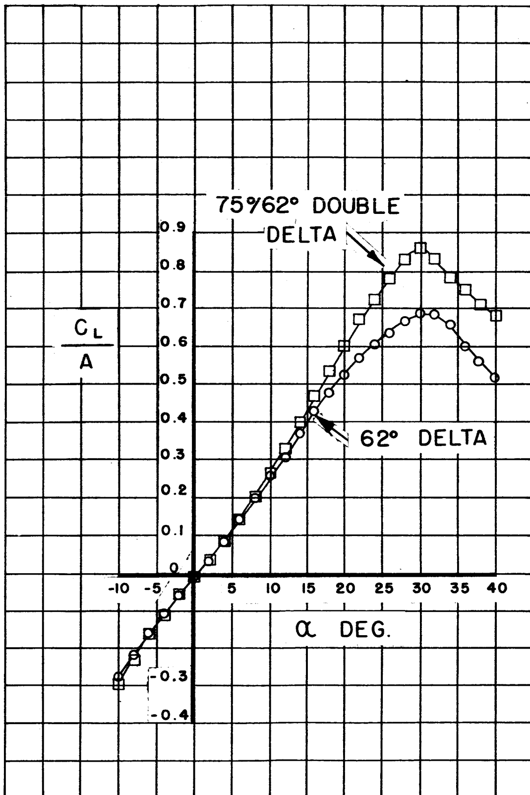
Figure 18a.- C_L/A vs \alpha 62^\circ delta wing and 75^\circ/62^\circ double-delta wing.
