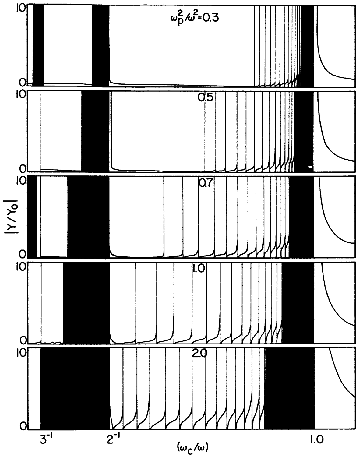
Fig. 5(a). Coaxial cylinder capacitor - Normalized admittance variation with (\omega_c/\omega) and (\omega_p^2/\omega^2) for (v_T/h\omega) = 0.02 , (b/a) = 3.0 , (a) (v/f_c) = 0
