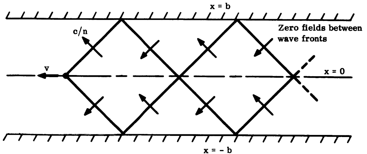
FIG. 3: SHOCK WAVE GEOMETRY, PARALLEL PLATE BOUNDARY
