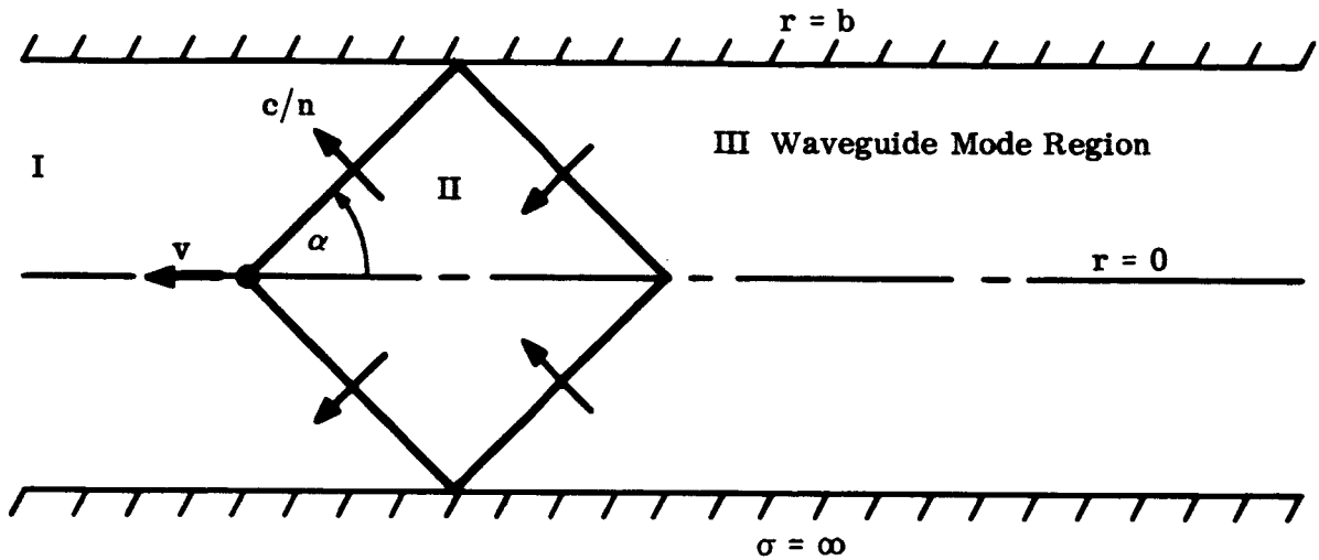
FIG. 2: SHOCK WAVE GEOMETRY, CYLINDRICAL BOUNDARY
