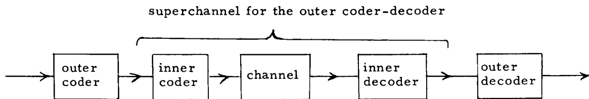
Fig. 9. Forney coding-decoding.
