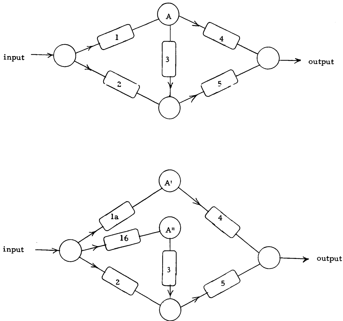
Fig. 11. Node splitting.
