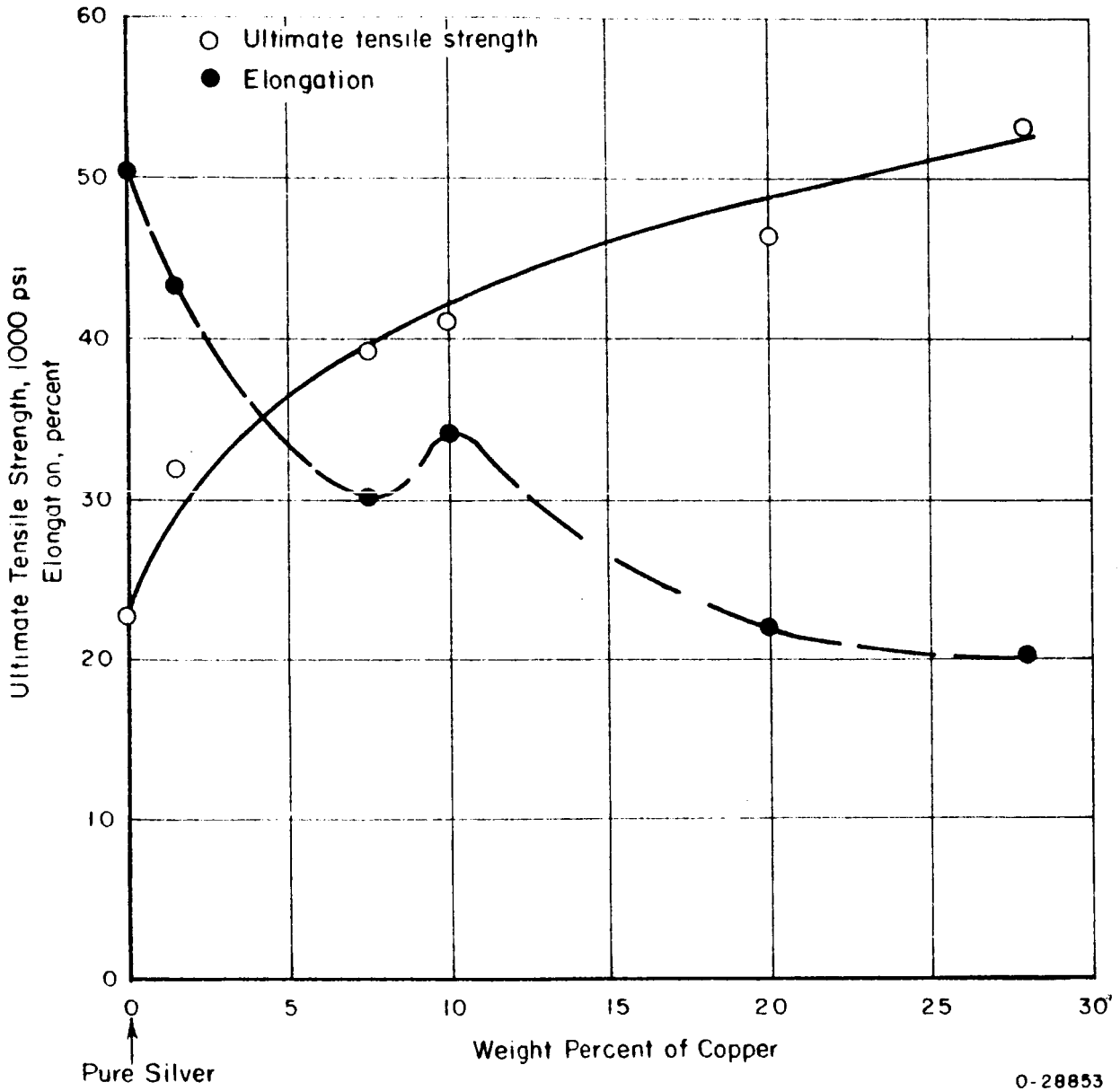
FIGURE B-8. TENSILE PROPERTIES OF ANNEALED SILVER-COPPER ALLOYS
