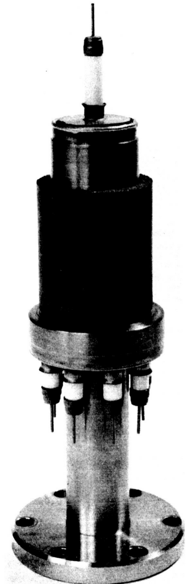
Fig. 8 Photograph of the hot-cathode magnetron with magnet in place. The tubulation is 2.5 cm in diameter by 8 cm long.
