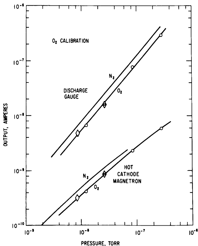
Fig. 17 Calibration curves obtained with \text{O}_2 . The applicable \text{N}_2 calibration is also shown for comparison. Emission of hot-cathode magnetron was 1 \times 10^{-7} amp (magnet off): \circ = pressure increasing, and \diamond = pressure decreasing.
