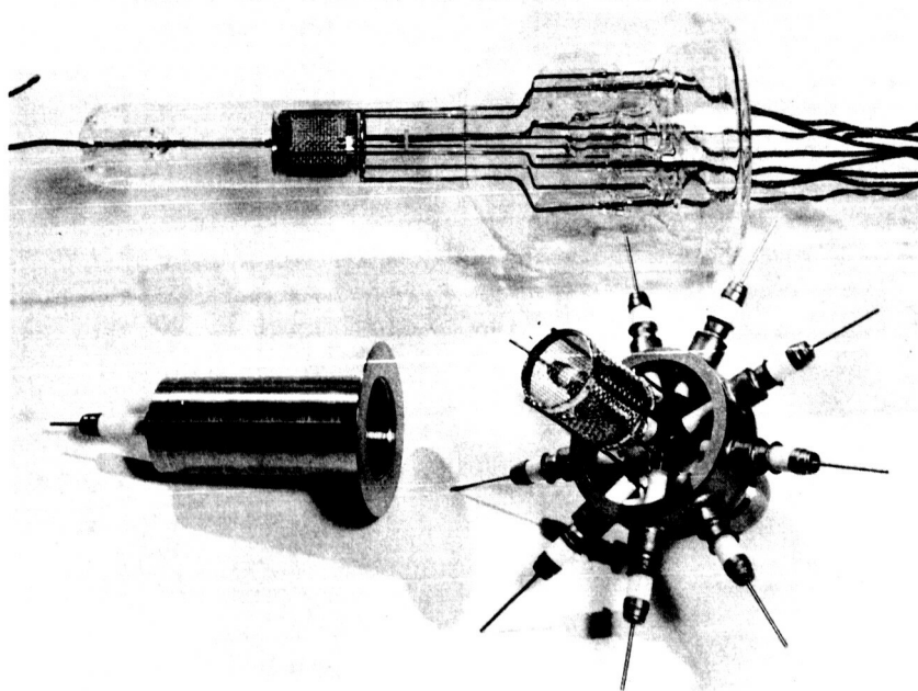
Fig. 22 Photograph of flight model and all-glass versions of the hot-cathode magnetron gauge.
