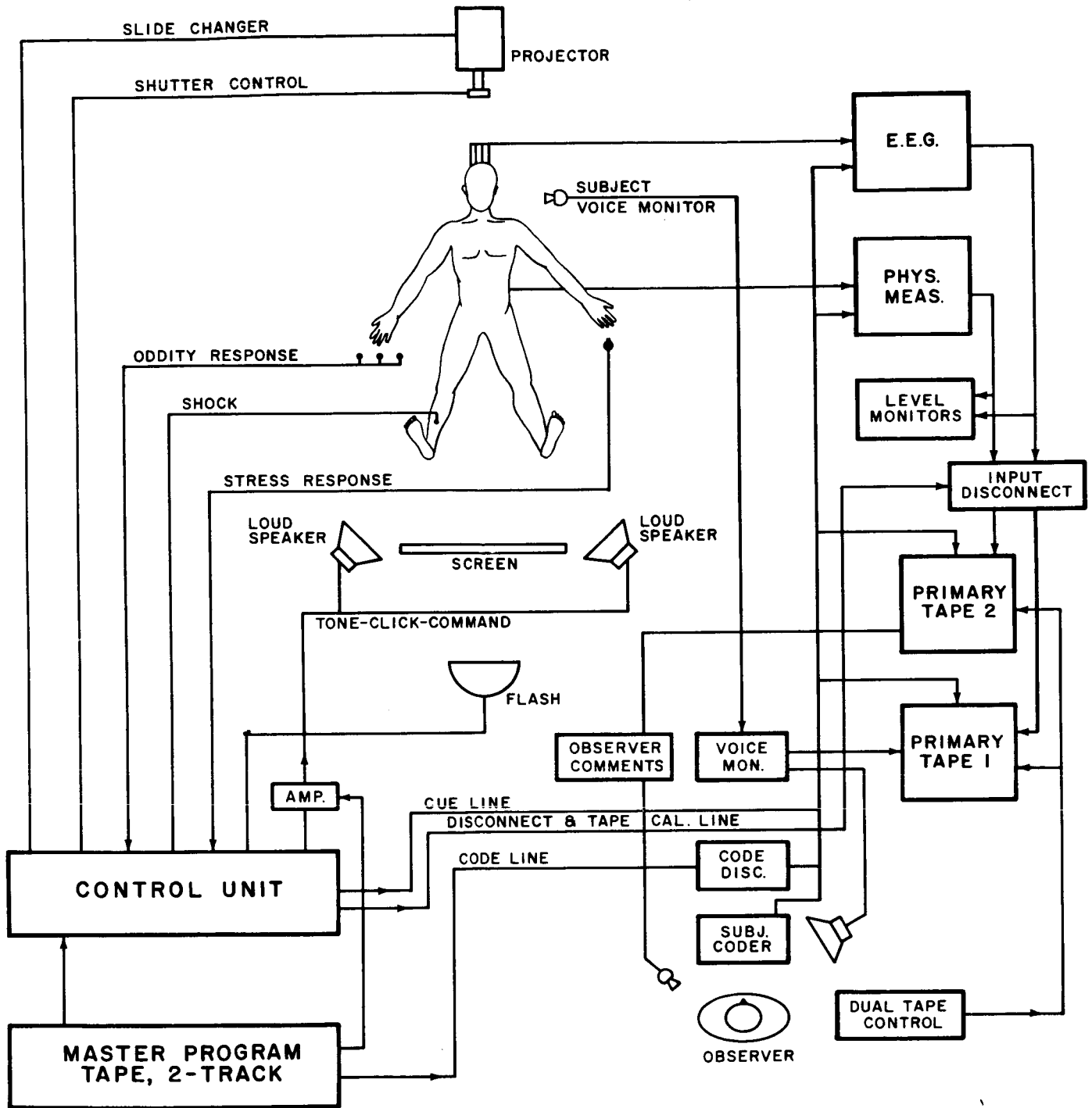
PSYCHO-PHYSIOLOGICAL TESTING AND DATA ACQUISITION SYSTEM BLOCK DIAGRAM
