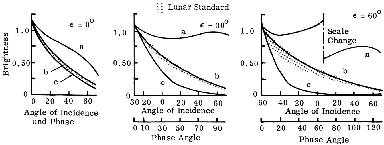
d. Angle of Incidence and Phase Angle vs Brightness
