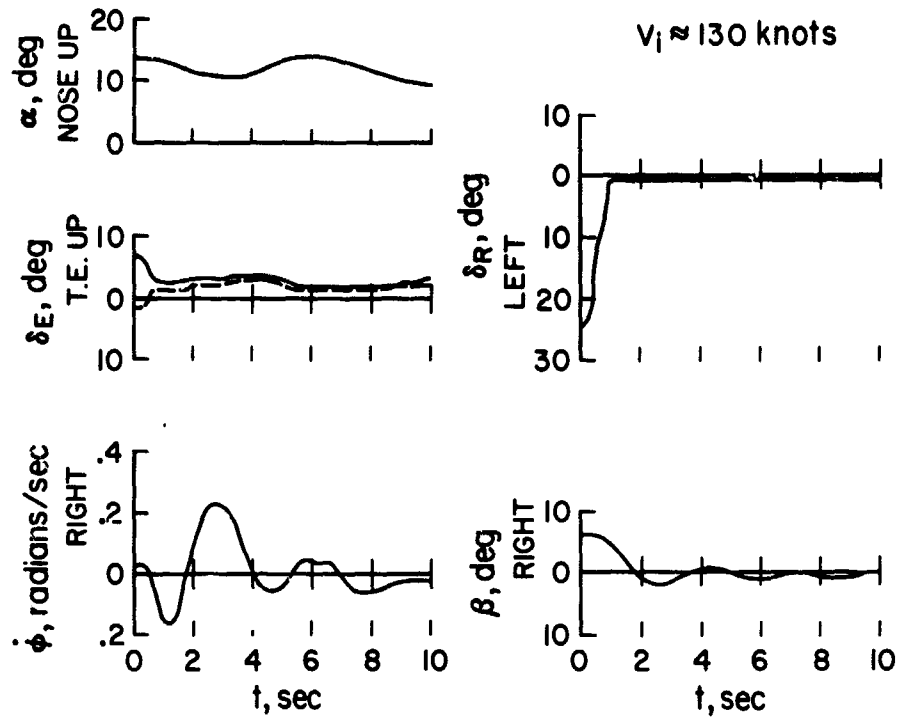
Fig. 6 Lateral-directional oscillation, V_1 \approx 130 knots
