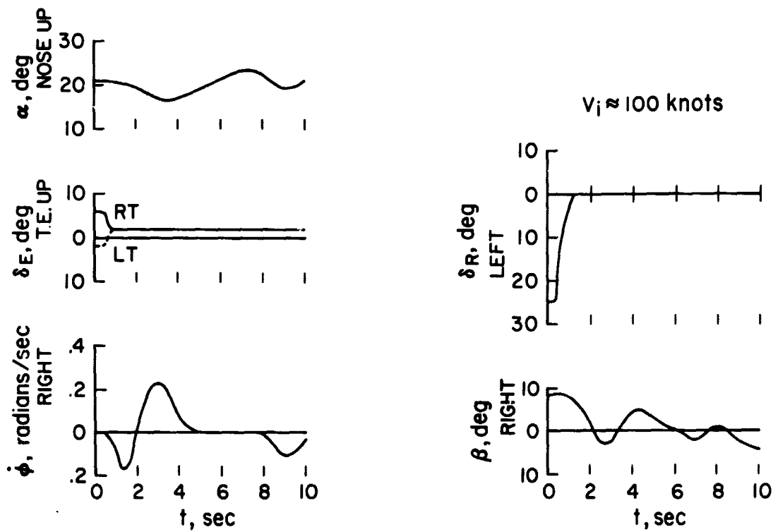
Fig. 7 Lateral-directional oscillation, V_1 \approx 100 knots
