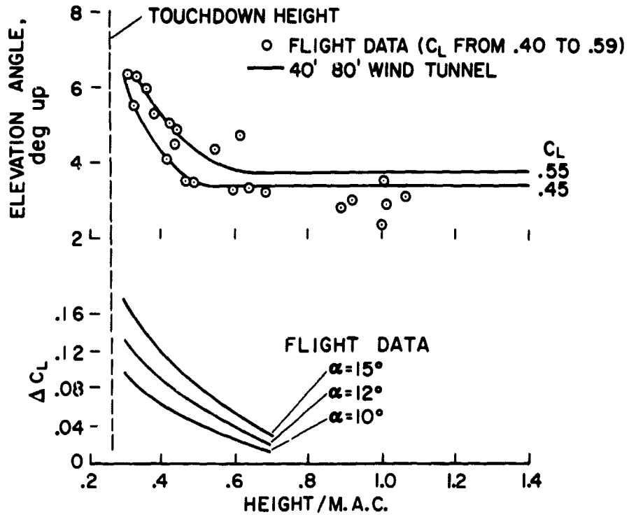
Fig.10 Ground-effect measurements
