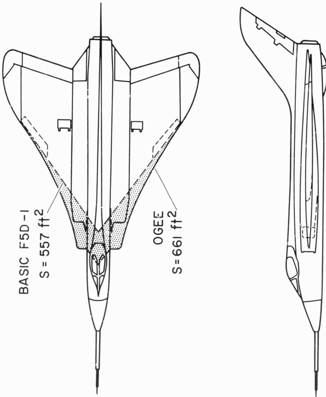
Fig.1 Test airplane
