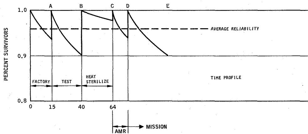
Figure 2. Reliability Curves of Semiconductor System Containing 20,000 Parts (Series)
