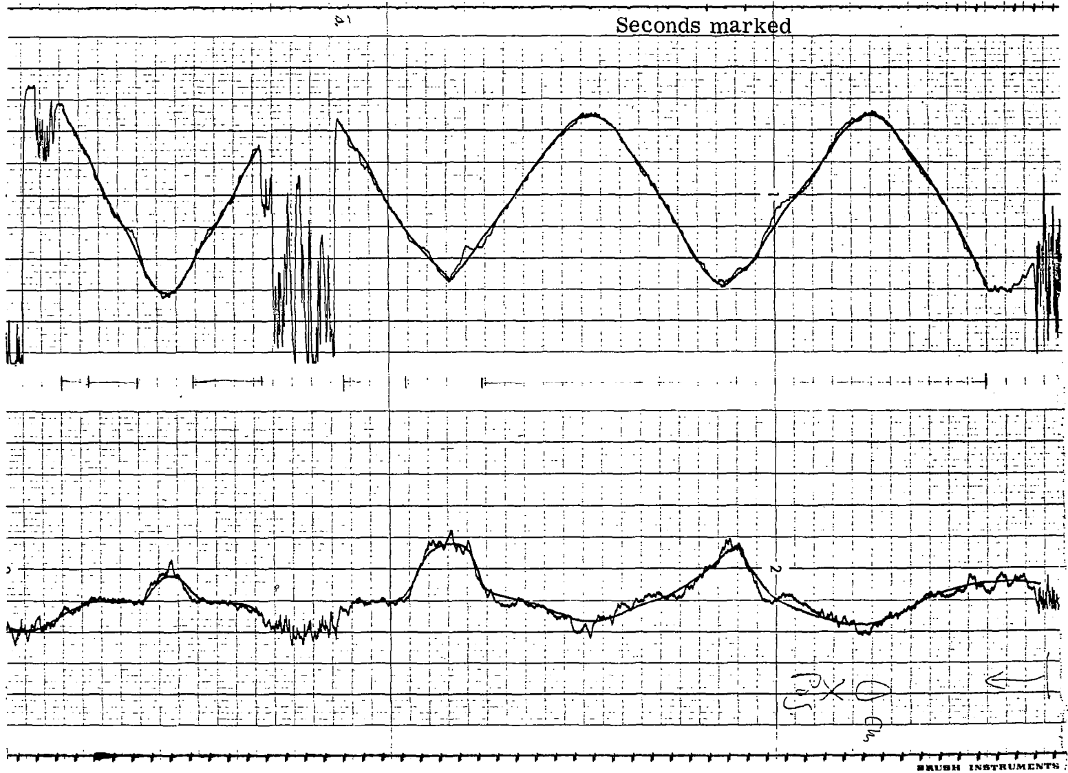
Figure 4.21 OCULOMETER OUTPUT WITH EYE TRACKING A Y = 40^\circ , X = 0 , PEAK-TO-PEAK STIMULUS MOTION
