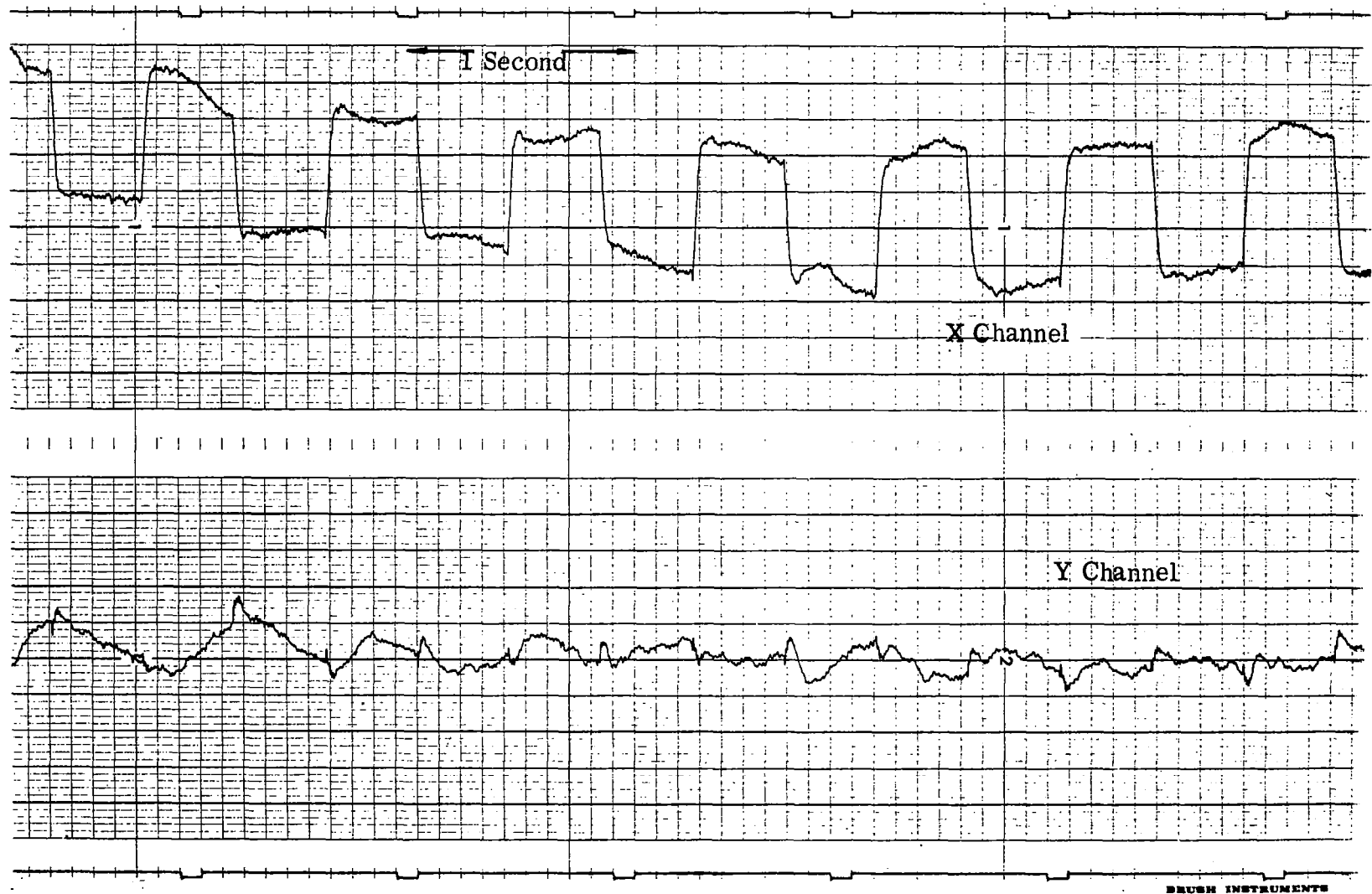
Figure 4.5 CLOSED LOOP RESPONSE OF CORNEAL POSITION LOOP TO VIRTUAL 0.6 mm STEP DISPLACEMENT AT THE EYE (Corneal integrator output at 100 mv/line)
