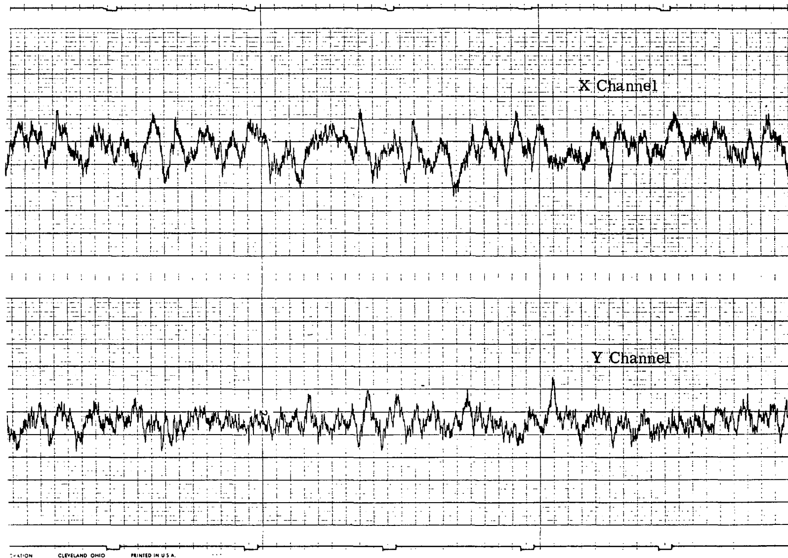
Figure 4.9 CORNEAL INTEGRATOR OUTPUT WHEN TRACKING REFLECTION IN ARTIFICIAL PUPIL -- 20 mv/line
