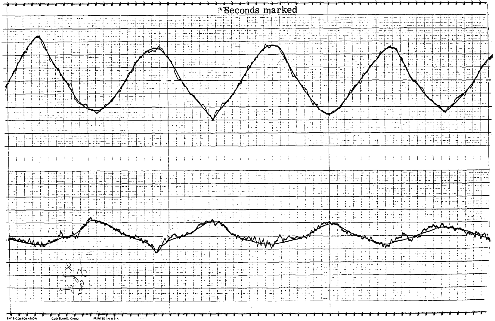
Figure 4.23 OCULOMETER OUTPUT WITH EYE TRACKING AN x = -7^\circ , Y = 40^\circ , PEAK-TO-PEAK STIMULUS MOTION
