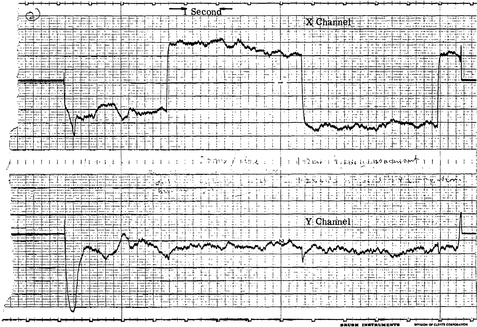
Figure 4.4 CLOSED LOOP RESPONSE OF PUPIL POSITION LOOP TO VIRTUAL 2.4 mm STEP DISPLACEMENT AT THE EYE (Pupil integrator output at 50 mv/line)
