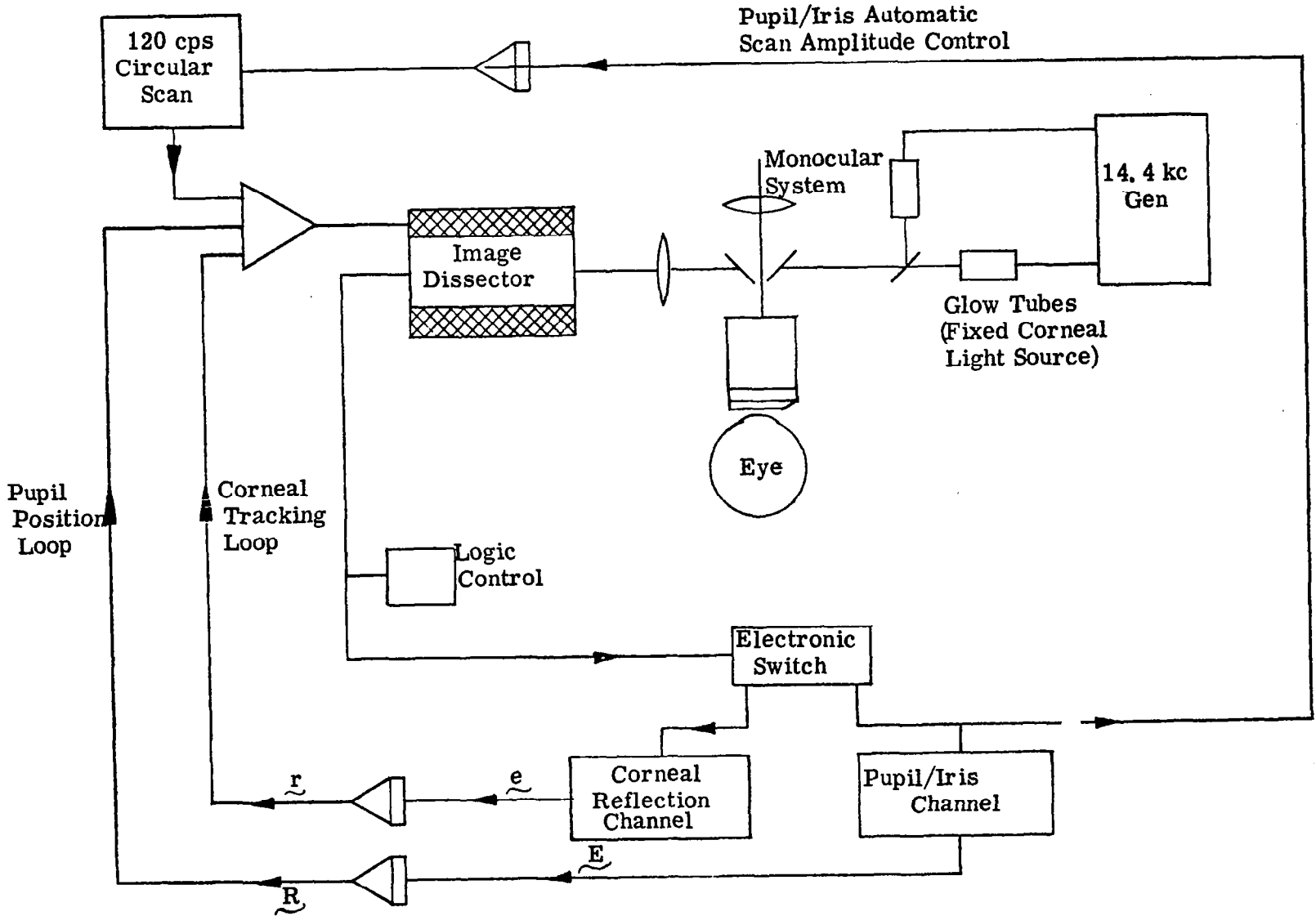
Figure 3.17 OCULOMETER BLOCK DIAGRAM
