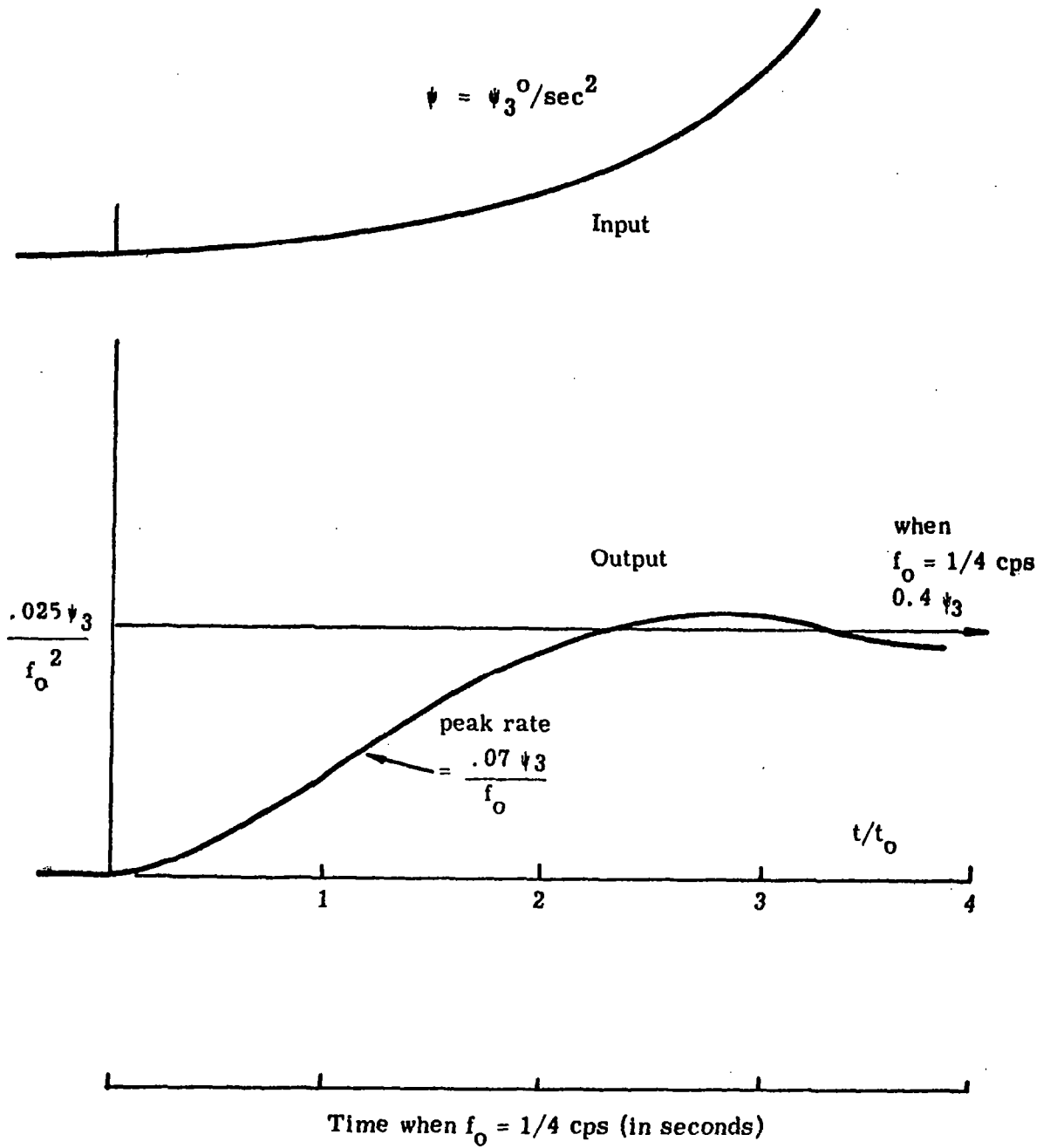
Figure A.6 RESPONSE TO AN ACCELERATING RAMP INPUT
