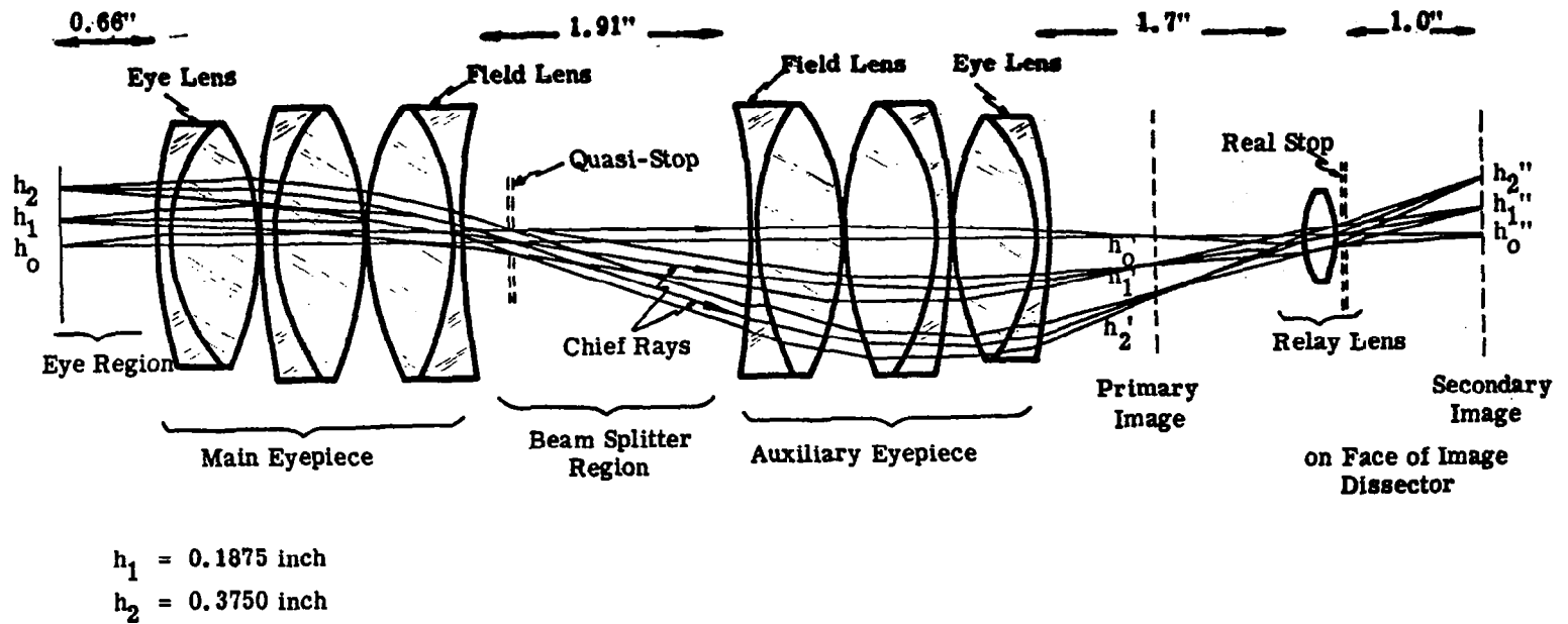
Figure 3.7 IMAGE DISSECTOR SYSTEM (UNFOLDED)
