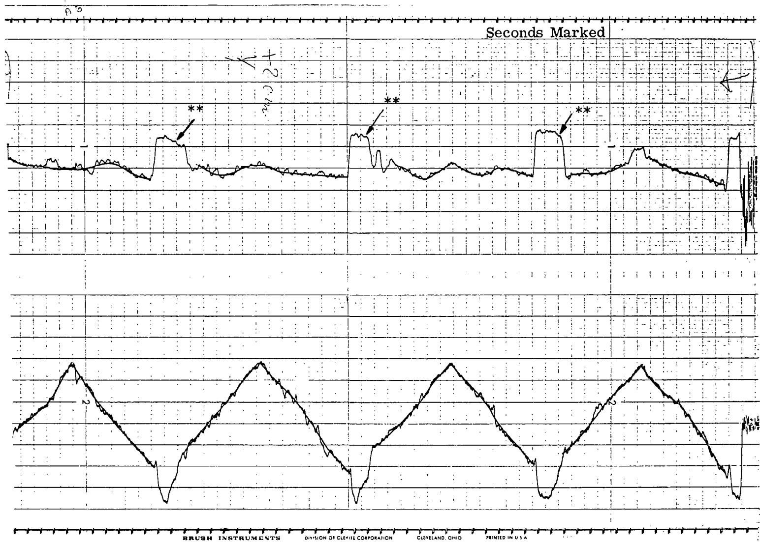
Figure 4.17 OCULOMETER OUTPUT WITH EYE TRACKING A Y = +7°, X = 35°, PEAK-TO-PEAK SAWTOOTH STIMULUS MOTION
