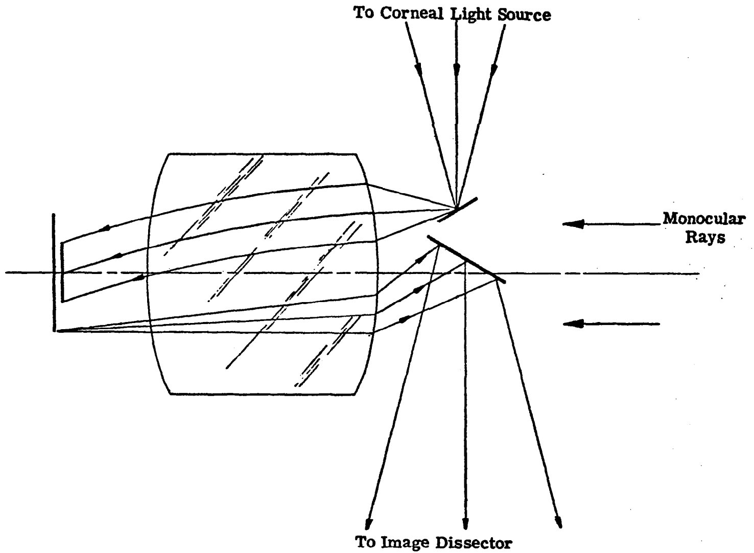
Figure 3.5 LOCATION OF BEAM SPLITTERS
