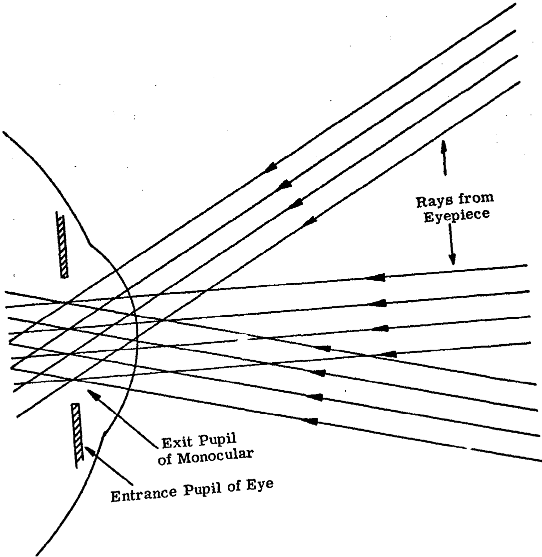
Figure 3.3 POSITION OF EYE RELATIVE TO MONOCULAR EXIT PUPIL
