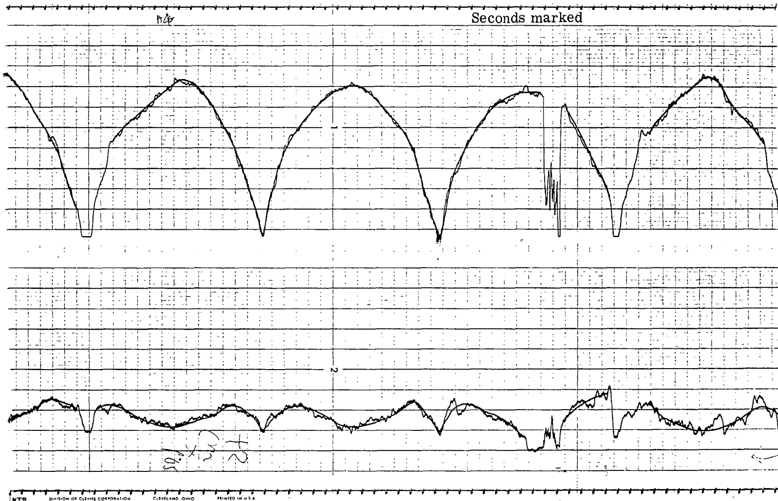
Figure 4.22 OCULOMETER OUTPUT WITH EYE TRACKING AN X = +7^\circ , Y = 40^\circ , PEAK-TO-PEAK STIMULUS MOTION
