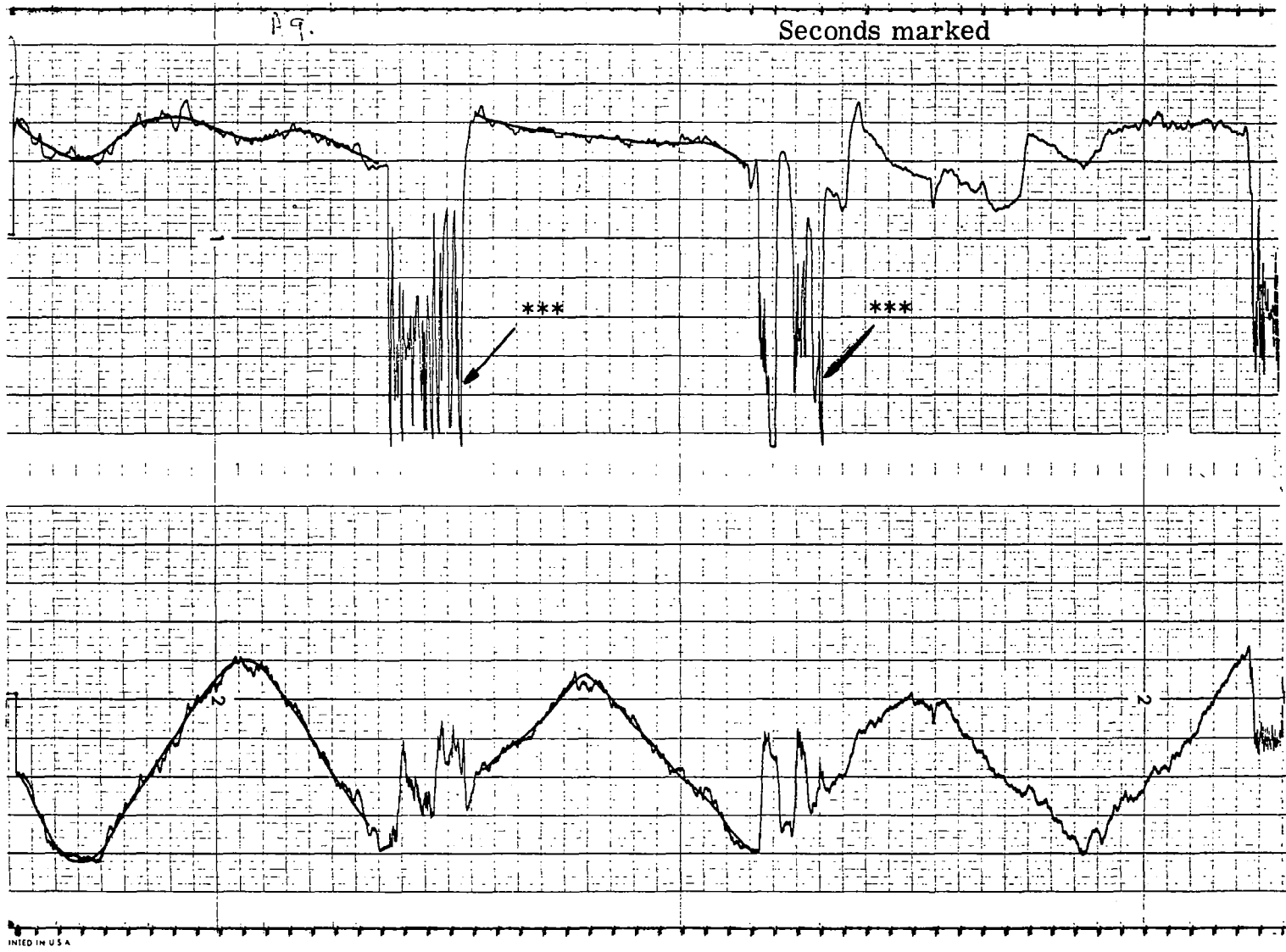
Figure 4.20 OCULOMETER OUTPUT WITH EYE TRACKING A Y = -14°, X = 35°, PEAK-TO-PEAK STIMULUS MOTION
