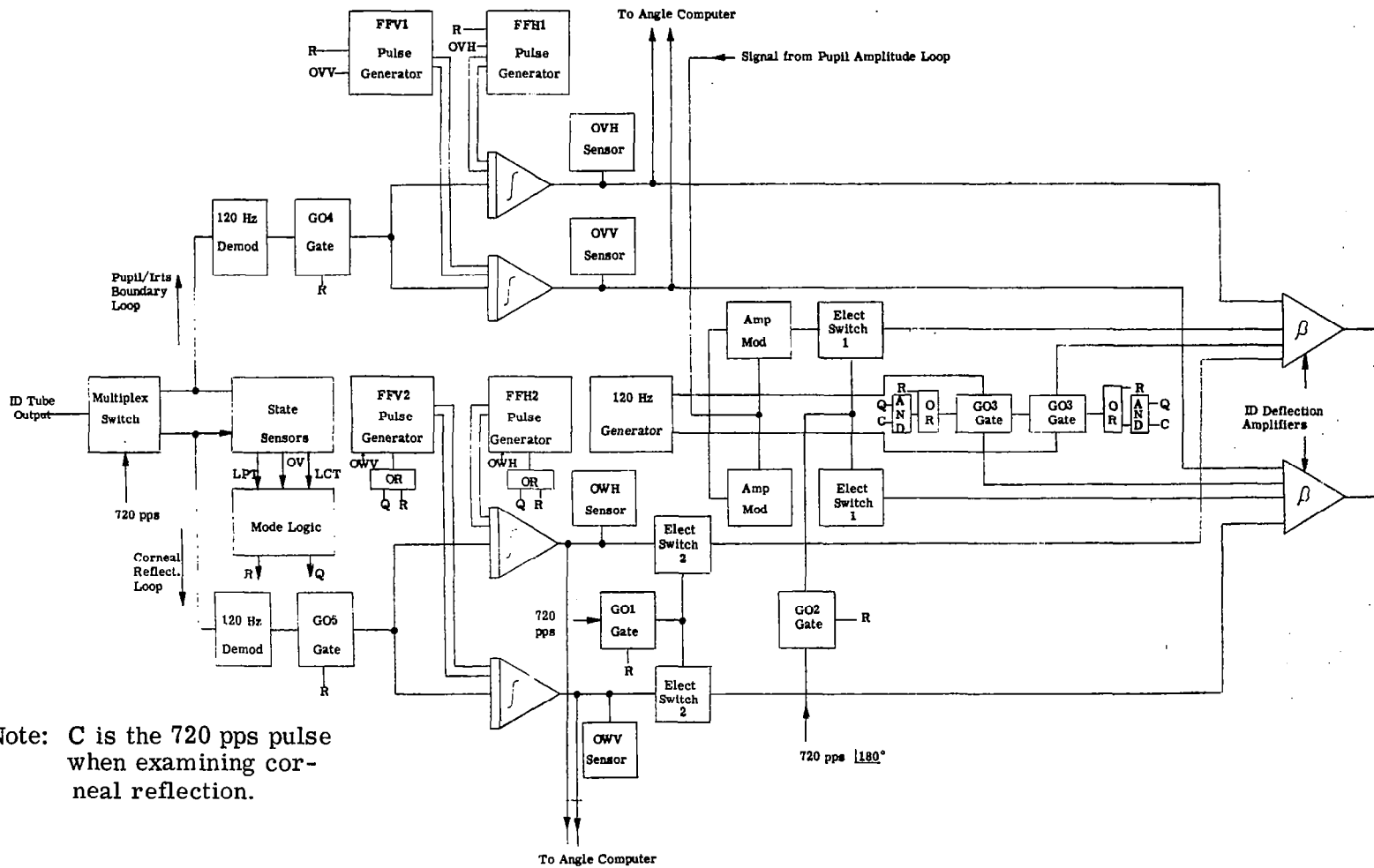
Figure 3.21 AUTOMATIC ACQUISITION SYSTEM BLOCK DIAGRAM
