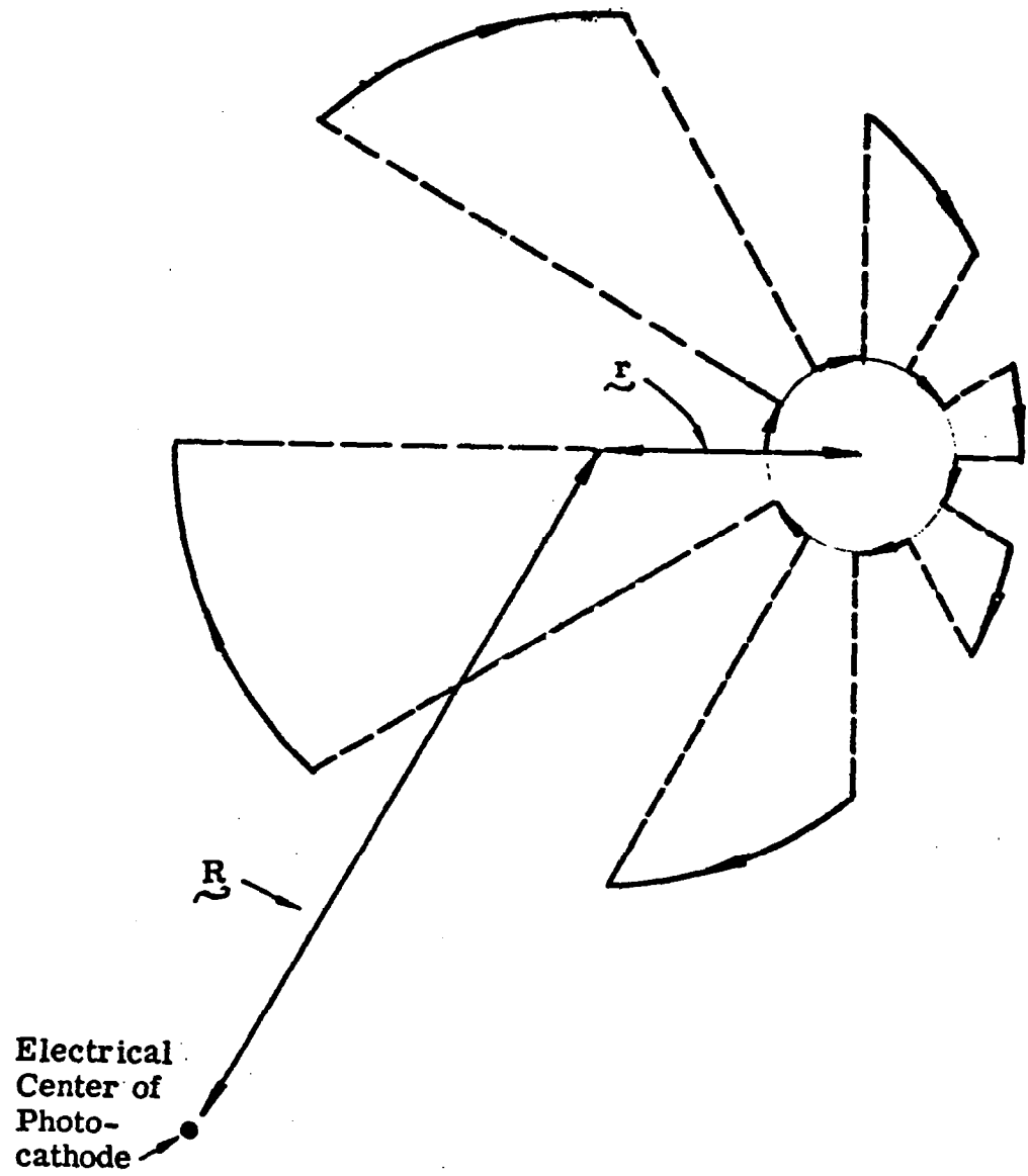
Figure 3.15 ROTATING, TIME-DIVISION-MULTIPLEXED CIRCULAR SCAN
