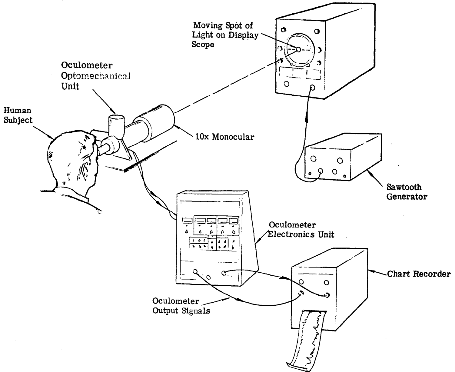
Figure 4.12 EYE TRACKING EXPERIMENTS
