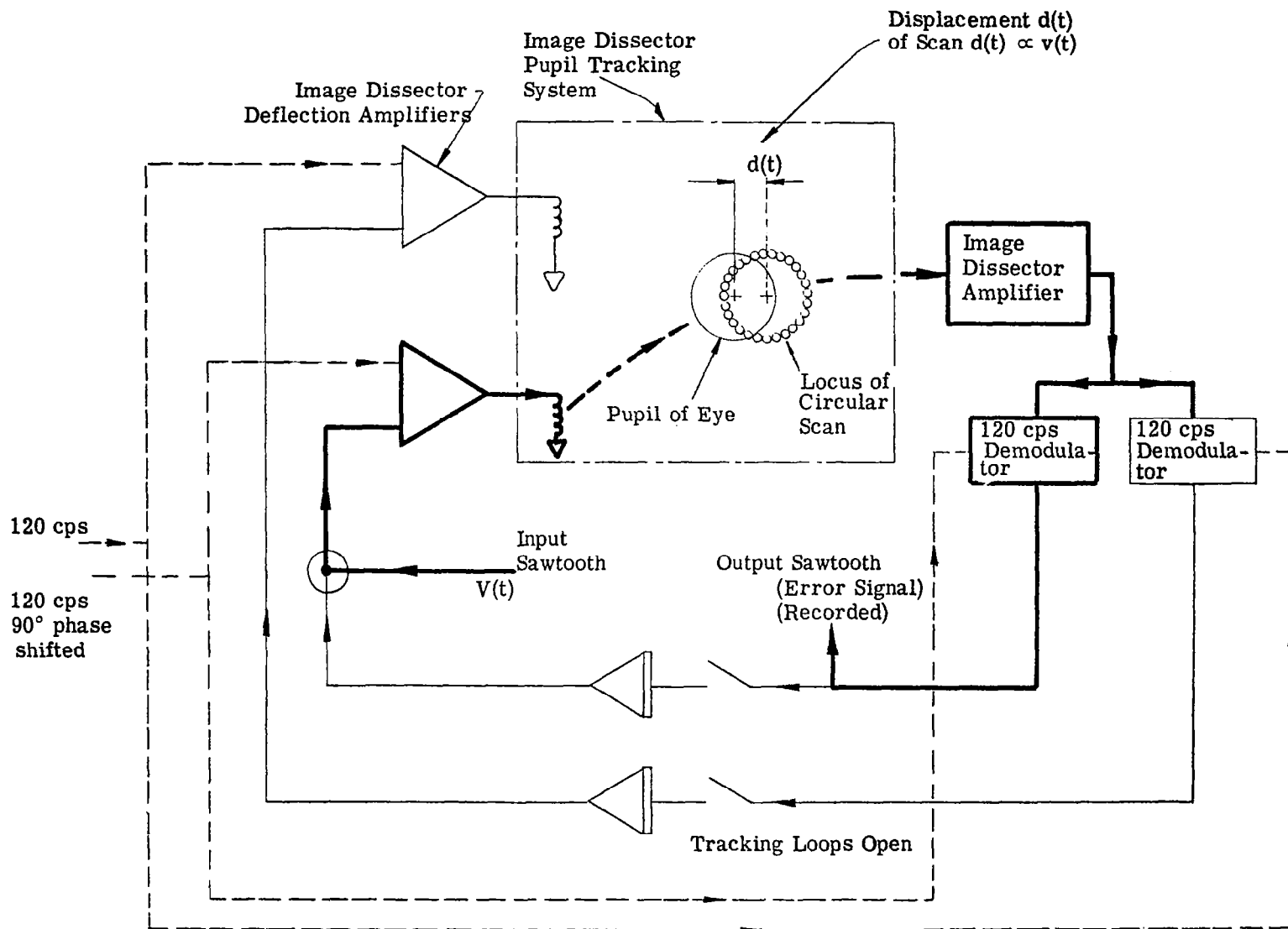
Figure 4. 1 SCHEMATIC OF ERROR SIGNAL TEST
