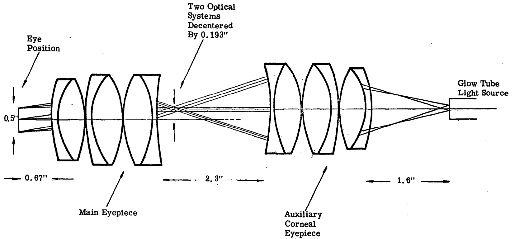
Figure 3.8 CORNEAL ILLUMINATION SYSTEM (UNFOLDED)
