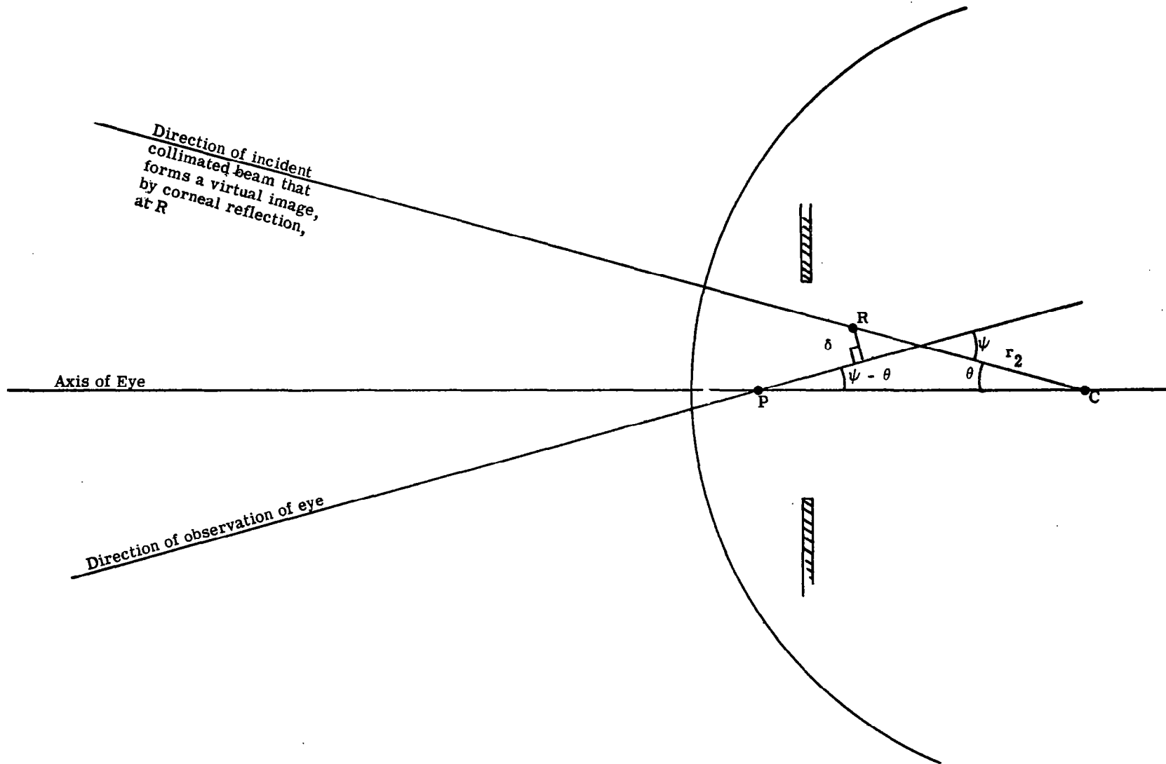
Figure B.1 GEOMETRY OF EYEBALL
