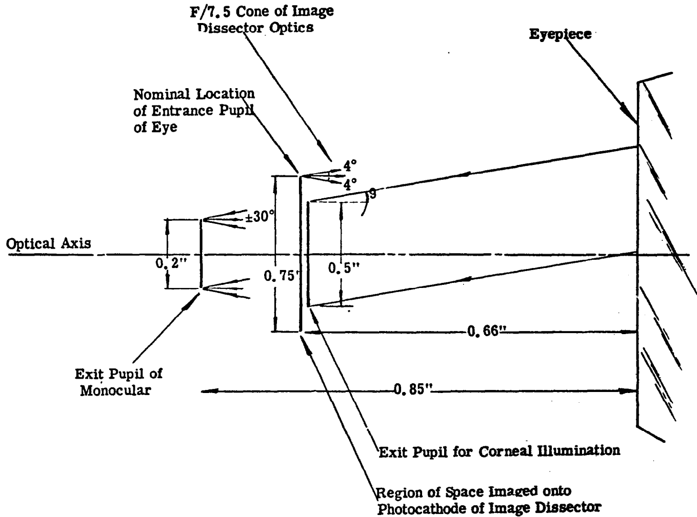
Figure 3.4 OPTICAL PARAMETERS IN RELATION TO EYEPIECE
