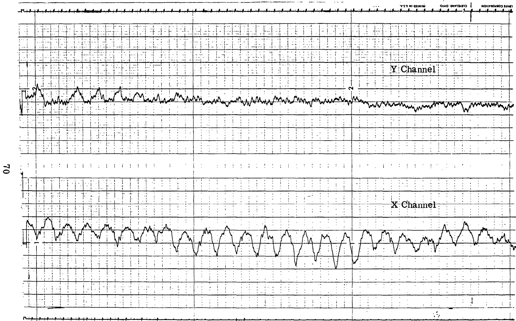
Figure 4.13 EYE DIRECTION MEASURED WITH SAWTOOTH STIMULUS MOTION OF 7^\circ IN X DIRECTION
