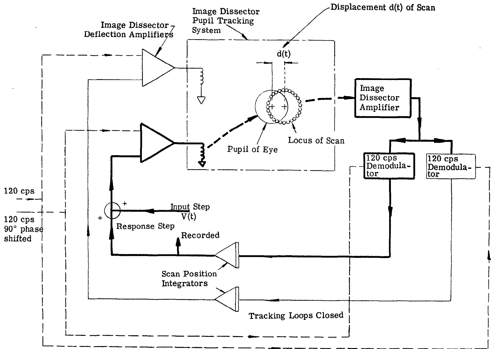
Figure 4.3 SCHEMATIC OF DYNAMIC TEST OF OCULOMETER TRACKING LOOP
