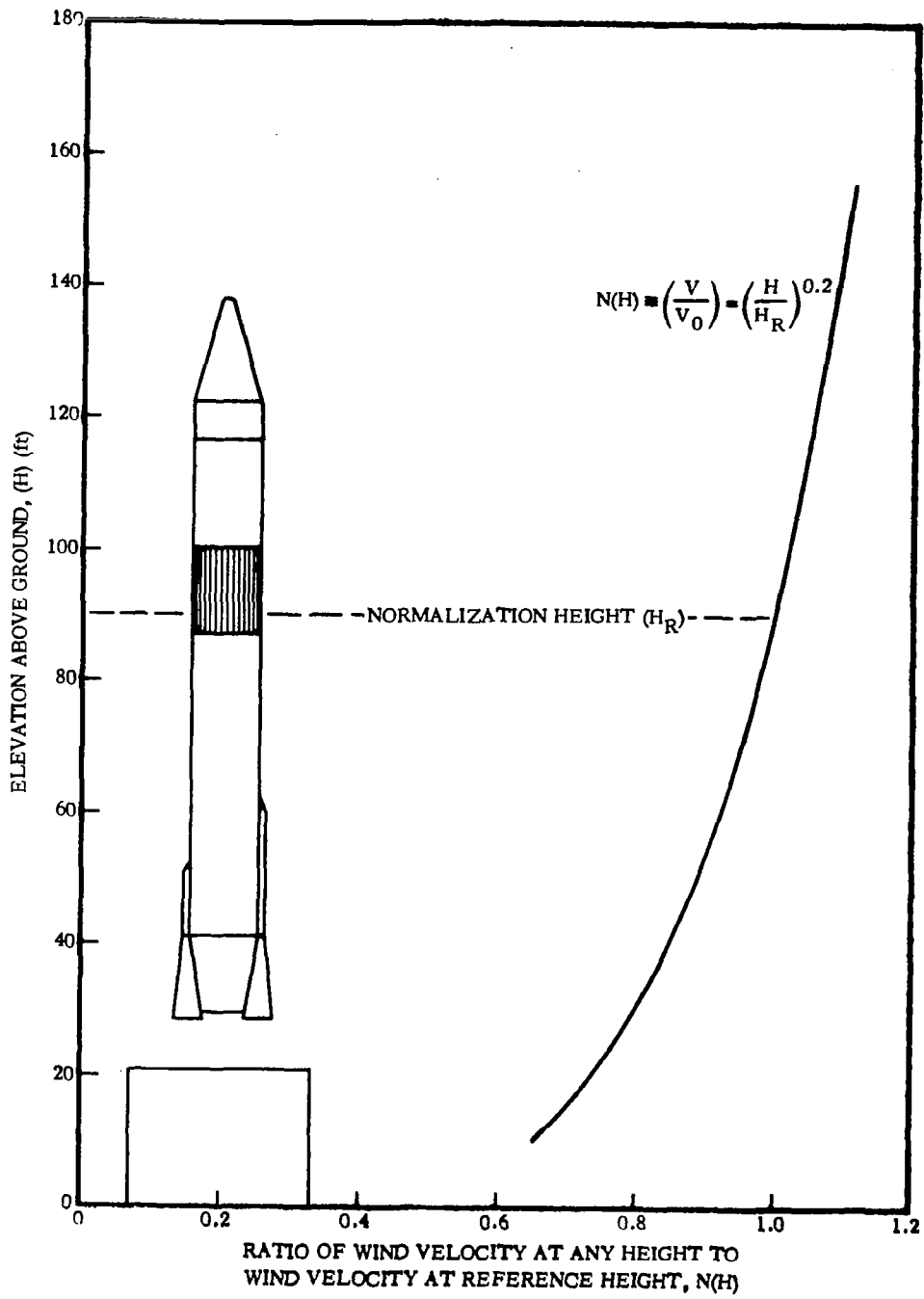
Figure 2. Simple Power-Law Wind Profile
