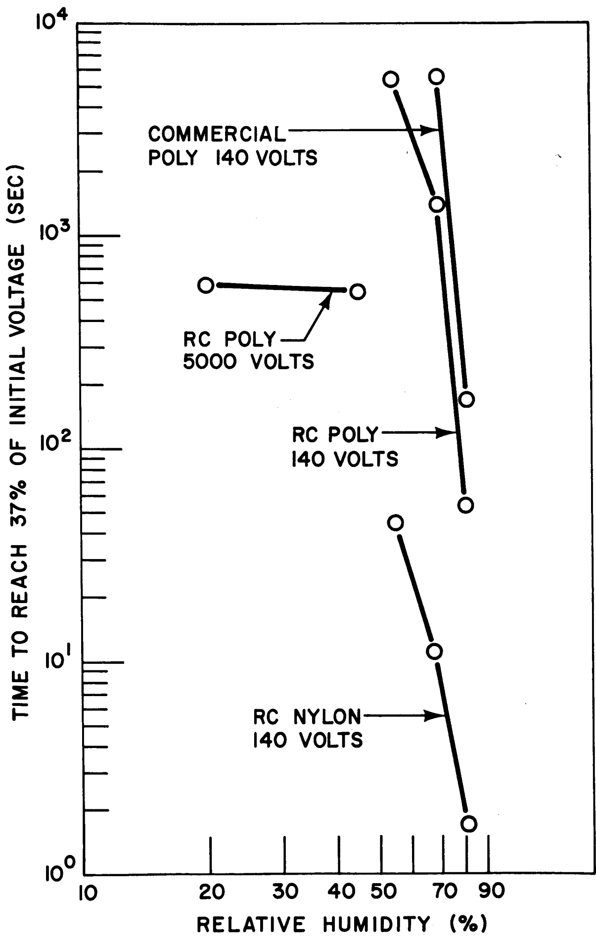
Fig. D-2 - Bulk Properties of Anti-Static Plastic Materials
