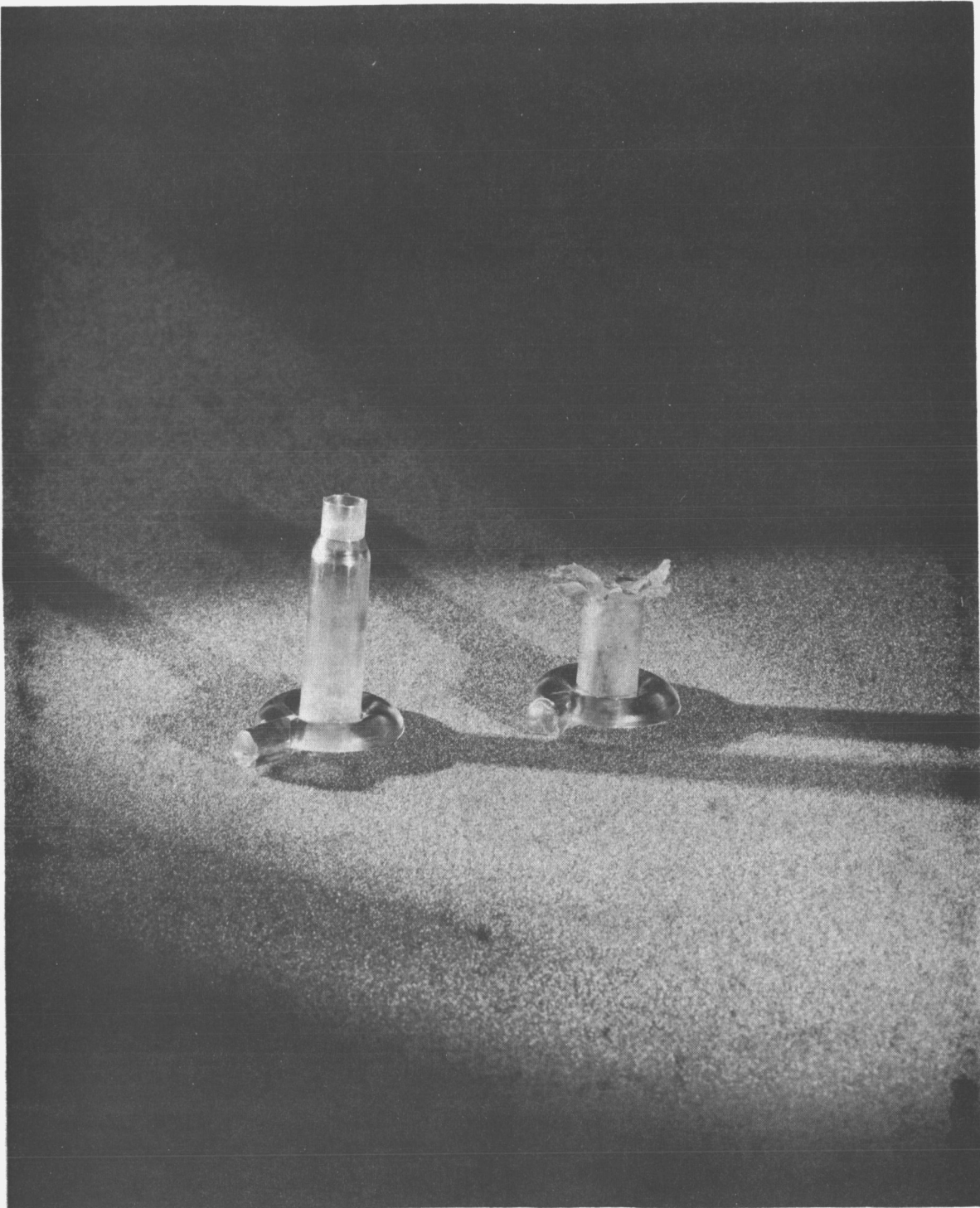
Fig. 14 - Effects of T24E1 Detonator on Polycarbonate Plastics: Various Configurations
