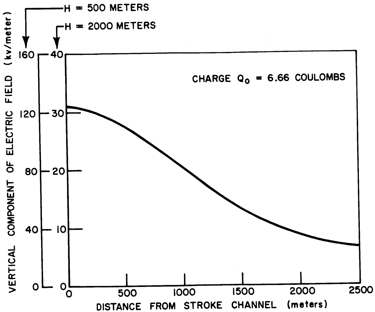
Fig. 7 - Static Electric Field Preceding a Thunderstorm
