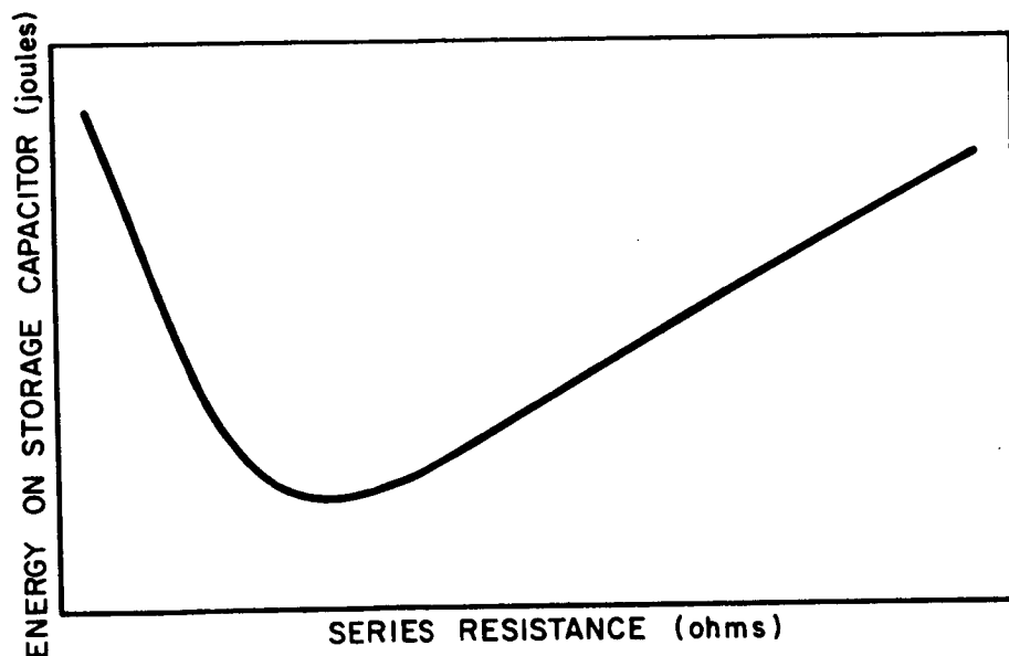
Fig. 6 - Response of Typical Explosive Material to Spark Gap with Series Resistance
