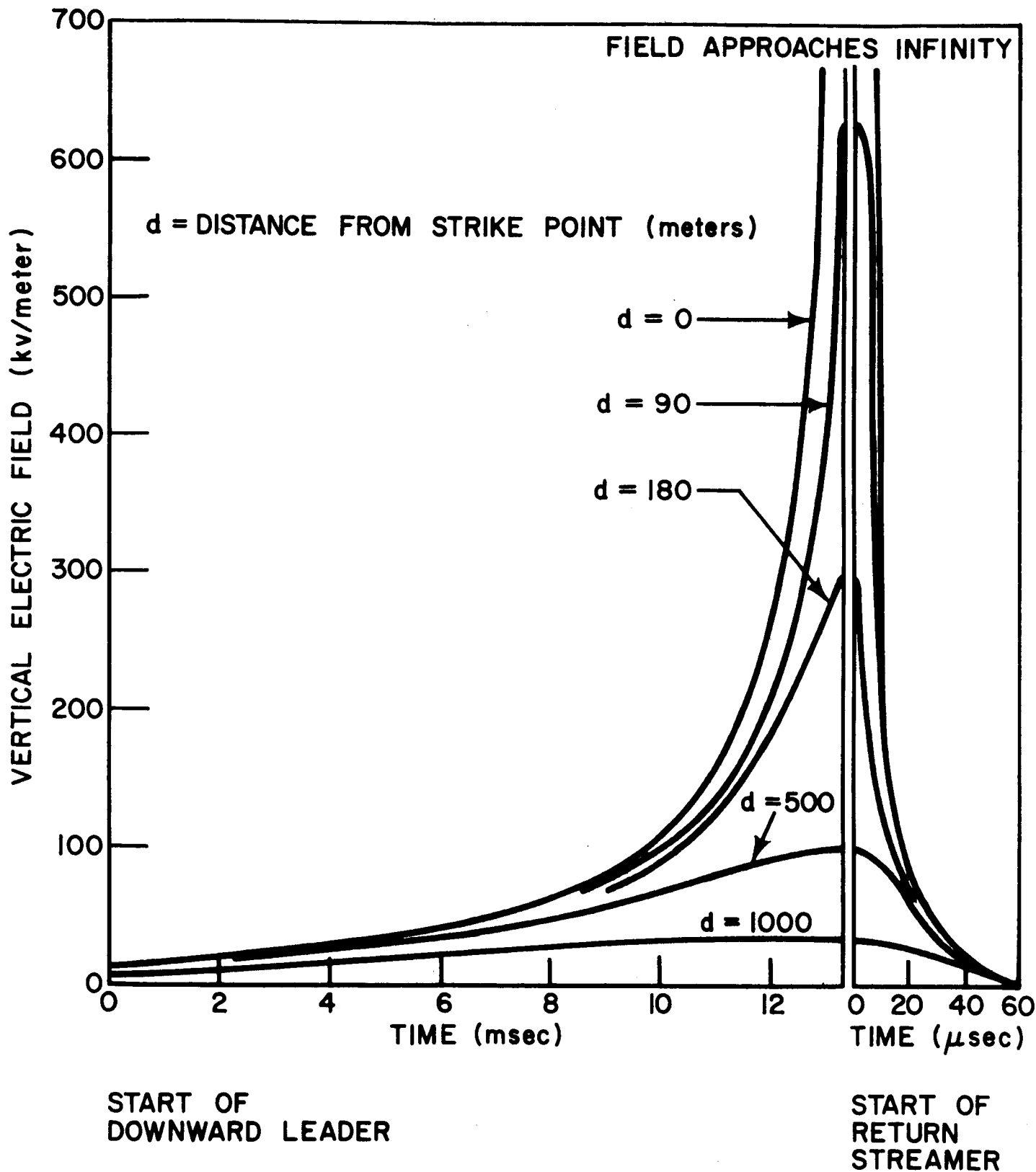
Fig. 8 - Vertical Electric Field During Dynamic Portions of the Lightning Discharge
