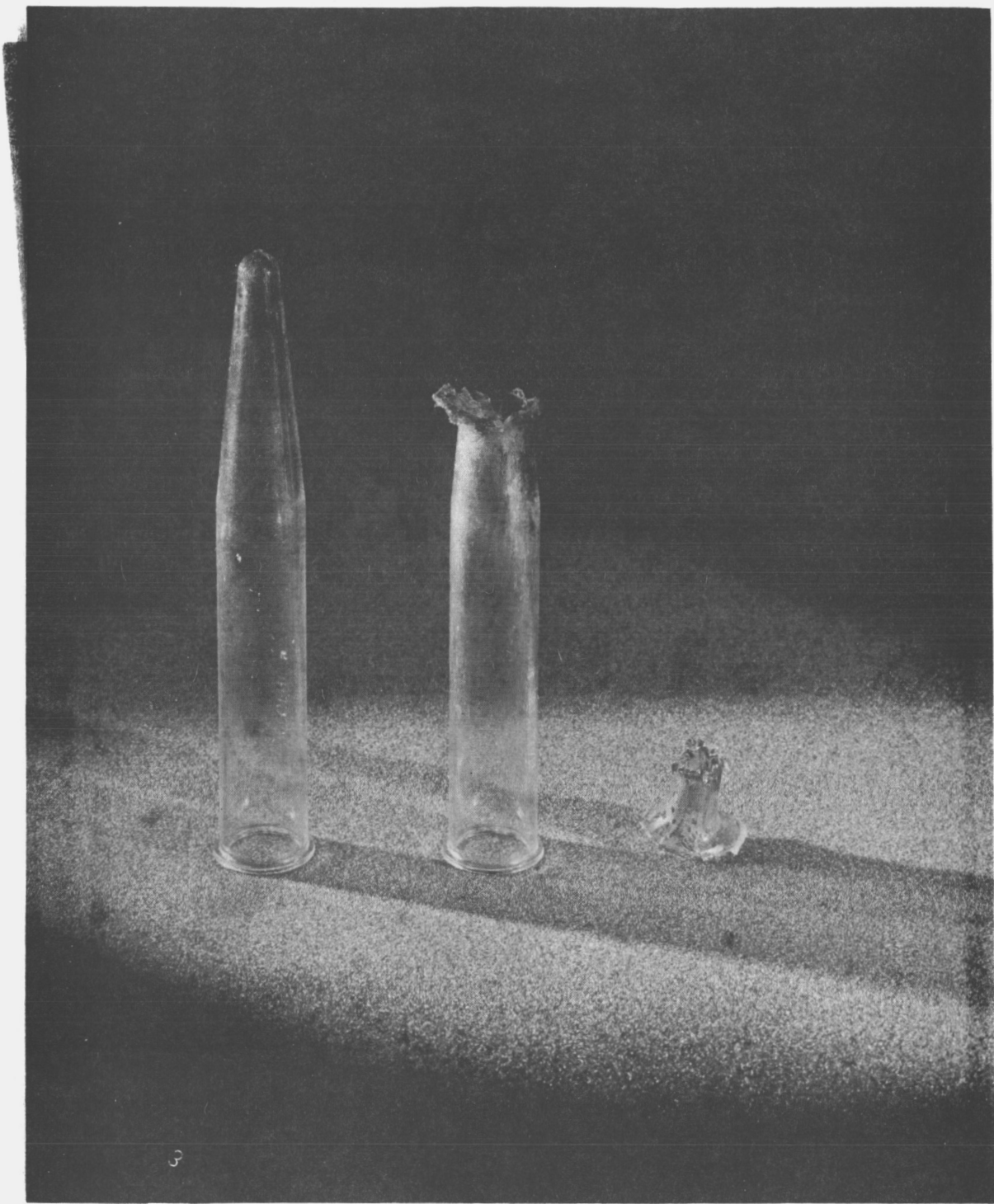
Fig. 16 - Effects of T24E1 Detonator on Polycarbonate Plastics: Various Configurations
