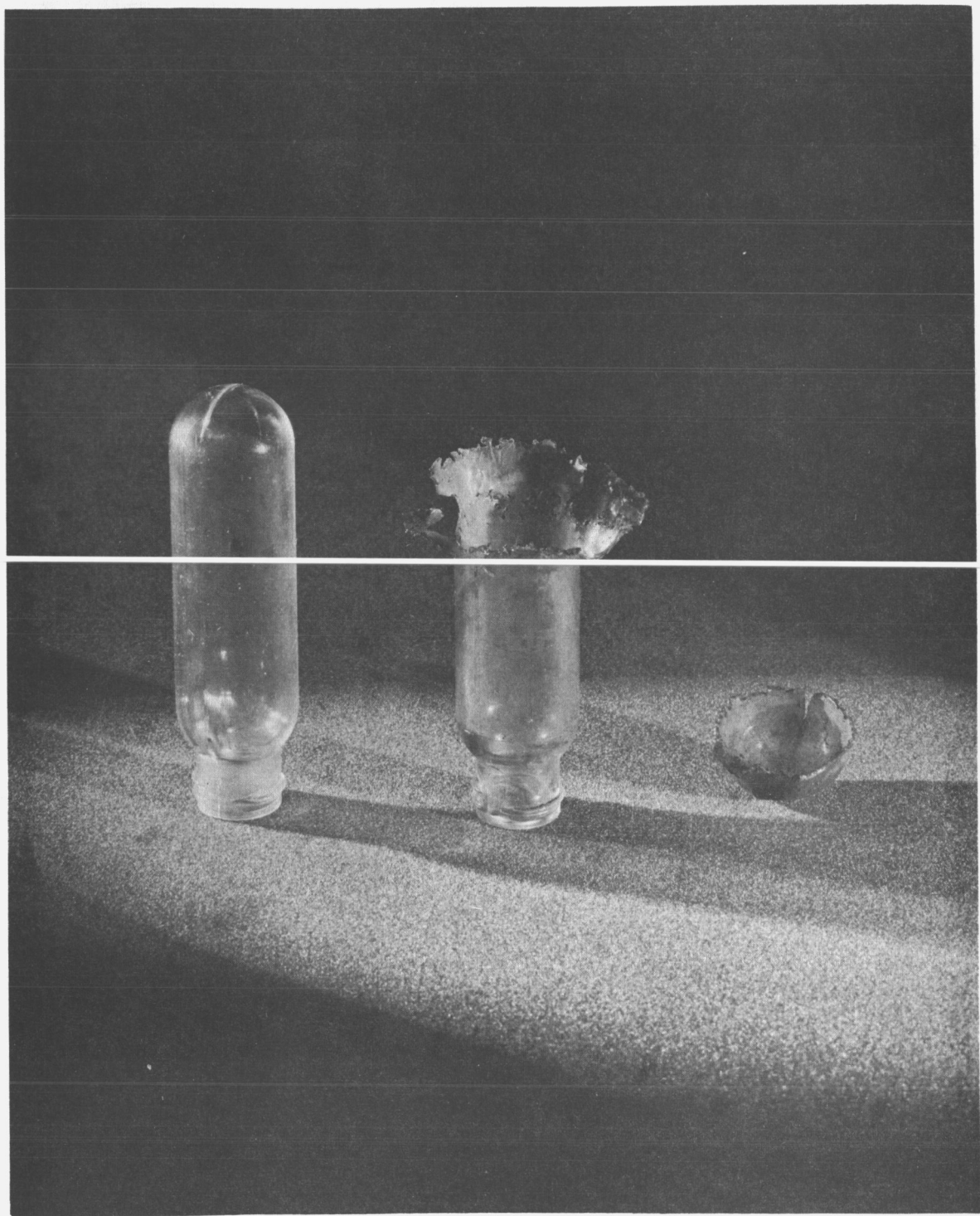
Fig. 15 - Effects of T24E1 Detonator on Polycarbonate Plastics: Various Configurations
