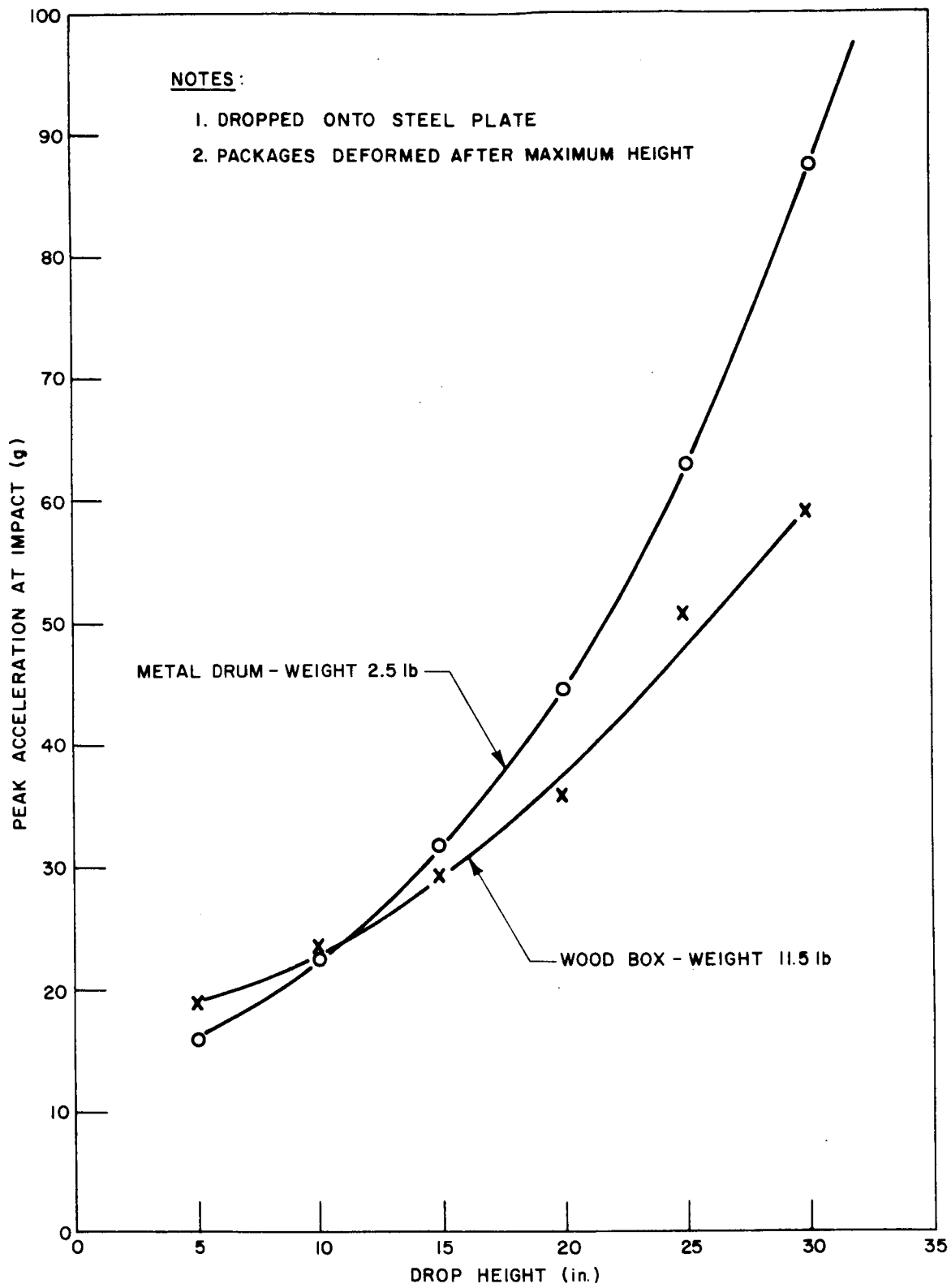
Fig. 11 - Shock Acceleration of Conventional Packages of Electroexplosives at Impact
