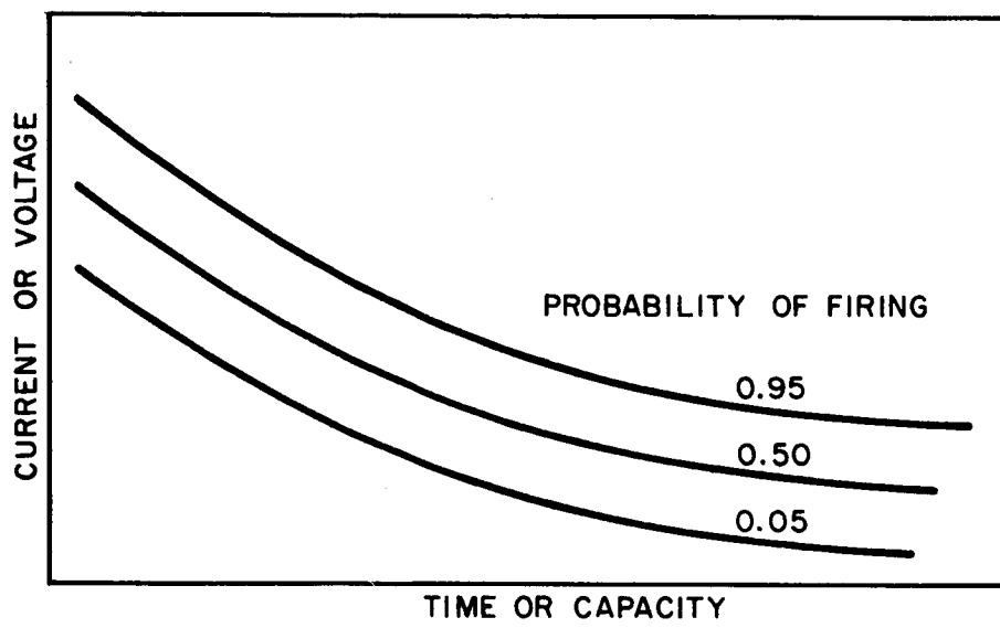
Fig. 3 - Typical Sensitivity Curve of Electroexplosive Devices
