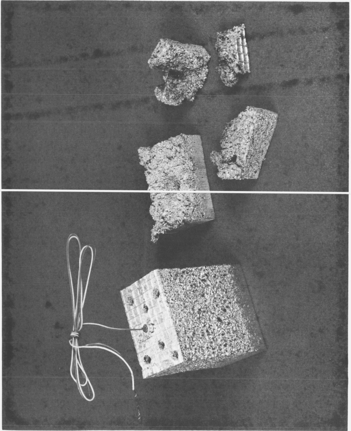
ig. 13 - Foam Aluminum Tested as Dunnage Material - Propagation Stop
