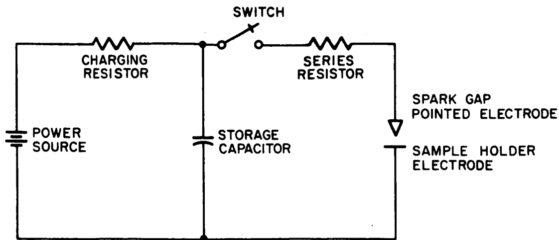
Fig. 5 - Frequently Used Circuit to Determine the Minimum Energy for Explosive Ignition
