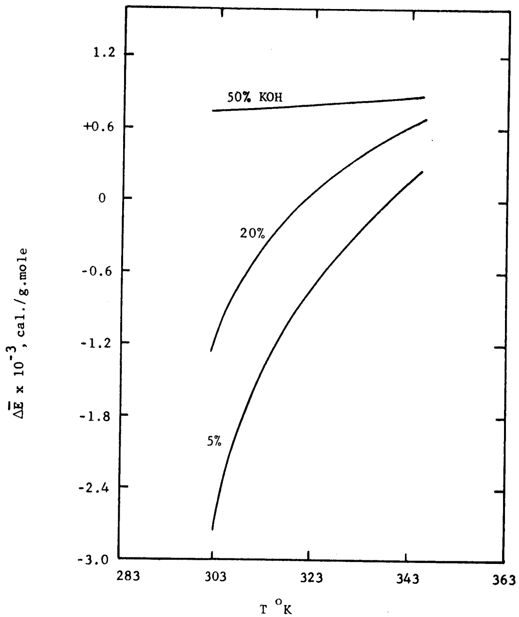
Figure 2.13 ENERGIES OF SOLUTION FOR \text{O}_2 -AQUEOUS KOH SYSTEM
