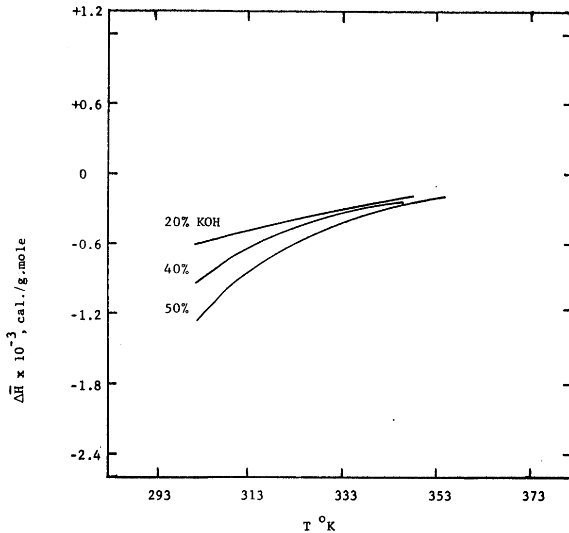
Figure 2.8 HEATS OF SOLUTION FOR H 2 -AQUEOUS KOH SYSTEM
