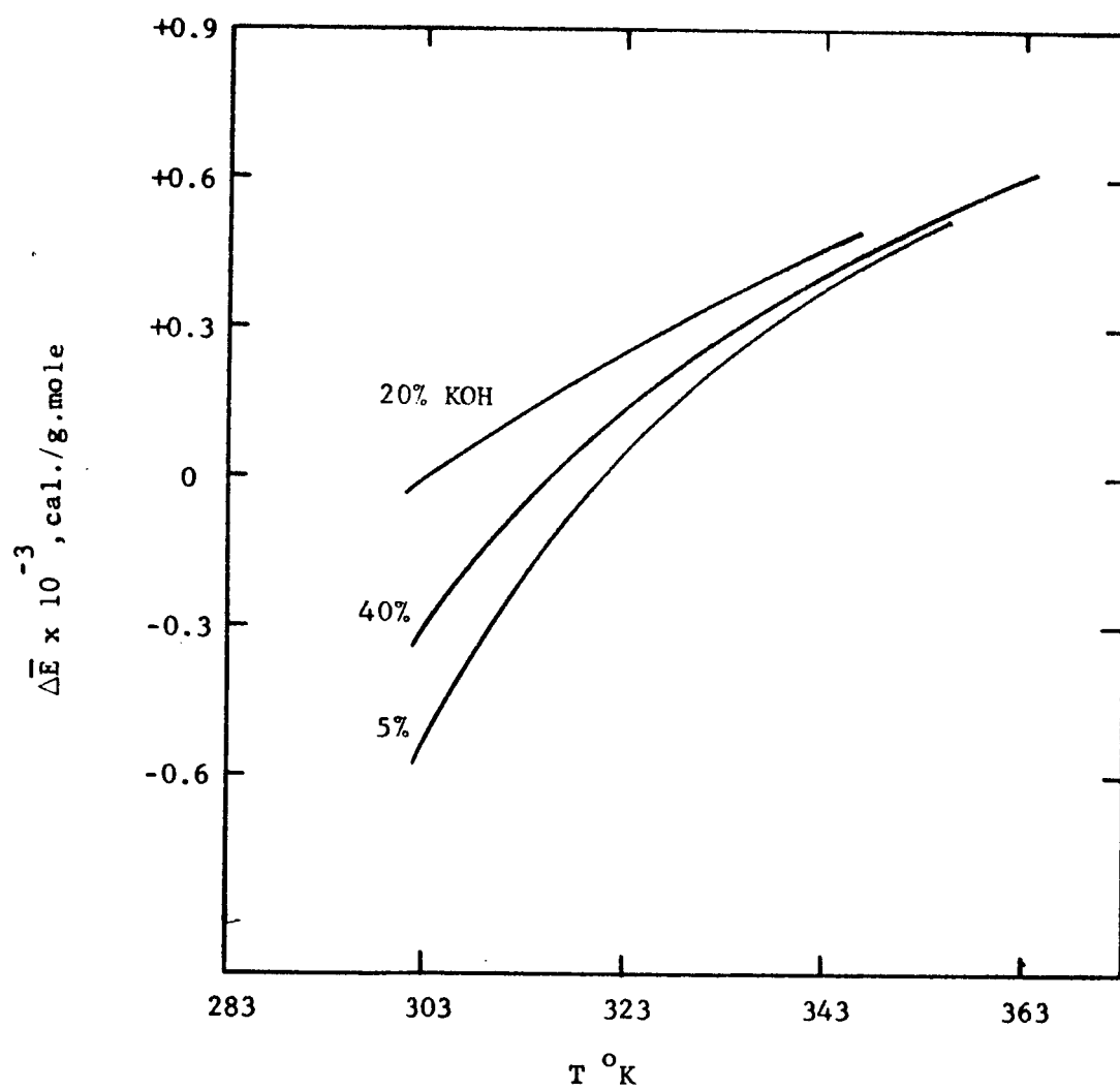
Figure 2.14 ENERGIES OF SOLUTION FOR \text{H}_2 -AQUEOUS KOH SYSTEM
