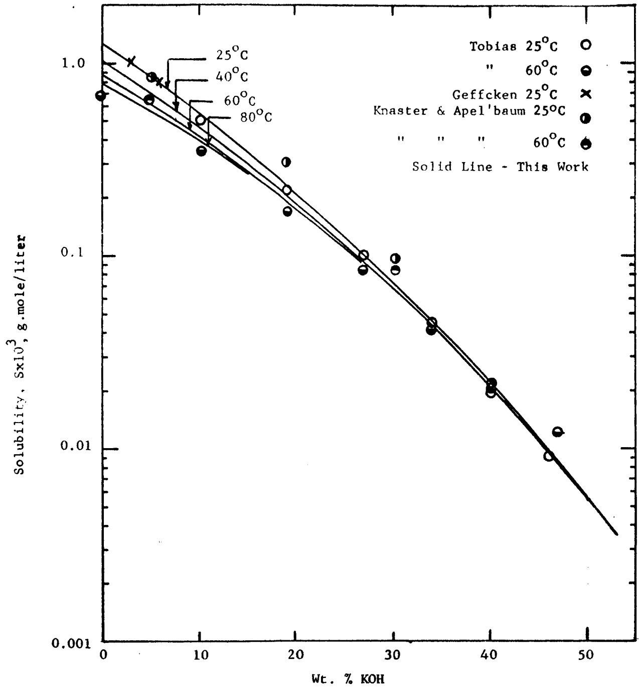
Figure 2.1 SOLUBILITY OF OXYGEN IN AQUEOUS POTASSIUM HYDROXIDE SOLUTIONS
