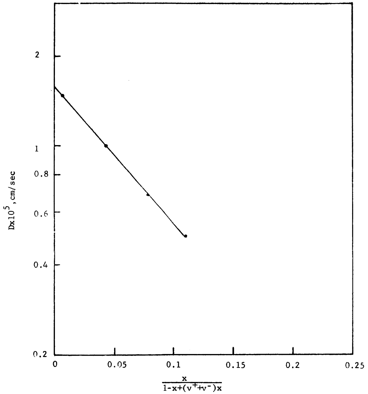
Figure 3.3 Relationship of Diffusivity of Oxygen to Species Fraction of Potassium Hydroxide
