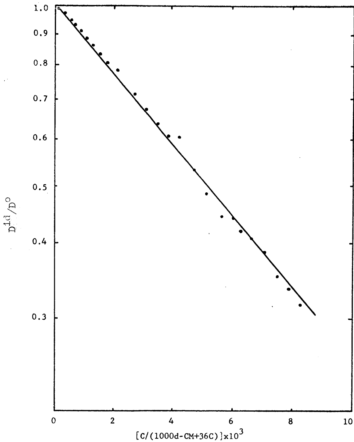
Figure 4.3 Relative diffusion coefficients D^{1d}/D^0 for Aqueous KOH solutions at 25°C
