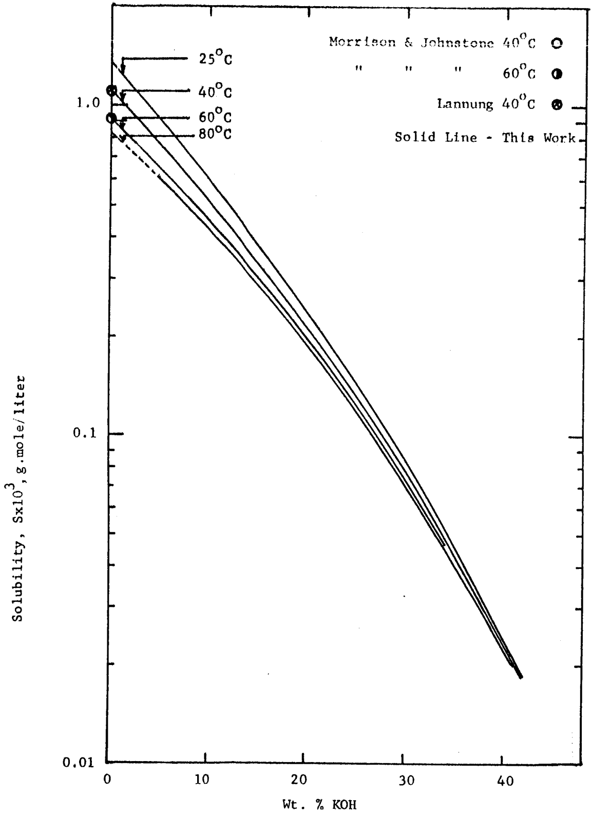
Figure 2.3 SOLUBILITY OF ARGON IN AQUEOUS POTASSIUM HYDROXIDE SOLUTIONS
