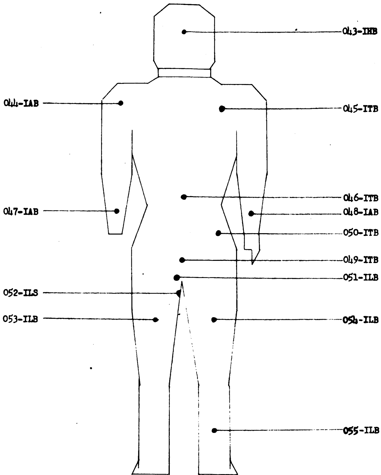
FIGURE 64 THERMOCOUPLE LOCATIONS ON INSIDE, BACK OF SUIT COMFORT LAYER AND INSIDE, BACK OF HELMET
