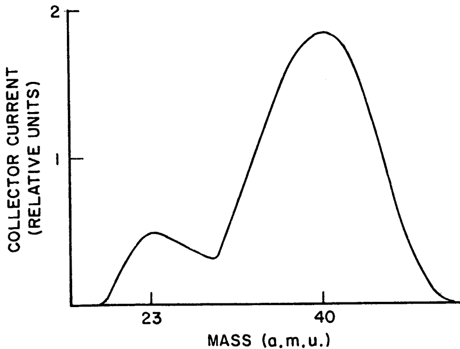
MASS SPECTRUM OF ^{23}\text{Na}^+ , ^{39}\text{K}^+ , ^{41}\text{K}^+ , FROM GATED SPECTROMETER (DIFFERENT SAMPLE FROM THAT USED IN FIGURE 10)
