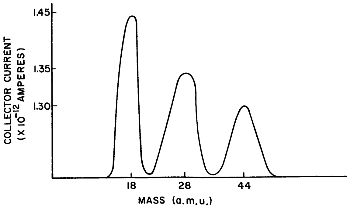
RESIDUAL GAS SPECTRUM FROM GATED SPECTROMETER
