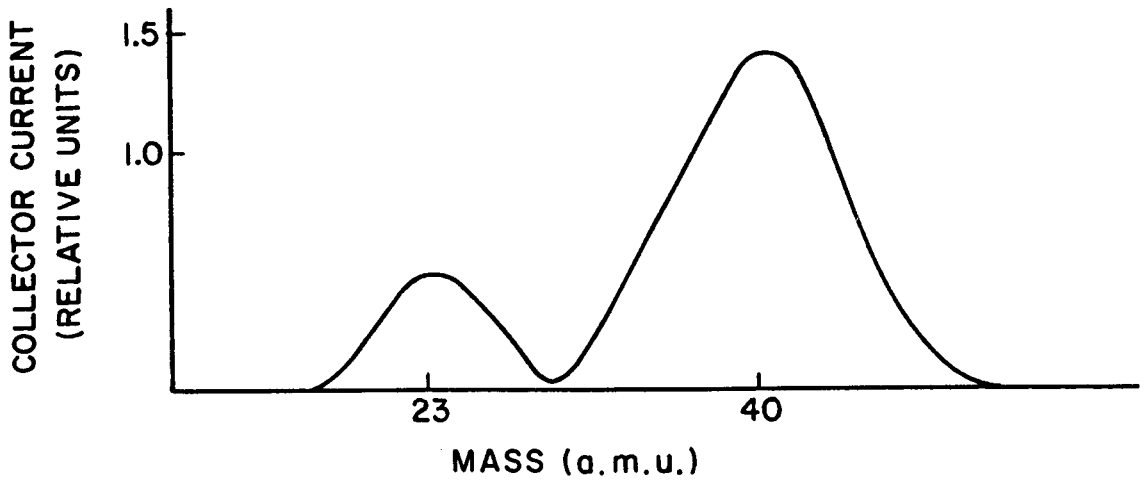
MASS SPECTRUM OF ^{23}\text{Na}^+ , ^{39}\text{K}^+ , ^{41}\text{K}^+ , FROM GATED SPECTROMETER WITH FOCUSING PLATES
