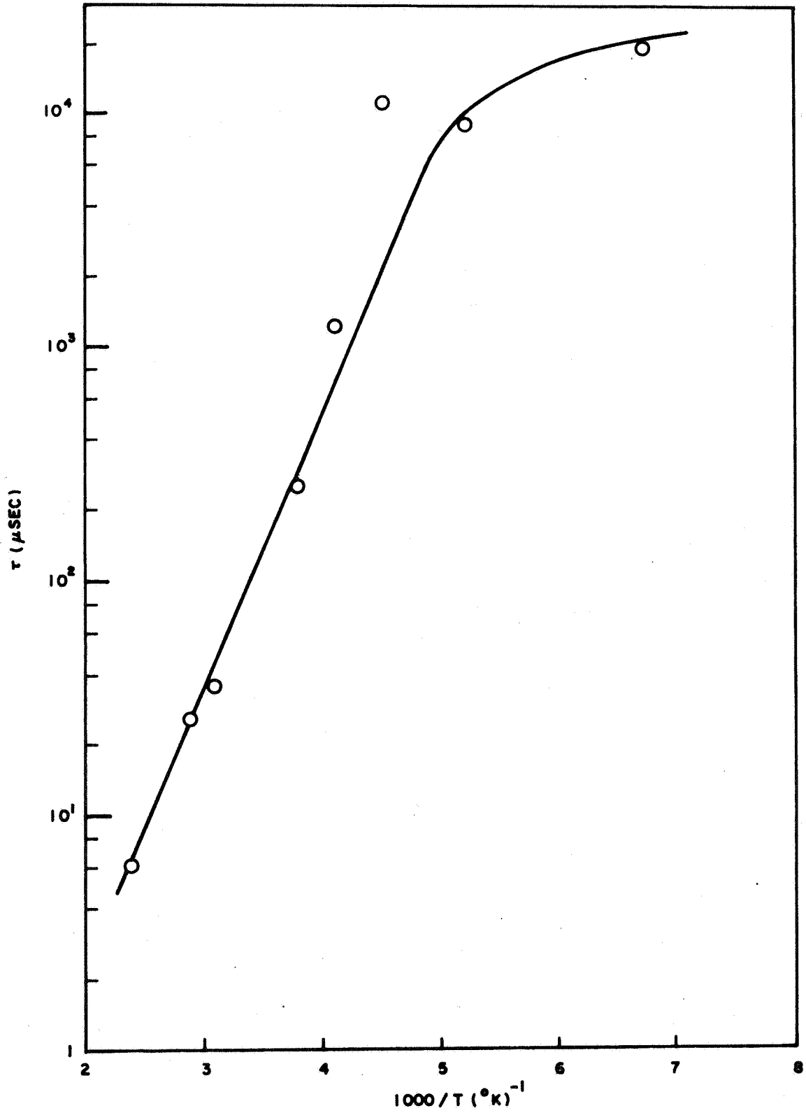
Fig. 16--Inverse temperature dependence of lifetime of high-purity n-type silicon after irradiation at 4.2^{\circ} K and anneal to 340^{\circ} K
