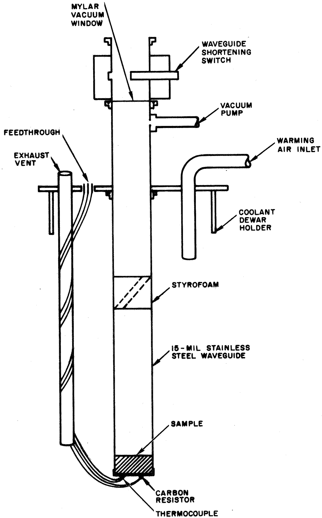
Fig. 2--Sample-holder configuration
