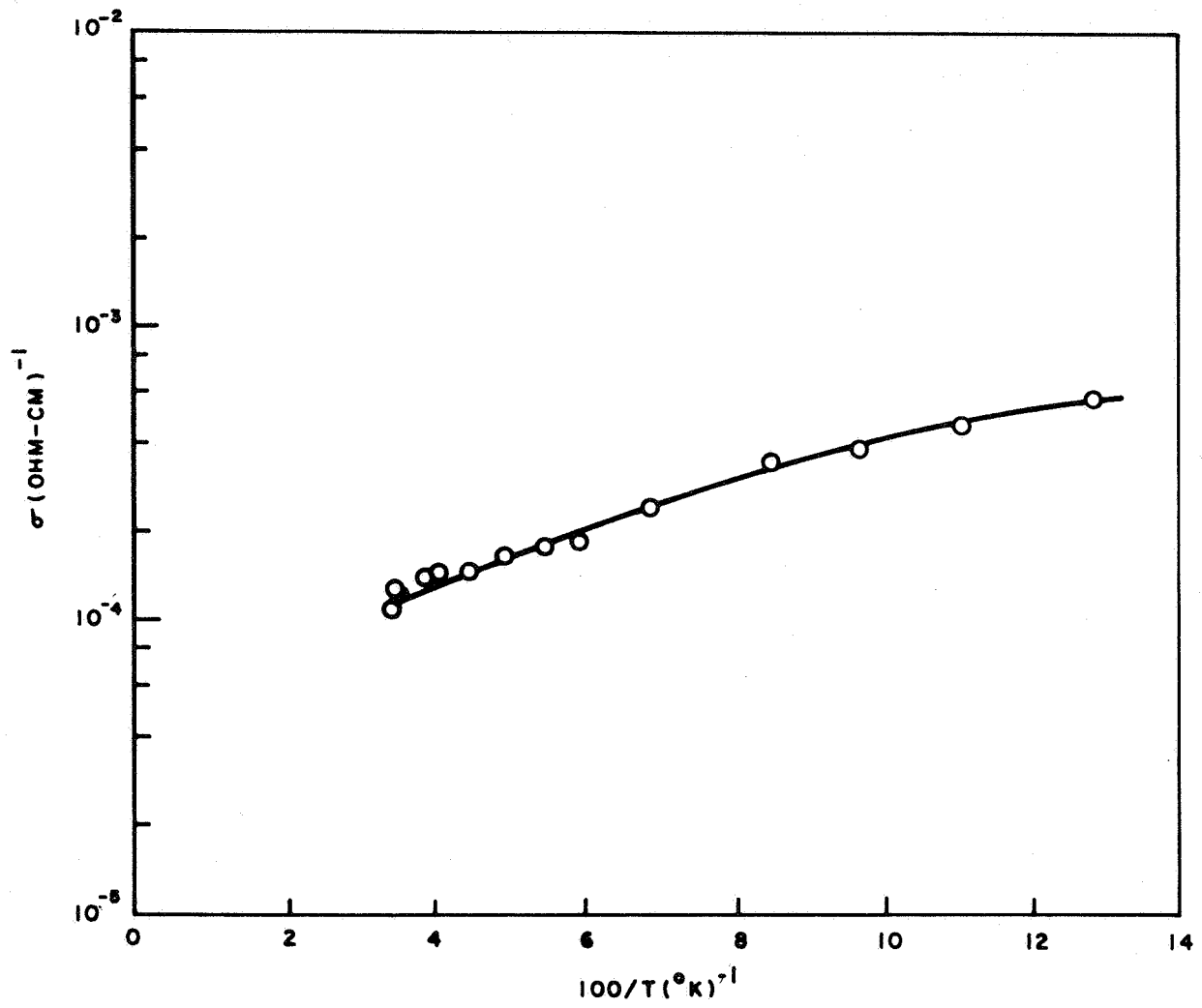
Fig. 5--Preirradiation electrical conductivity as a function of inverse temperature
