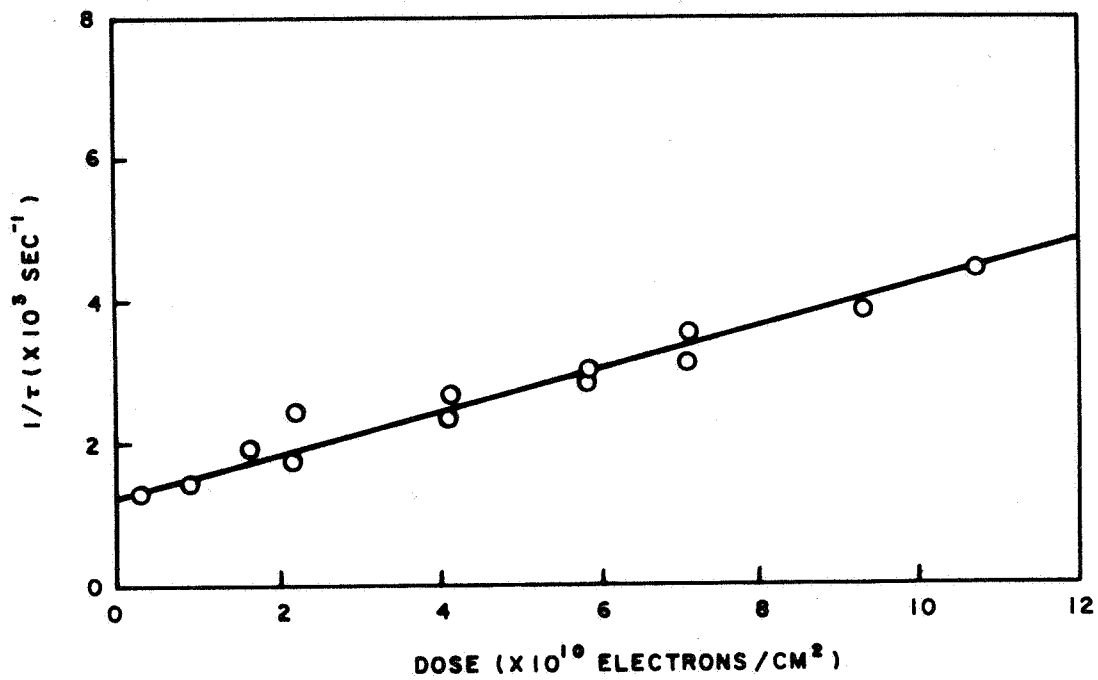
Fig. 19--Degradation of excess-carrier lifetime for p-type silicon after 30-MeV electron irradiation
