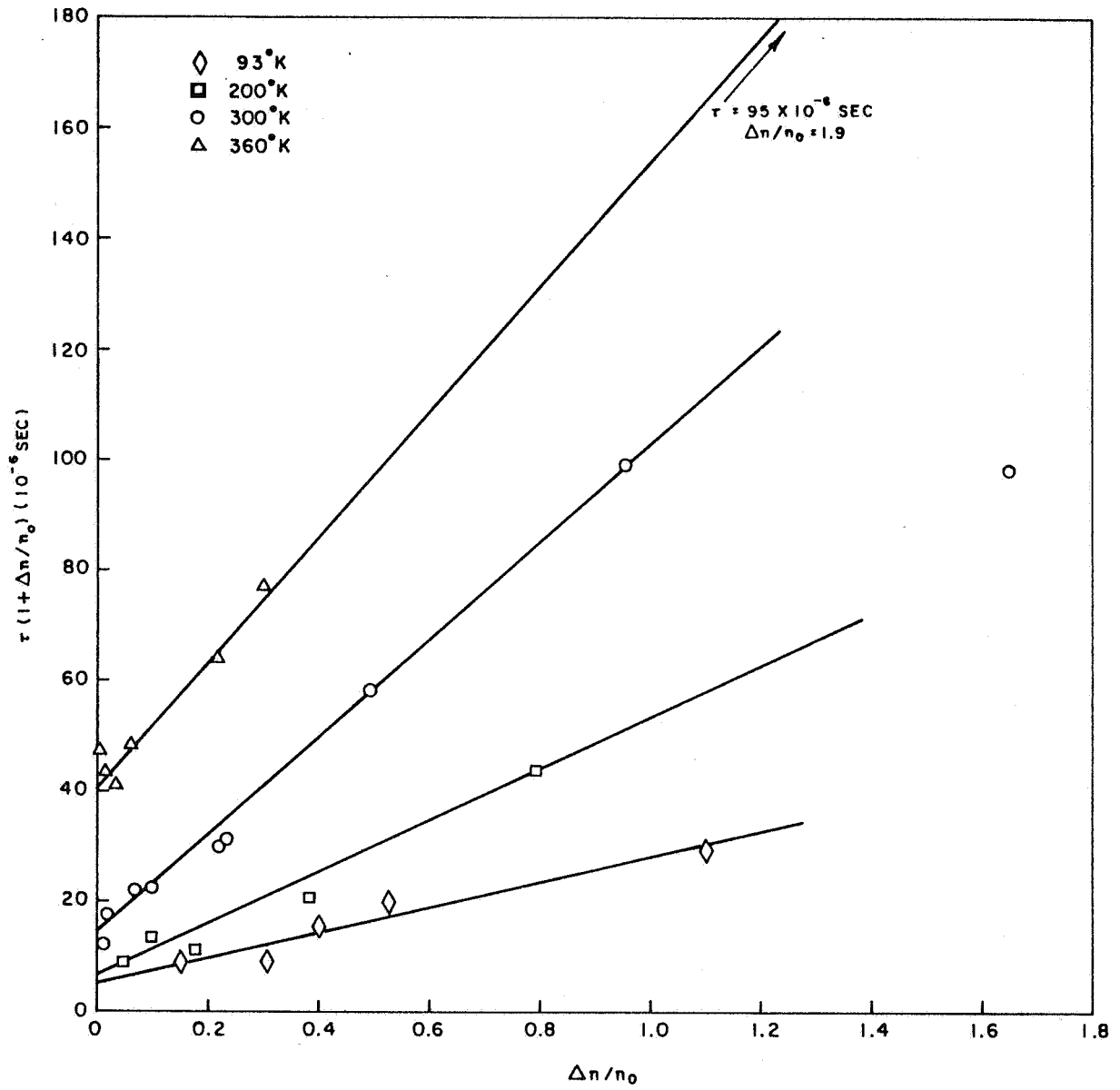
Fig. 29--Dependence of lifetime on excess carrier concentration for 50-ohm-cm, P-doped, QC silicon
