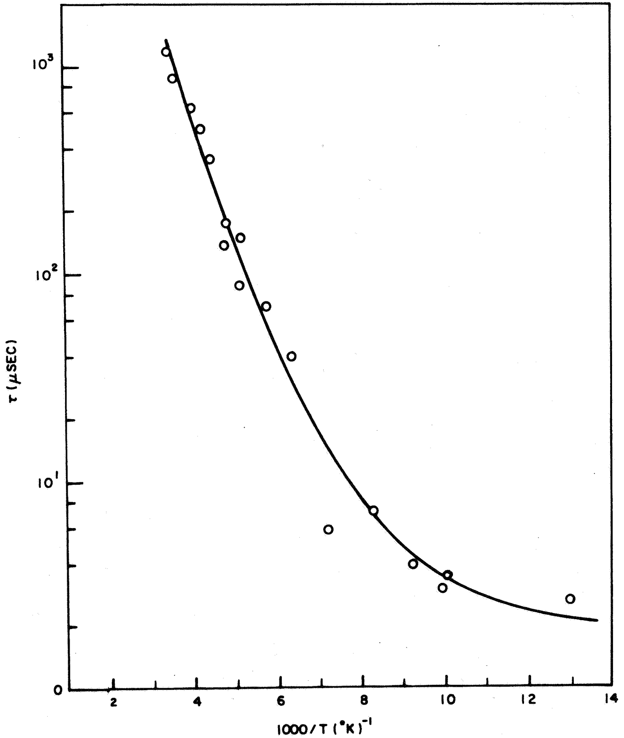
Fig. 17--Preirradiation temperature dependence of excess-carrier lifetime for p-type silicon
