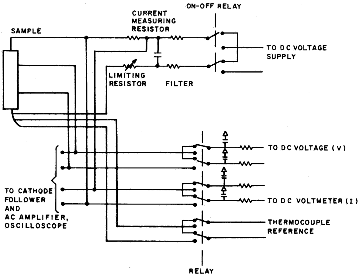
Fig. 26--Lifetime measuring circuit
