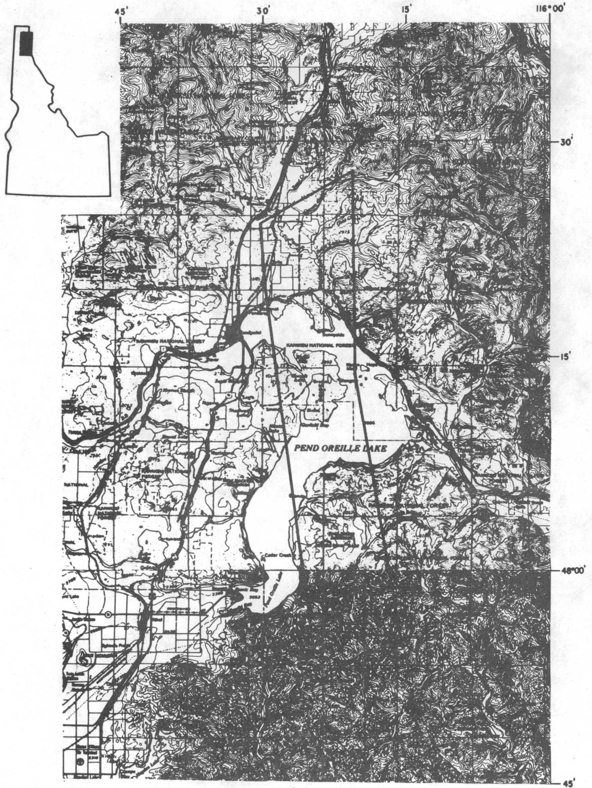
Figure 1. INDEX MAP SHOWING LOCATION OF AREA COVERED BY INFRARED IMAGERY
