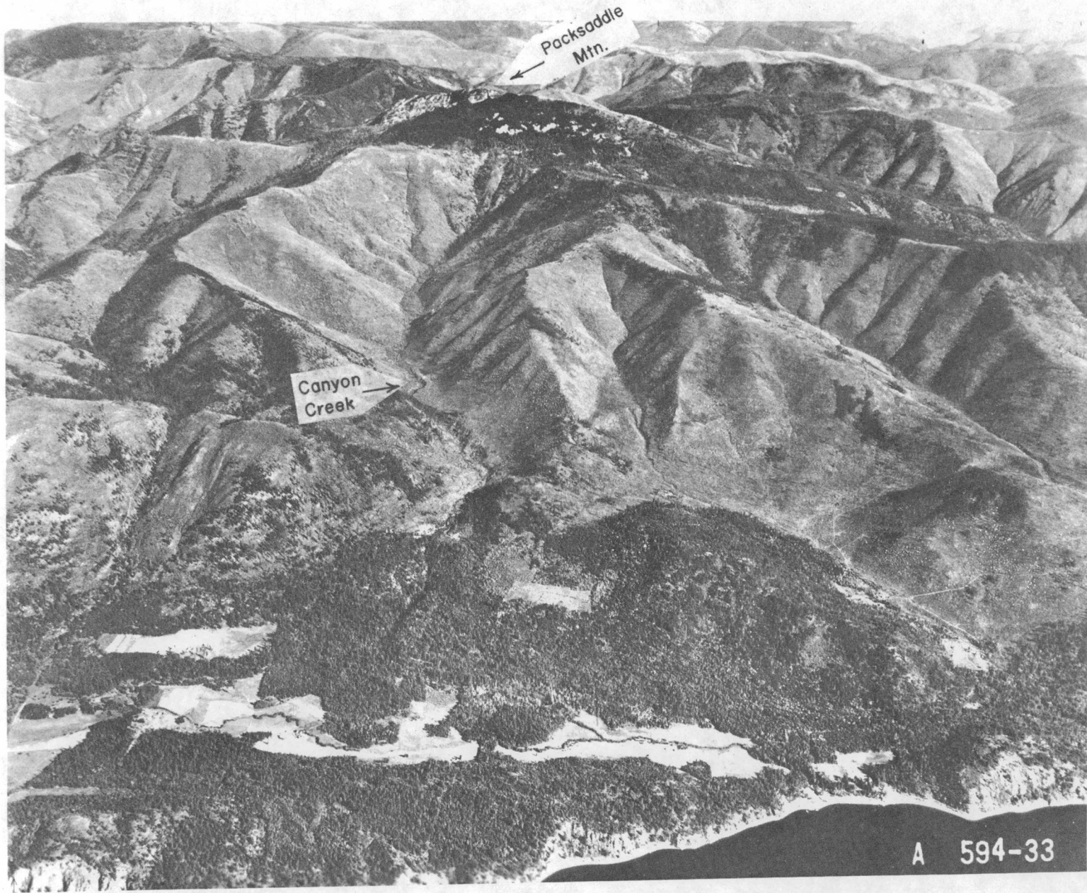
FIGURE 6 BLACK AND WHITE AERIAL OBLIQUE PHOTO OF PACKSADDLE MOUNTAIN (COURTESY OF 11th PHOTO SECTION, WASHINGTON NATIONAL GUARD)
