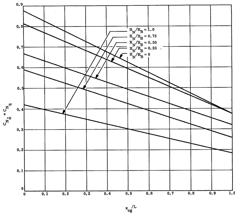
Figure 4-8. Normal Force Coefficient, C_{N\dot{\alpha}} + C_{Nq} , as a Function of R_N/R_B and x_{cg} for Real Gas Case
