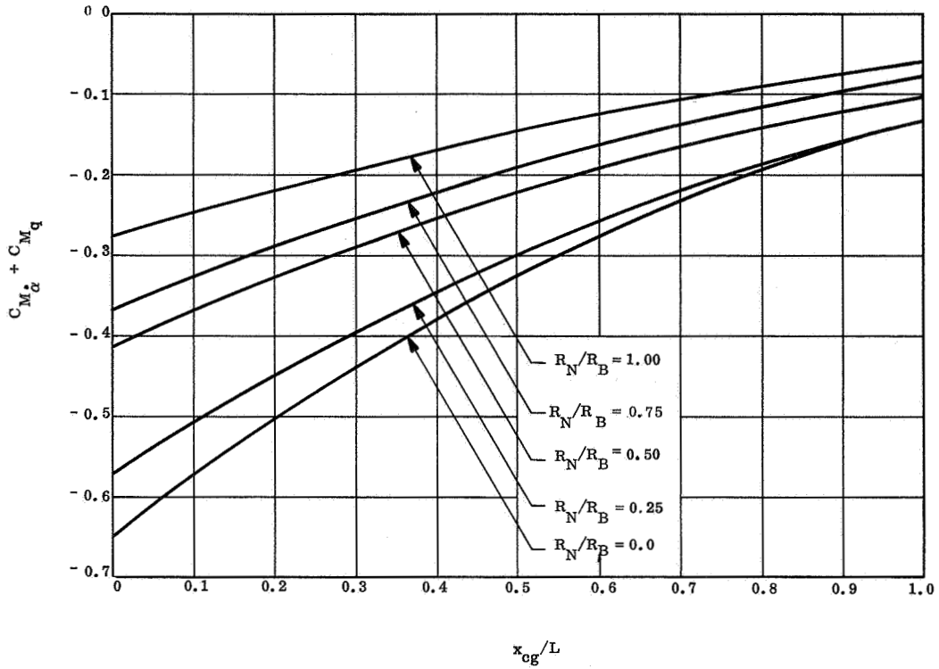
Figure 4-1. Dynamic Stability Coefficient, C_{M_q} + C_{M_{\dot{q}}} , as a Function of R_N/R_B and x_{cg} for Ideal Gas Case
