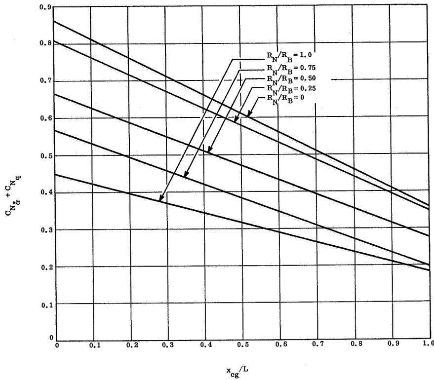
Figure 4-7. Normal Force Coefficient, C_{N\dot{\alpha}} + C_{Nq} , as a Function of R_N/R_B and x_{cg} for Ideal Gas Case
