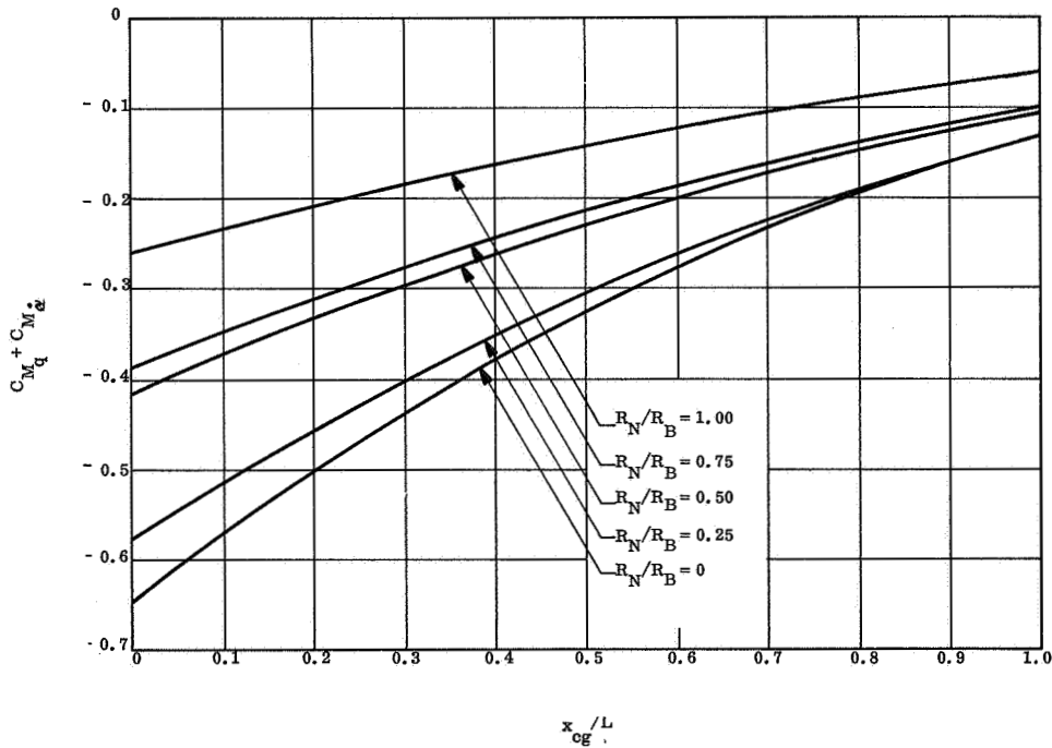
Figure 4-2. Dynamic Stability Coefficient, C_{M_q} + C_{M_{\dot{q}}} , as a Function of R_N/R_B and x_{cg} for Real Gas Case
