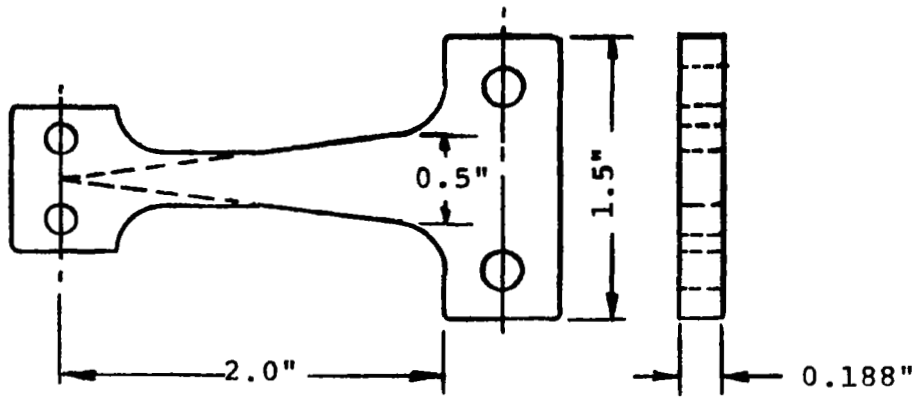
(a) Flexure fatigue specimen for Unit I
