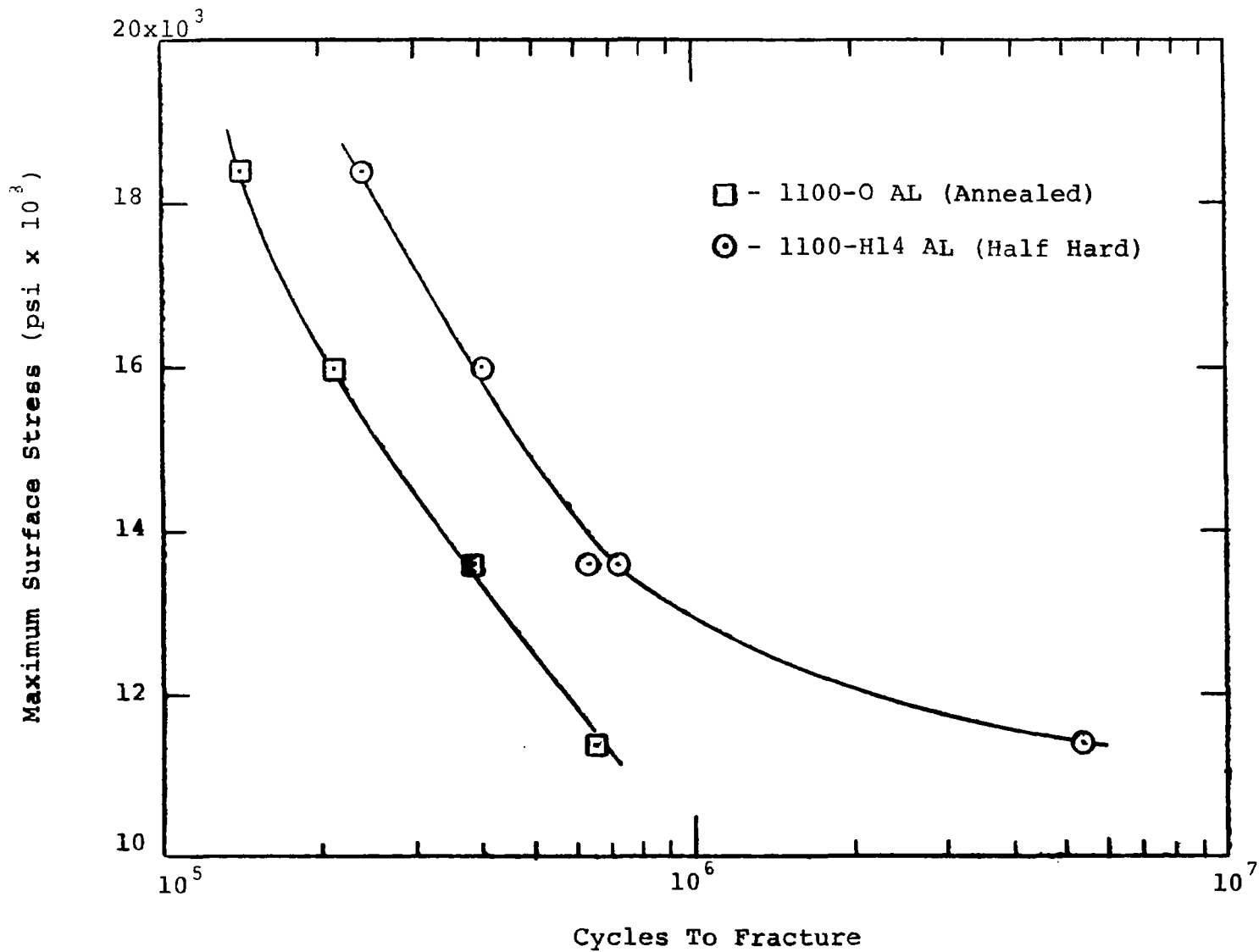
Fig. 17 Effect of prior cold work on the fatigue properties of aluminum
