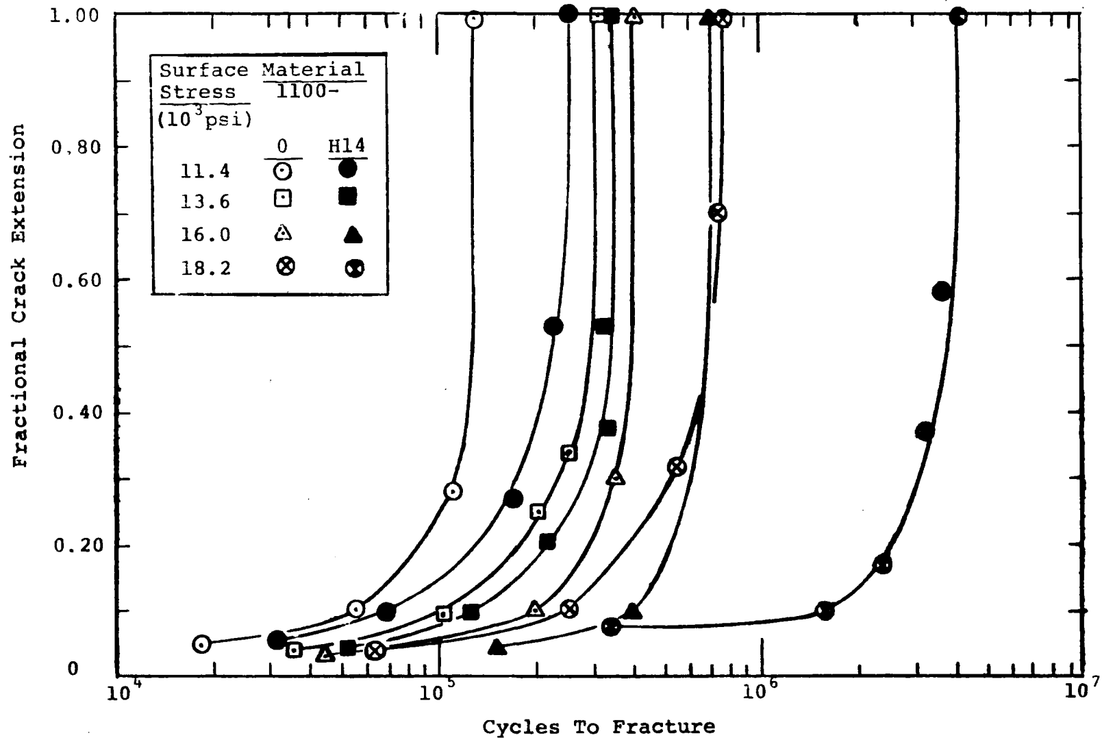
Fig. 19 The dependence of the rate of crack extension on and the number of cycles to fracture on applied stress amplitude.
