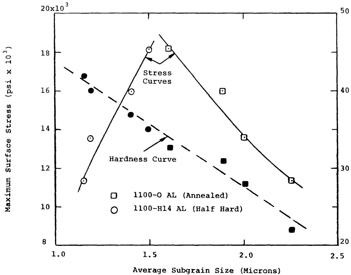
Fig. 18 Dependence of the fatigue subgrain size on applied stress amplitude and hardness level.
