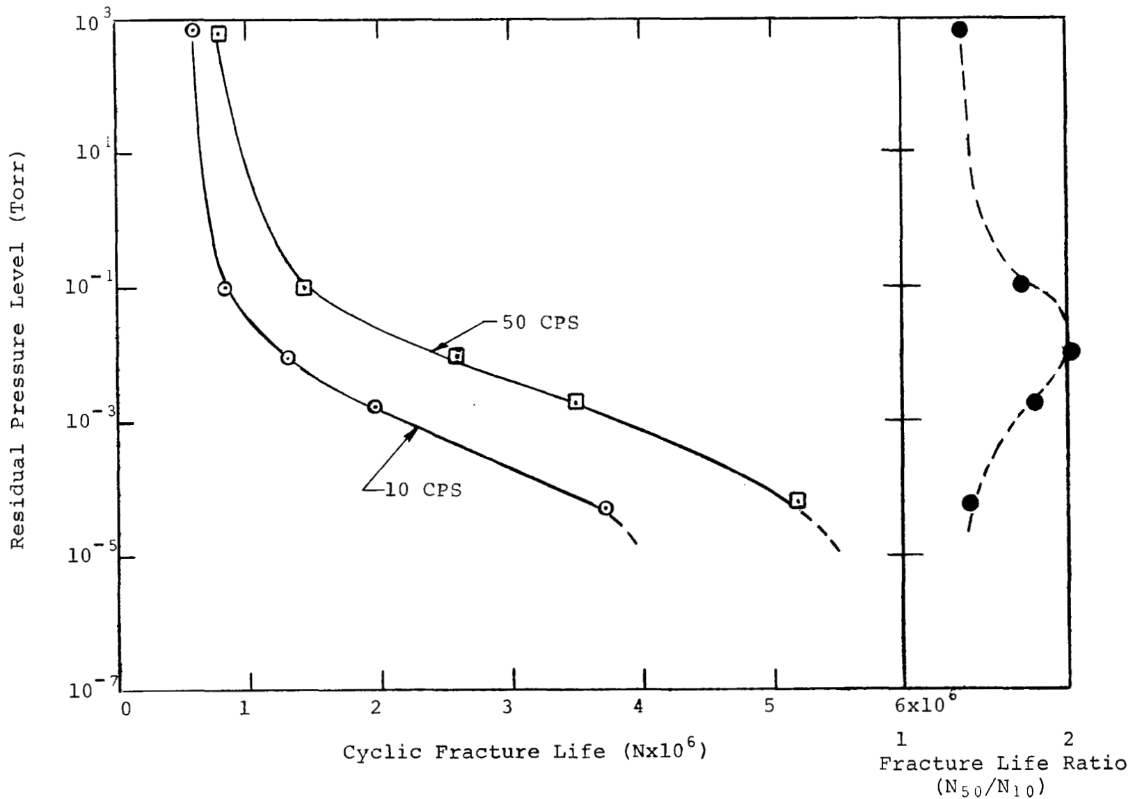
Fig. 7 Cyclic loading rate dependence of fatigue life of 1100 aluminum at reduced pressure in Unit I tests.
