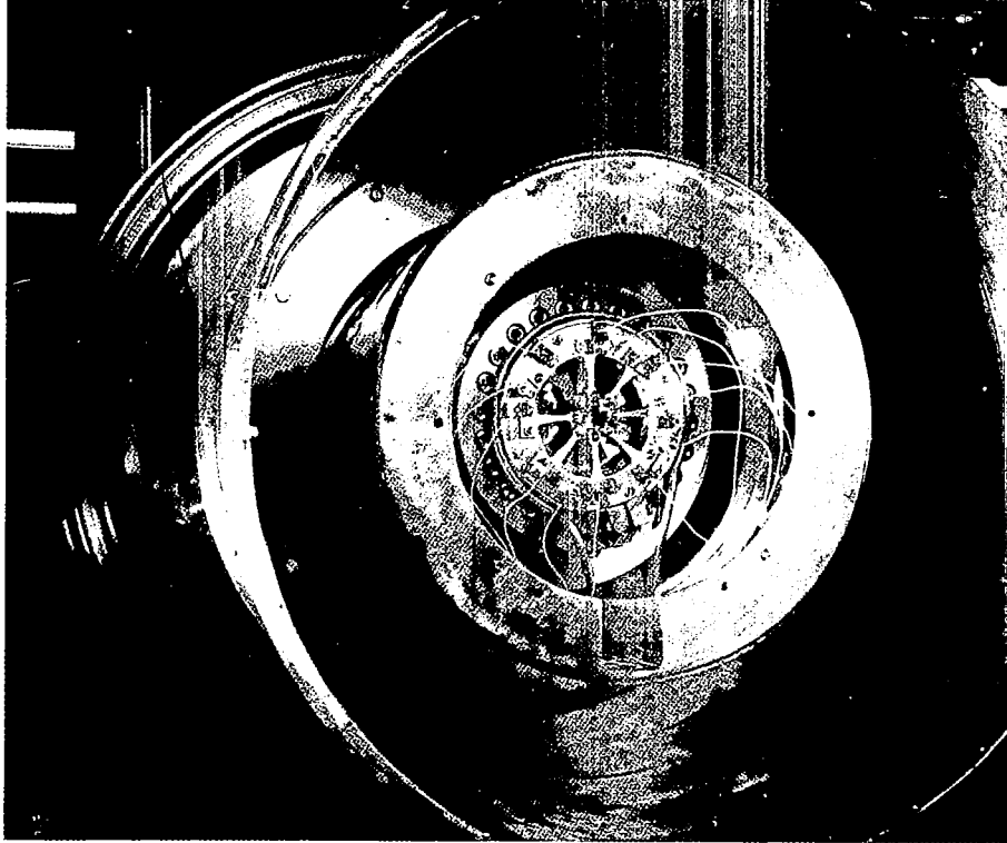
View of Fatigue Apparatus Unit II In XHV System
