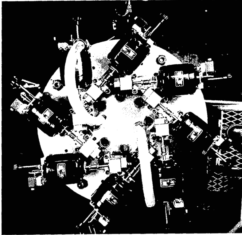
Top View Of Fatigue Unit I Vacuum Flange Showing Motor Drive and Bearing Housing Assemblies.
