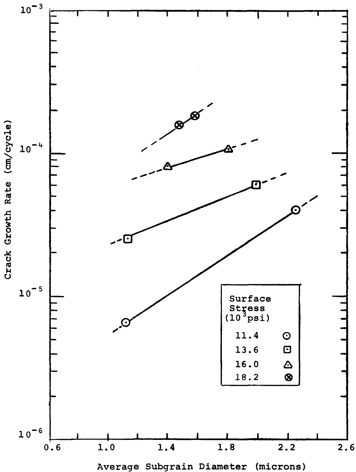
Fig. 20 The effect of the subgrain diameter on the observed crack growth rate.
