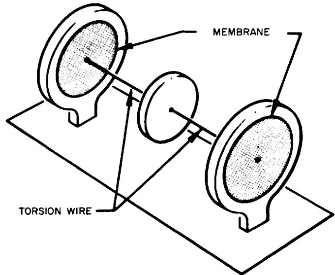
Fig. 9. Combined membrane and torsion-wire suspension
