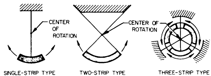
Fig. 3. Flexure suspensions (flat springs that support a rotating part). Three types are shown
