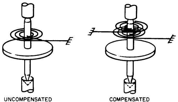
Fig. 7. Spiral spring suspensions with conical bearings
