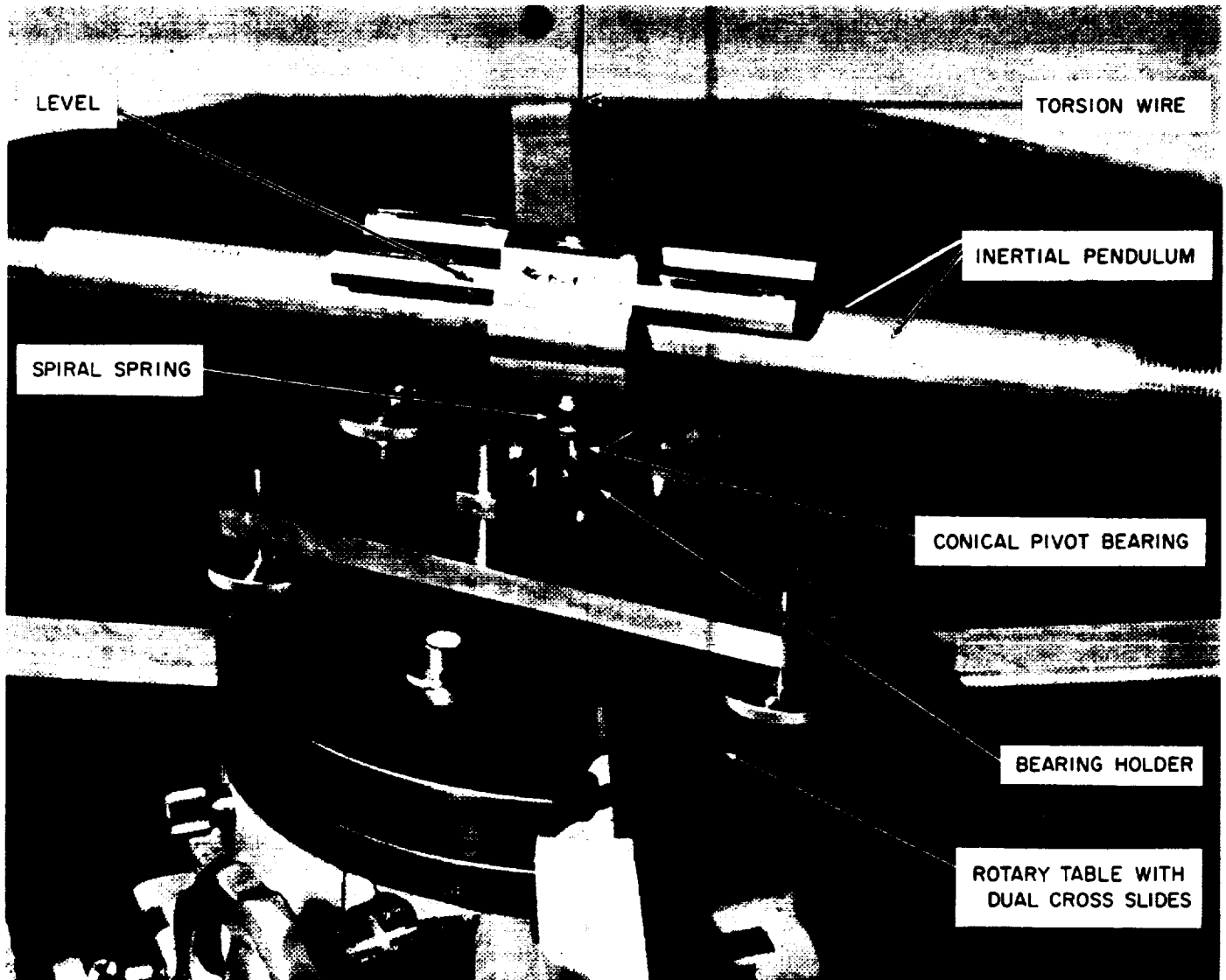
Fig. 10. Torsion wire and spiral-spring suspensions in an orbital simulator designed by the author (photograph courtesy of Philco-Ford Western Development Laboratories)
