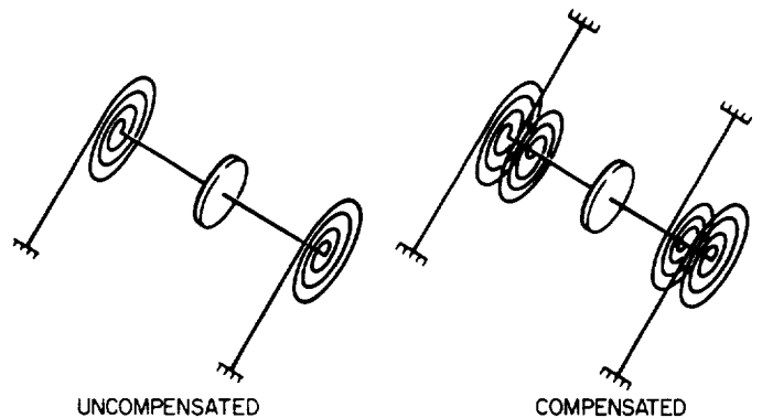
Fig. 6. Spiral spring suspensions
