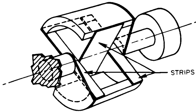
Fig. 4. Two-strip flexure suspension with one strip in one axis and two in the other axis
