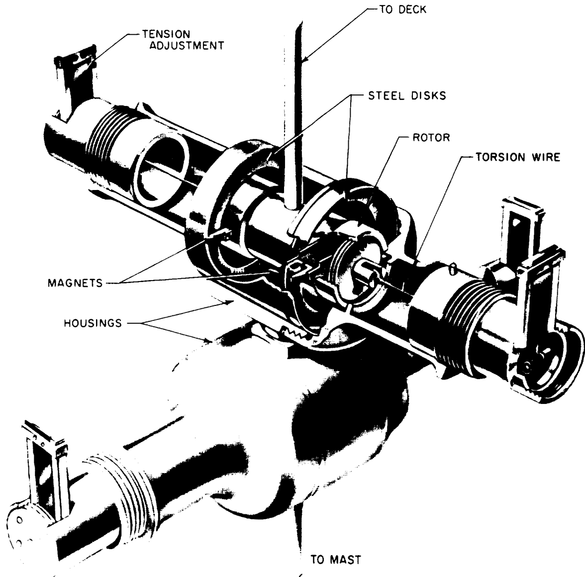
Fig. 1. Torsion-wire suspension used in magnetic hysteresis damper. Each unit contains a double suspension and each is free to rotate 60 deg in either direction from the null position (photograph courtesy of American Telephone and Telegraph Co.)
