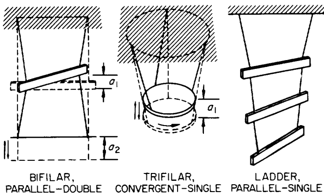
Fig. 2. Typical filar suspension configurations
