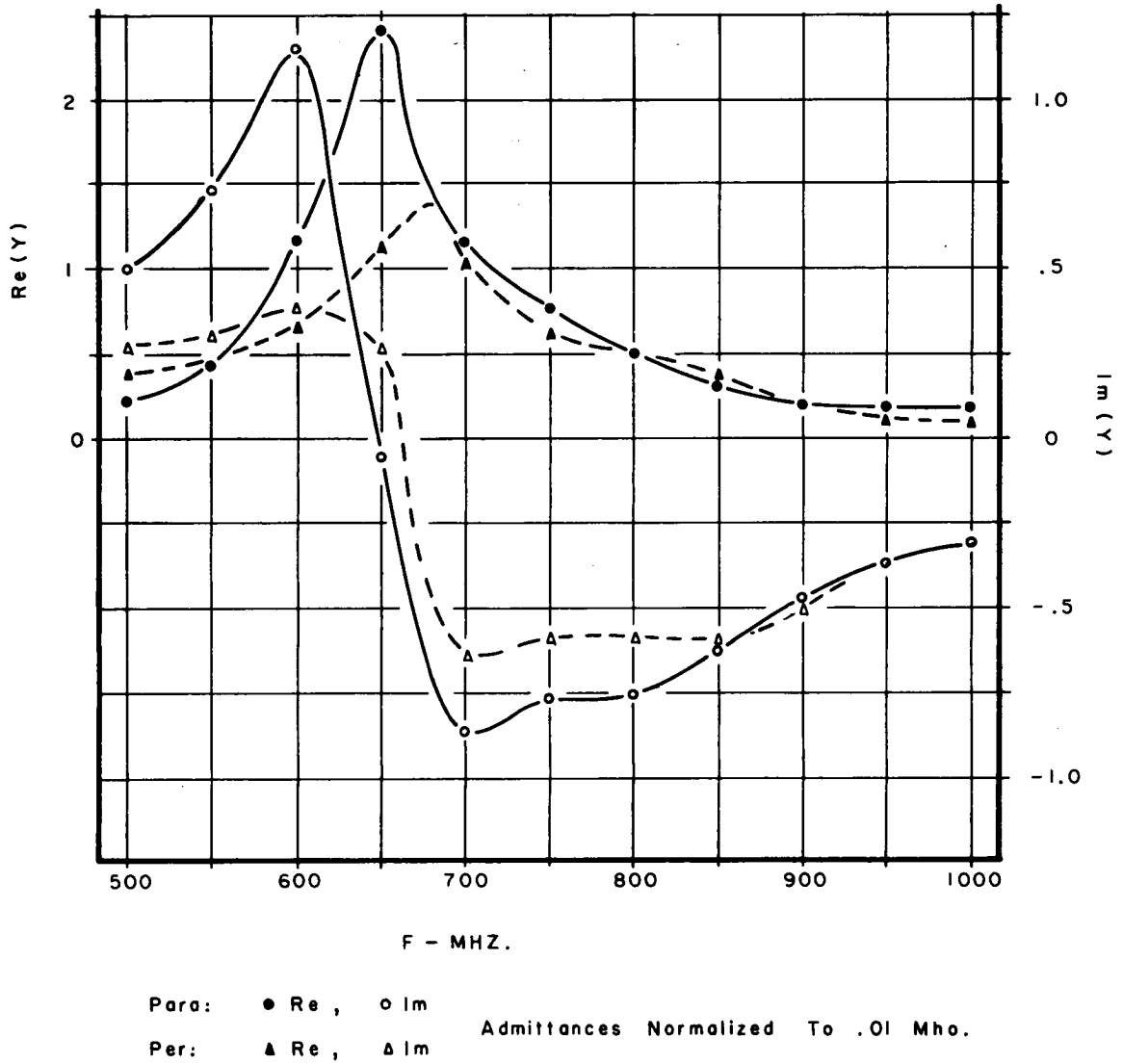
FIGURE II. MEASURED ADMITTANCES FOR THE TWO CASES. B = 256 GAUSS.
