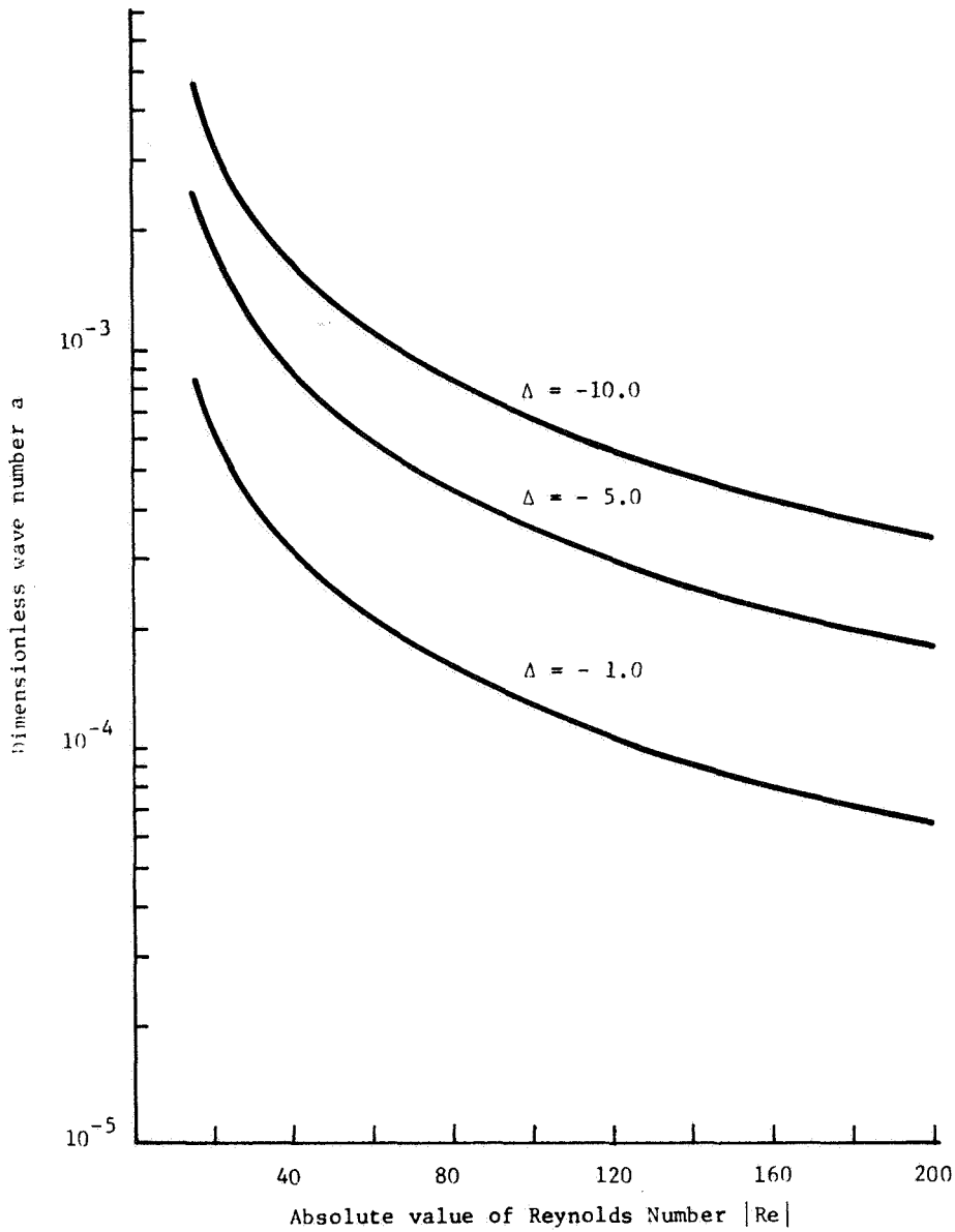
Fig. 6.15(b) Damped disturbances for upward film flow. Surface tension parameter \mathcal{S} = 3715.0 , centrifugal parameter \kappa = 0.0 , dimensionless damping index C_i = 0.005 , gas-pressure parameter \Delta = -1.0, -5.0, -10.0 .
