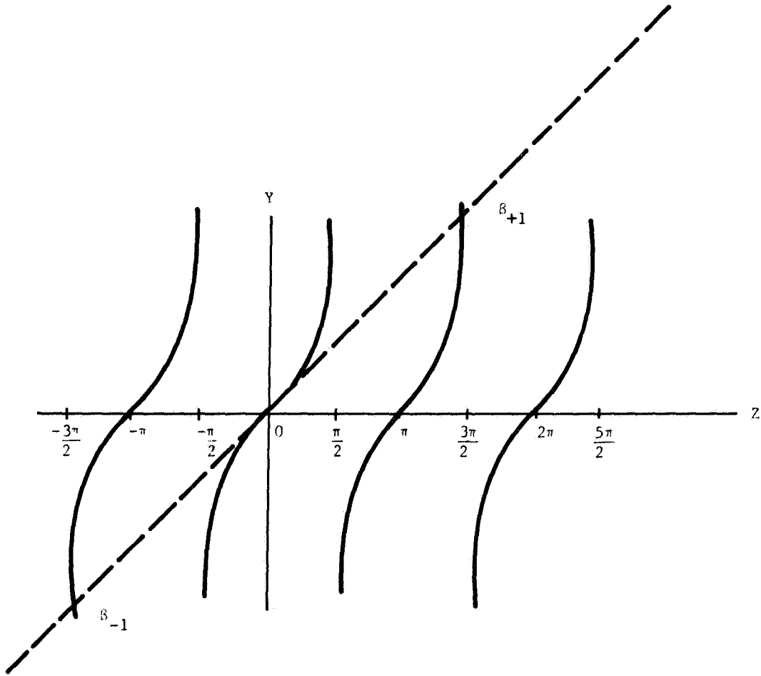
Fig. 5.1 Schematic location of the roots of \mathfrak{Z} = \tan Z ,
