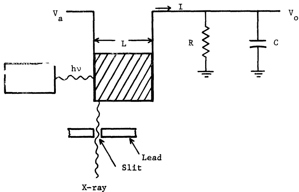
Figure 26. EXPERIMENTAL ARRANGEMENT SHOWING PHOTON AND X-RAY EXCITATION OF CARRIERS AND THE CURRENT MONITORING CIRCUIT.
