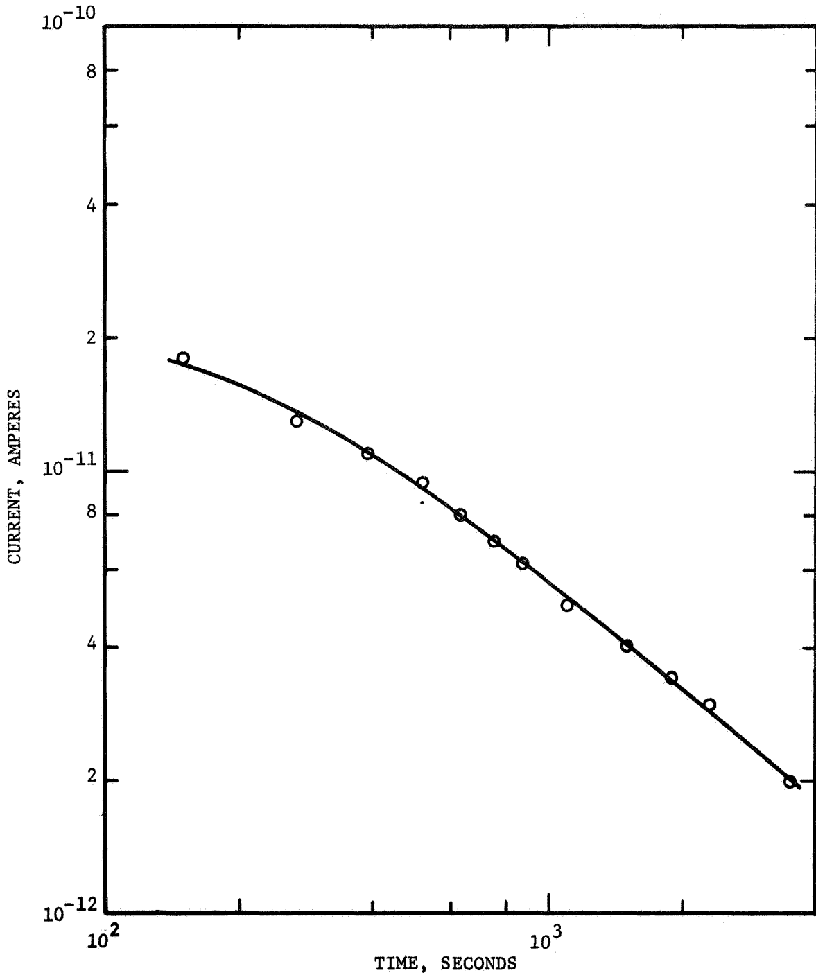
Figure 43. SHORT CIRCUIT CURRENT IN 5000Å FILM OF SiO AFTER ELECTRON IRRADIATION. Electron energy = 5 KW, beam current = 5 \times 10^{-8} amps/cm 2 , irradiation time = 240 sec.
