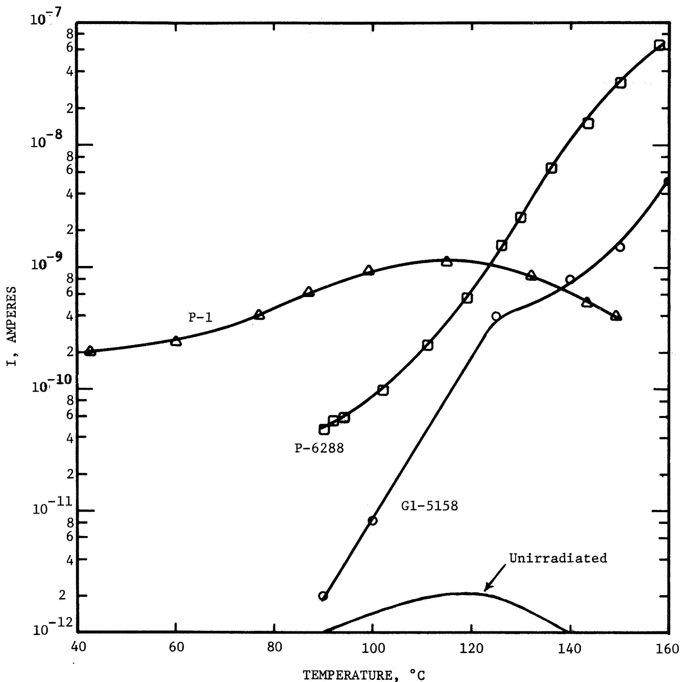
Figure 17. CONDUCTION CURRENT VERSUS TEMPERATURE IN PET UNDER TRANSIENT TEMPERATURE CONDITIONS.
