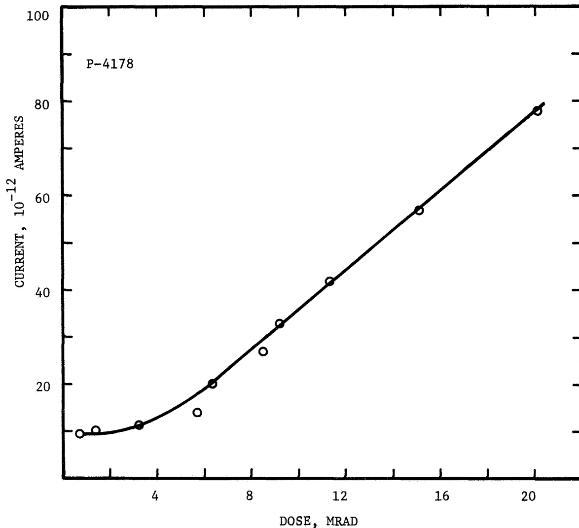
Figure 11. CURRENT IN 1 MIL PET AS A FUNCTION OF ACCUMULATED \gamma -DOSE.
