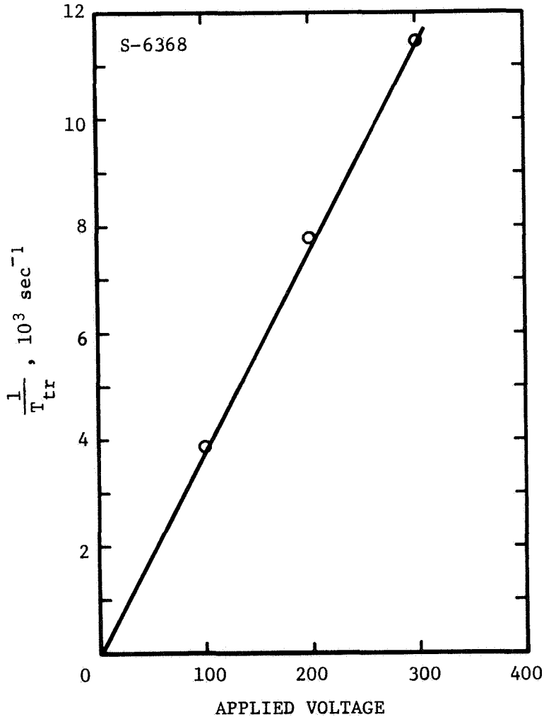
(b) INVERSE TRANSIT TIME VERSUS APPLIED VOLTAGE
