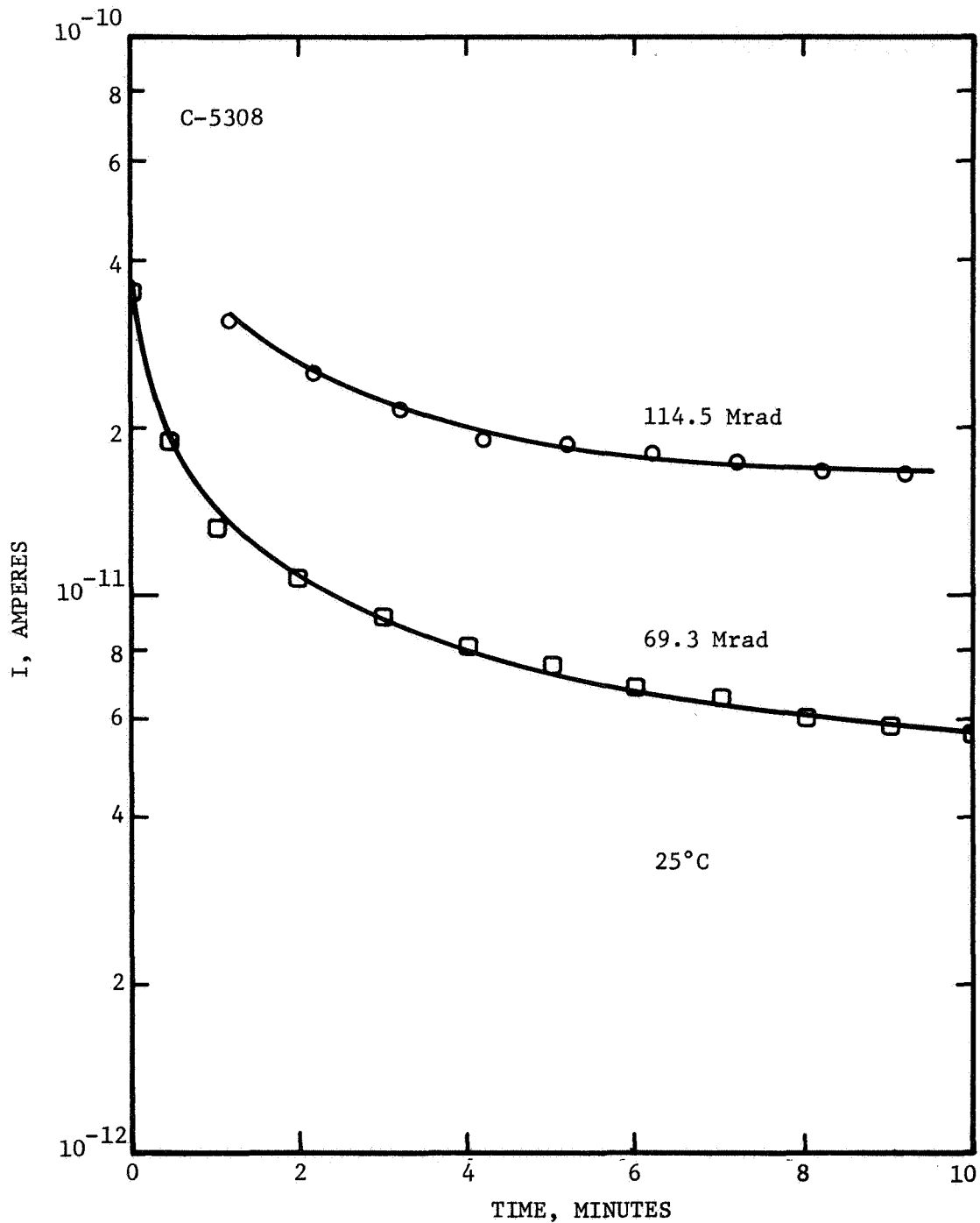
Figure 15. FIRST ORDER CURRENT DECAY OF 10 MIL PET IRRADIATED IN AIR. No voltage applied during irradiation, applied voltage during current measurement = 1000 volts
