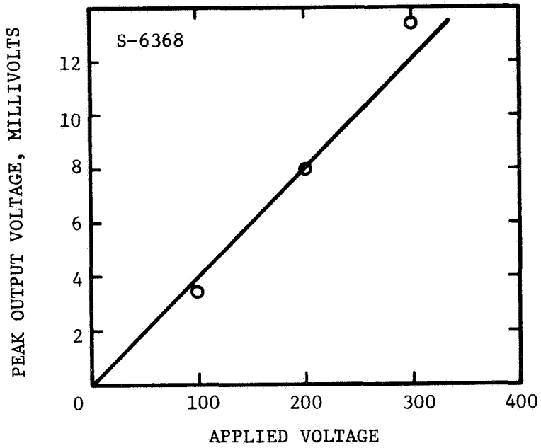
(a) PEAK OUTPUT VOLTAGE VERSUS APPLIED VOLTAGE
