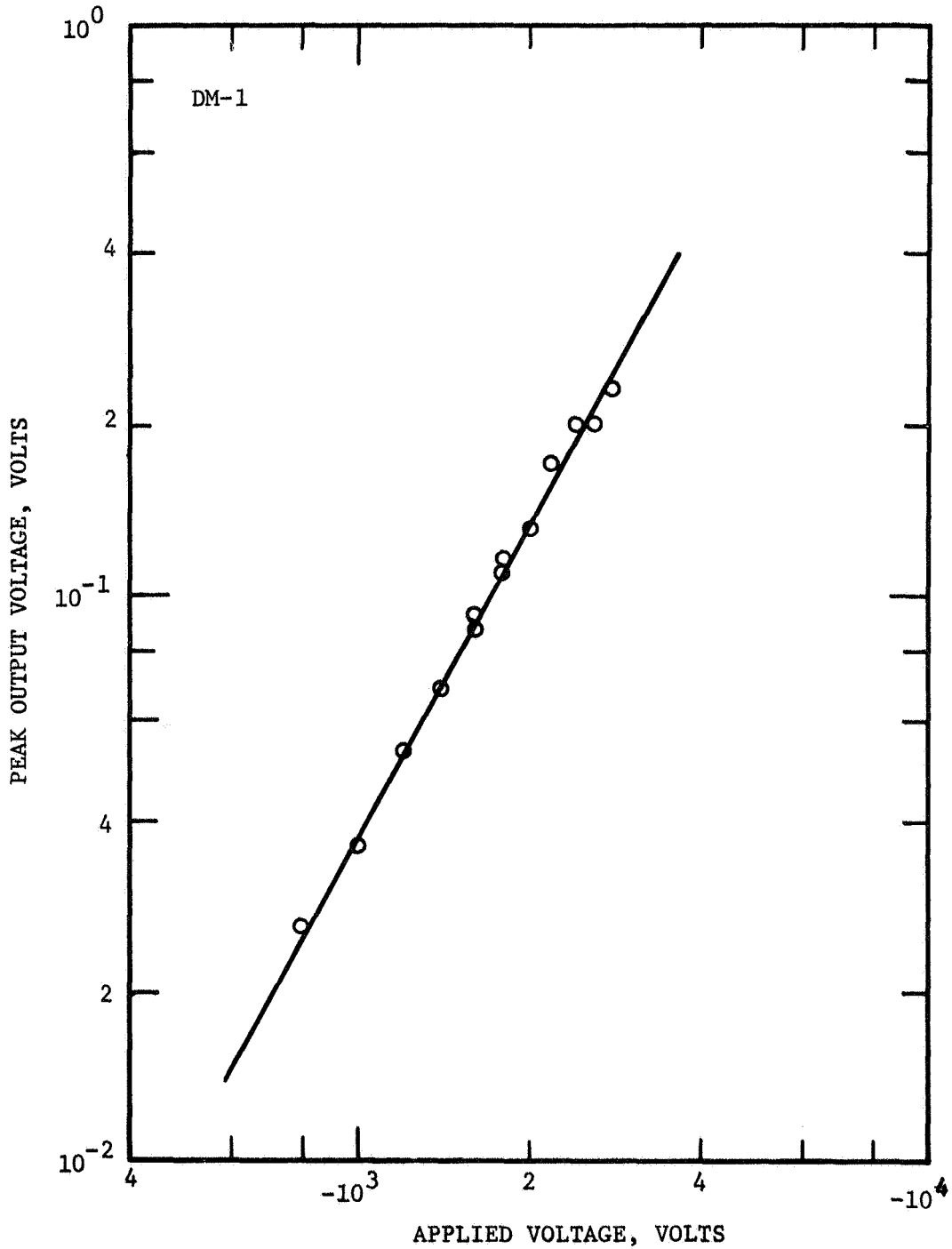
Figure 31. PEAK OUTPUT VOLTAGE VERSUS APPLIED VOLTAGE FOR A-AXIS OF DIMETHYLTEREPHTHALATE. 300 Å silver electrodes with silver paste guard ring, thickness = 0.45 cm, area = 0.37 cm 2 , R = 7 x 10 5 ohms.
