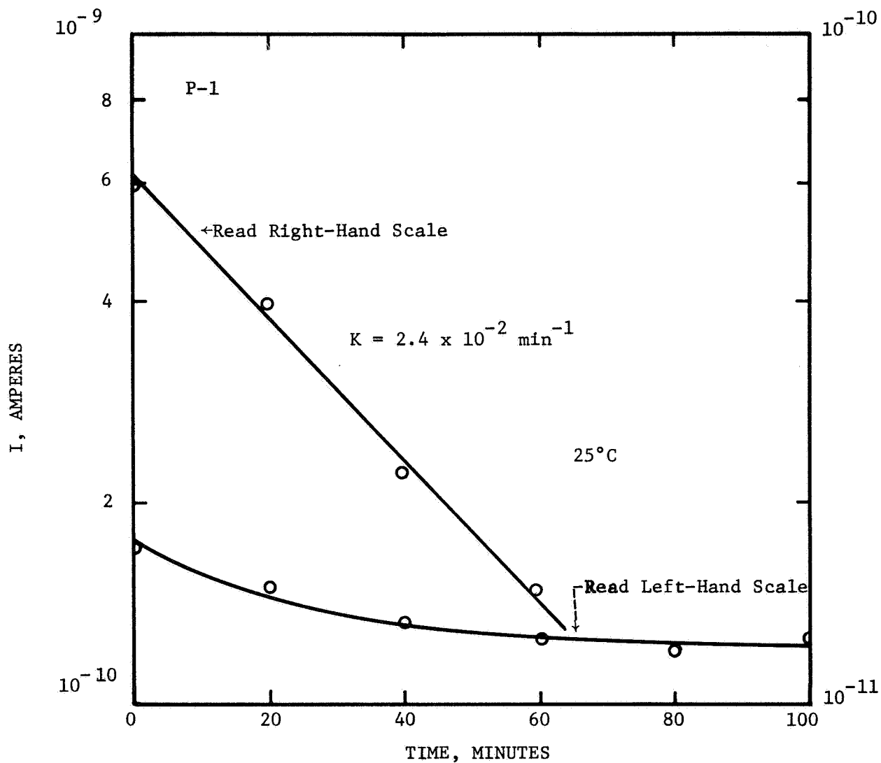
Figure 16. FIRST ORDER CURRENT DECAY IN IRRADIATED 1 MIL PET. V = 100 volts 300 A aluminum electrodes with area = 3.88 \text{ cm}^2 Dose = 6 Mrad
