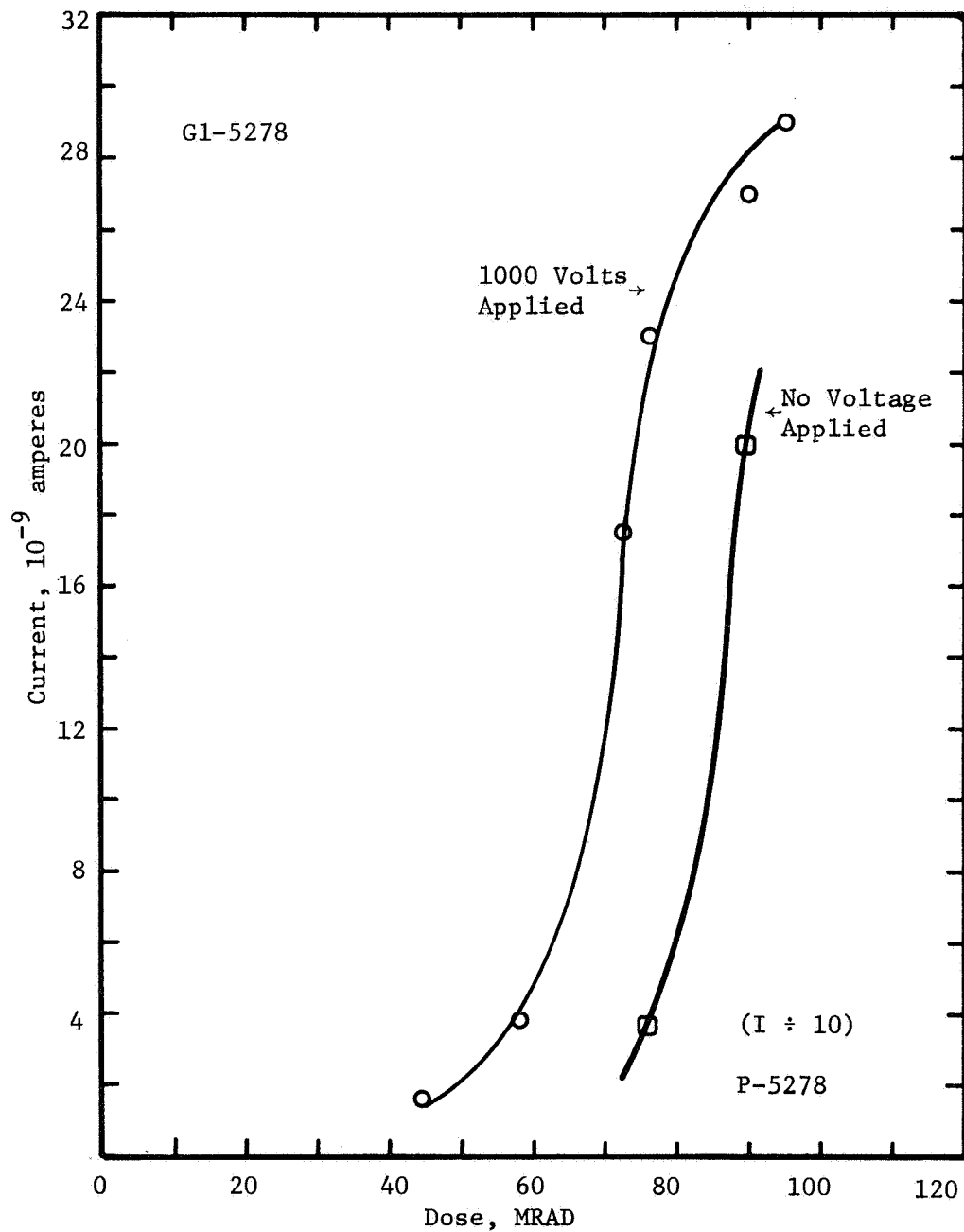
Figure 12. CURRENT IN 10 MIL PET AS A FUNCTION OF THE ACCUMULATED \gamma -DOSE. Applied voltage = 1000 volts, area = 3.88 cm 2 , 830 Å aluminum electrodes, dose rate = 0.19 Mrad hr -1 , \circ ...1000 volts applied during irradiation, \square ...no voltage applied during irradiation.
