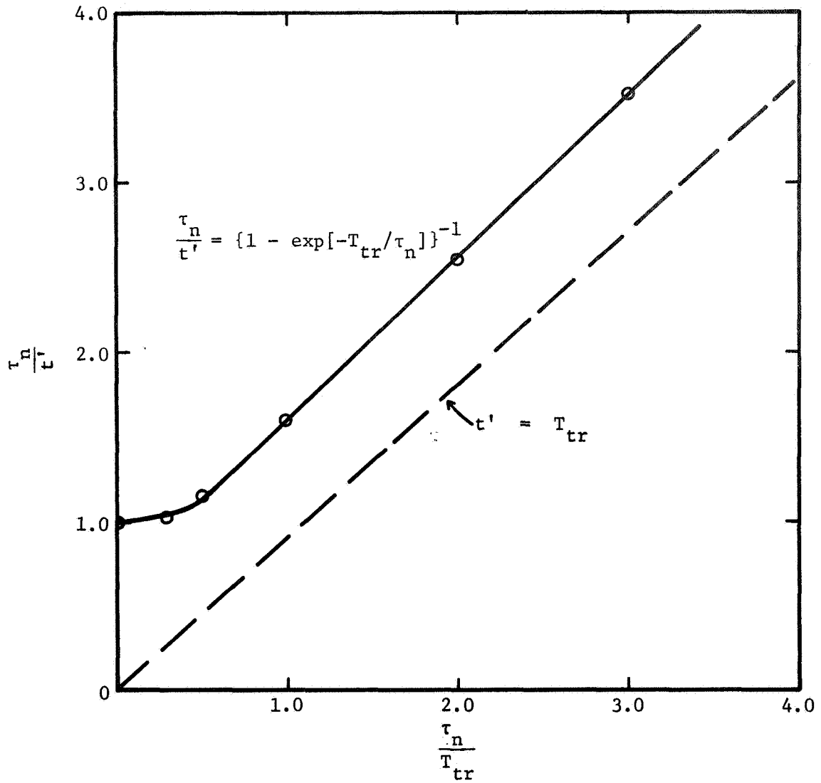
Figure 27. PLOT OF THE RELATION BETWEEN EFFECTIVE DRIFT TIME, t' , AND THE CARRIER TRANSIT TIME, T_{tr} , NORMALIZED TO THE CARRIER LIFETIME, \tau_n .
