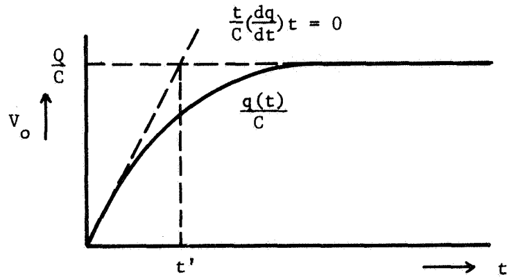
Figure 25. OUTPUT VOLTAGE OF INTEGRATING CIRCUIT WHEN THE CARRIER LIFETIME IS SHORT.
