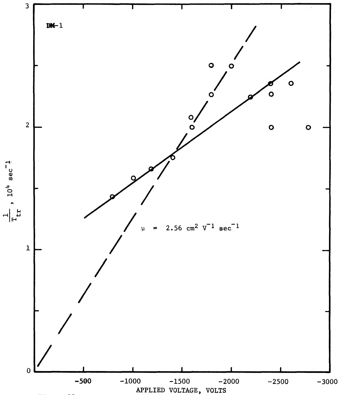
Figure 32. INVERSE TRANSIT TIME VERSUS APPLIED VOLTAGE FOR A-AXIS OF DIMETHYLTEREPHTHALATE.
