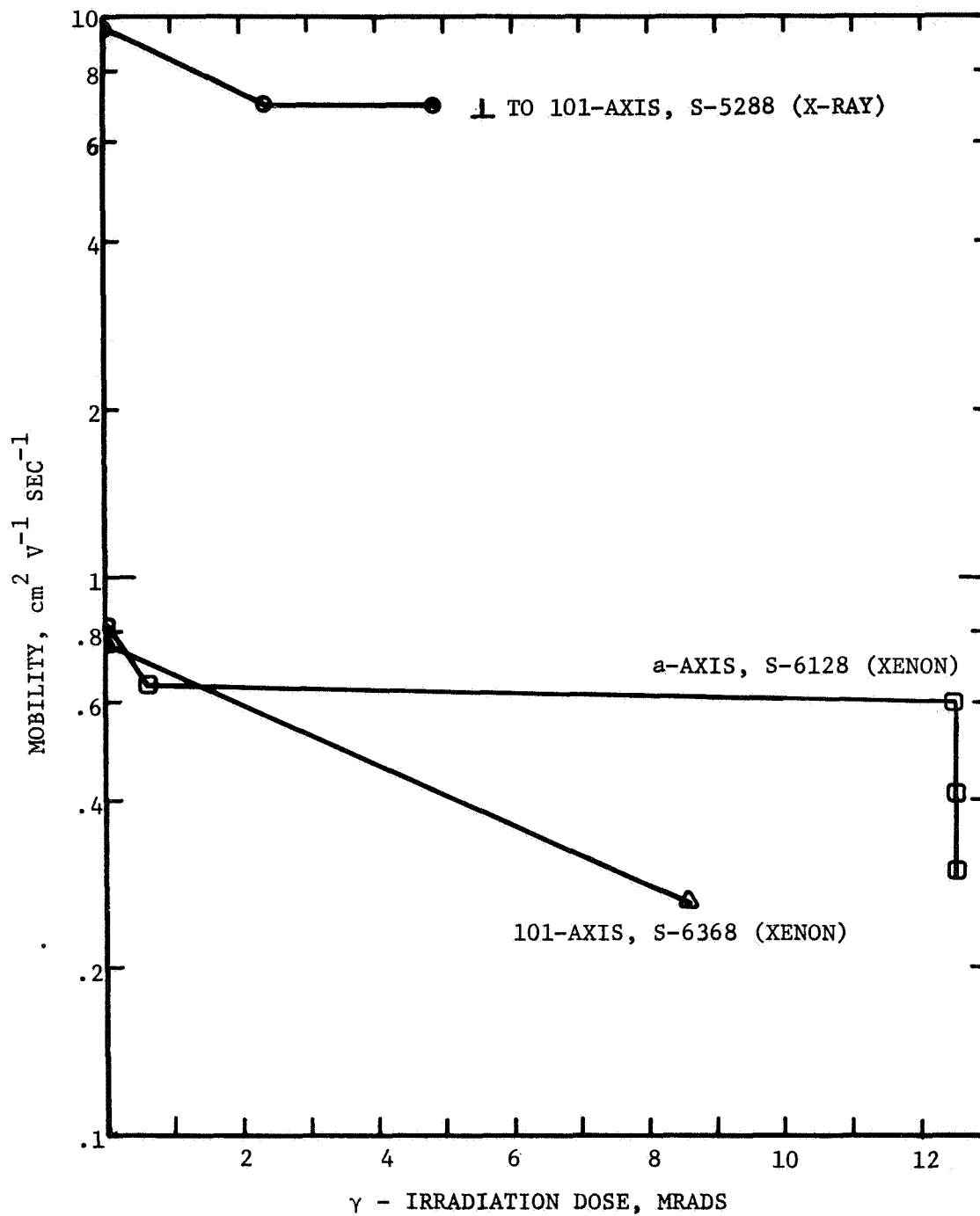
Figure 33. EFFECT OF \gamma - IRRADIATION ON HOLE MOBILITY IN DIMETHYLTEREPHTHALATE.
