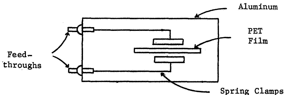
Figure 10. SAMPLE HOLDER FOR \gamma -IRRADIATION MEASUREMENTS.
