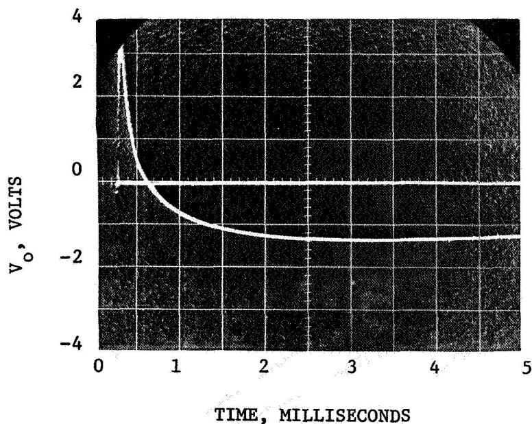
b. OUTPUT VOLTAGE PULSE ACROSS 10^7 OHMS
