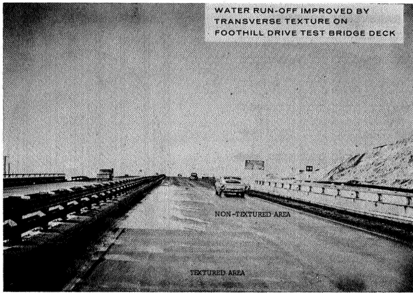
Figure 5.- Pavement drainage.
