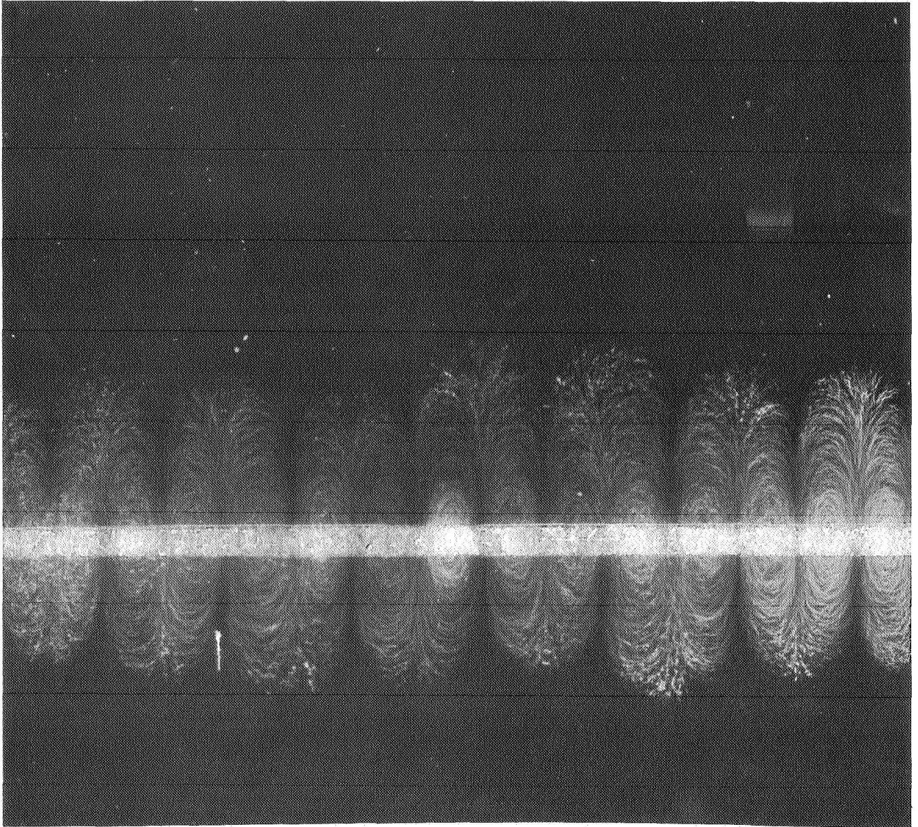
Fig. 6 Cellular convection resulting from electroconvective instability, as seen looking down at the interface (looking in the -z direction in Fig. 2b).
