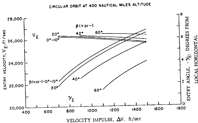
Figure 52. Effects of Angle of Deorbiting Impulse on Reentry
