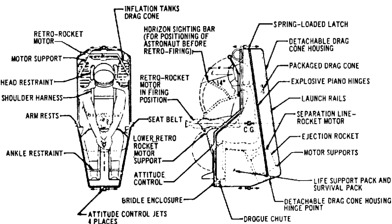
Figure 132. Paracone Survival Pack
