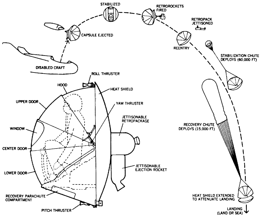
Figure 126. EGRESS Vehicle
