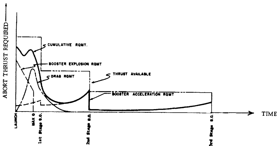
Figure 24. Abort Thrust Requirement Versus Flight Time
