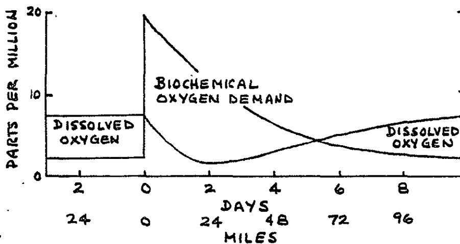
Fig. A-1.1 Assumptions in a hypothetical pollution case are a stream flow of 100 cfs, a discharge of raw sewage from a community of 40,000 and a water temperature of 25°C, with typical variation of dissolved oxygen and BOD. After Bartsch and Ingram, 1959.
