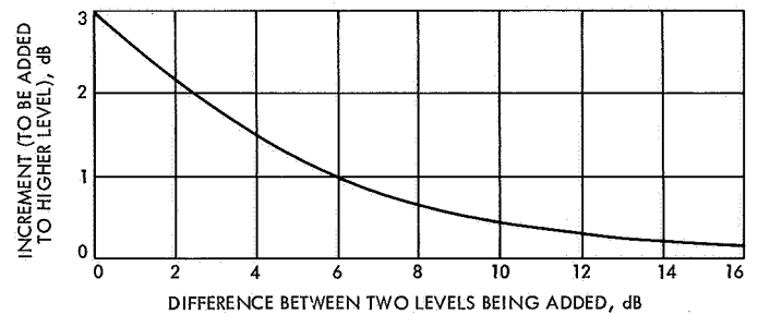
Fig. B-7. Chart for combining noise levels
