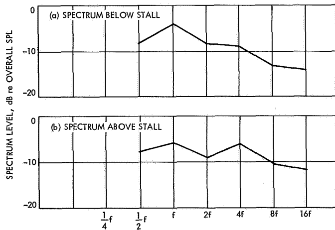
Fig. 10. Octave band vortex noise spectrum below stall (a), and above stall (b), (adapted from Ref. 13)
