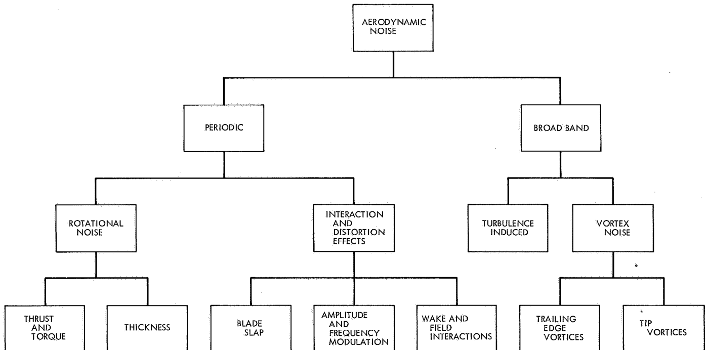
Fig. 3. Sources of aerodynamic noise
