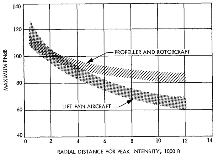
Fig. 17. Noise generated by STOL aircraft, 50,000 to 95,000 lb gross weight (adapted from Deckert, Ref. 23)
