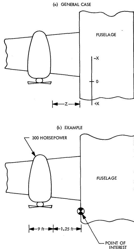
Fig. B-1. Near-field axis system
