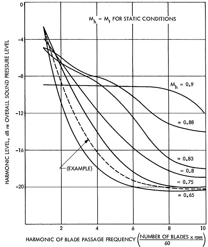
Fig. B-6. Harmonic distribution of rotational noise
