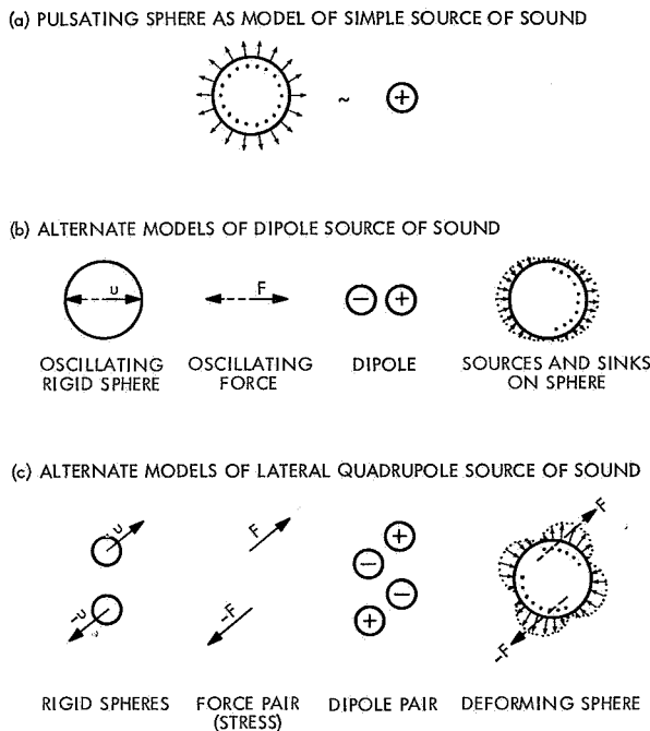
Fig. 1. Elementary sources of sound
