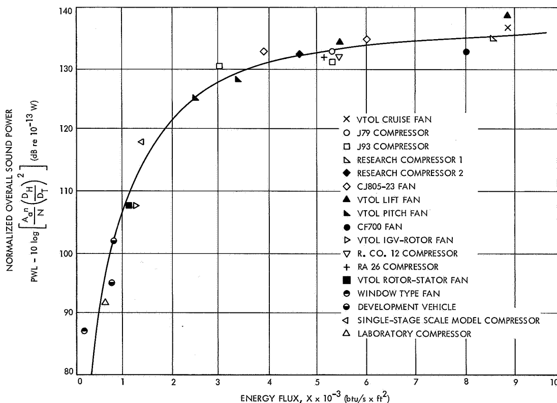
Fig. 16. Normalized overall power of compressor and fan noise (adapted from Ref. 26)
