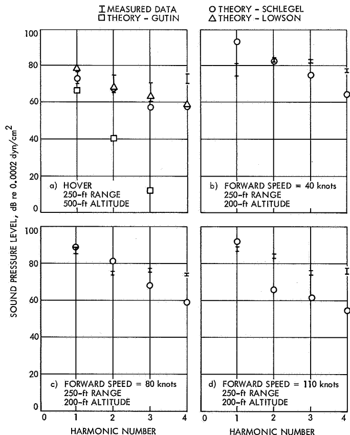
Fig. 7. Comparison of theories with experimental data at the side of a helicopter
