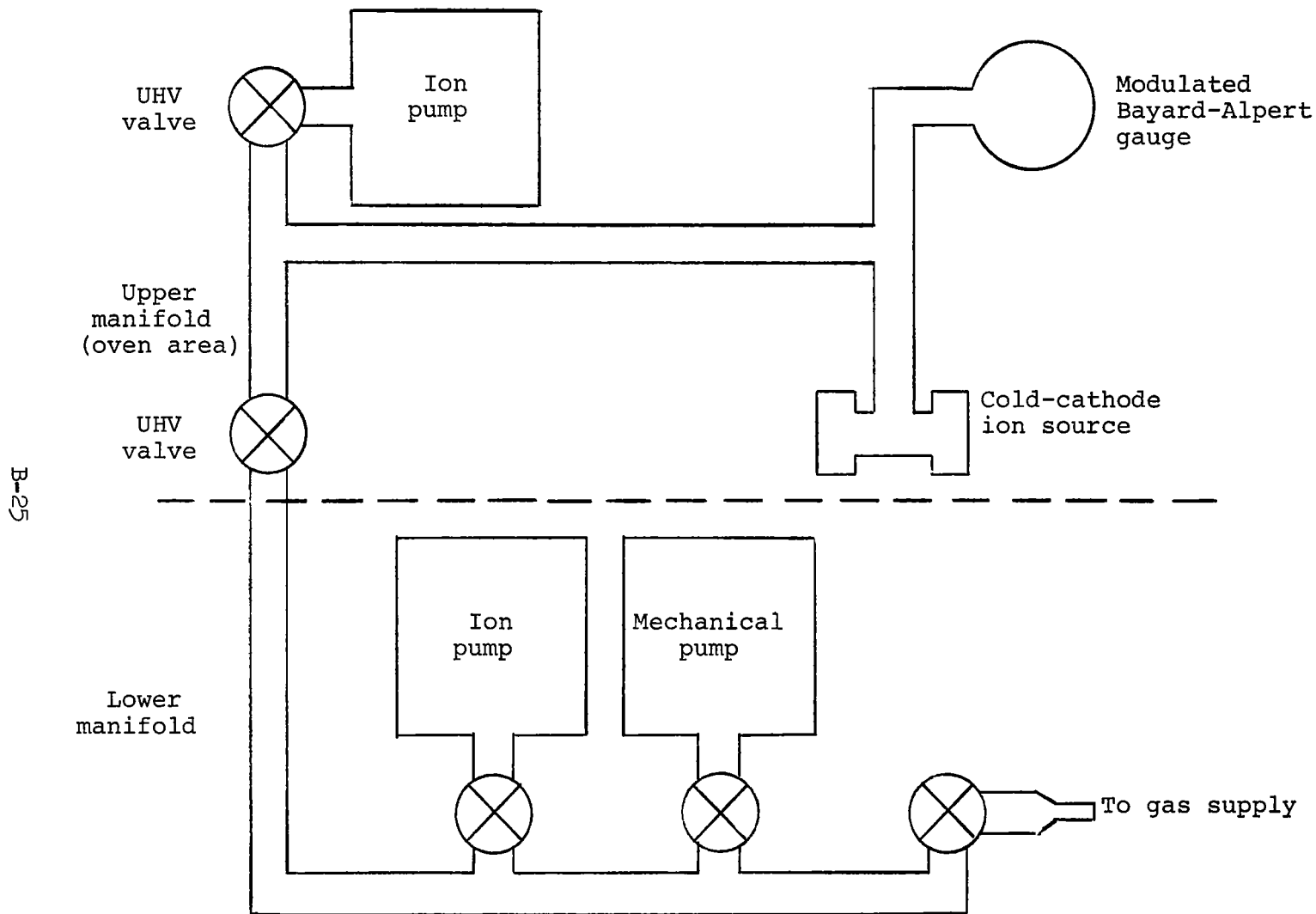
Figure B-5.- Vacuum system schematic
