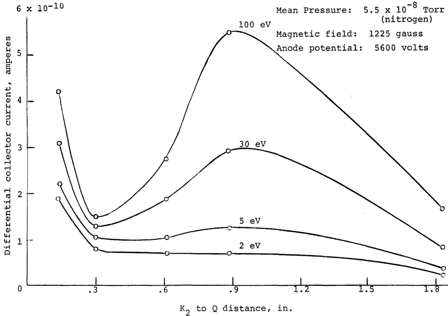
Figure B-11.- Differential collector current vs. distance for selected energy intervals, for V_{K1} = +40 volts
