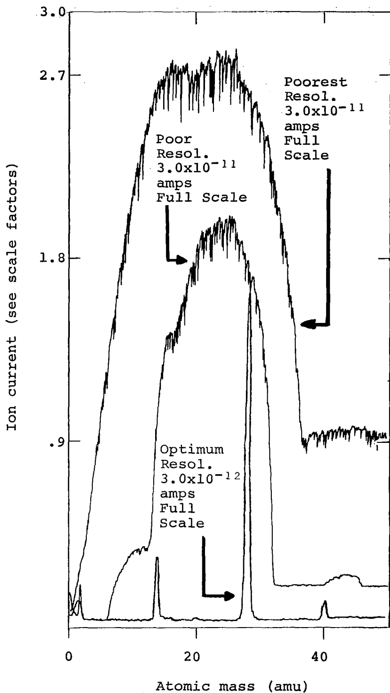
Figure 15.- Sensitivity vs. resolution- low mass range
