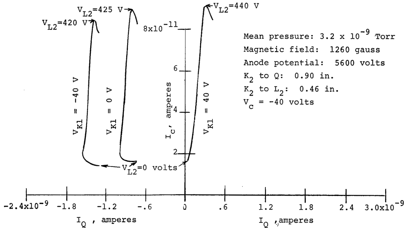
Figure B-18.- Effect of lens potential variations on I_c and I_Q at position 3, for V_{K1} = +40 , Zero and -40 volts
