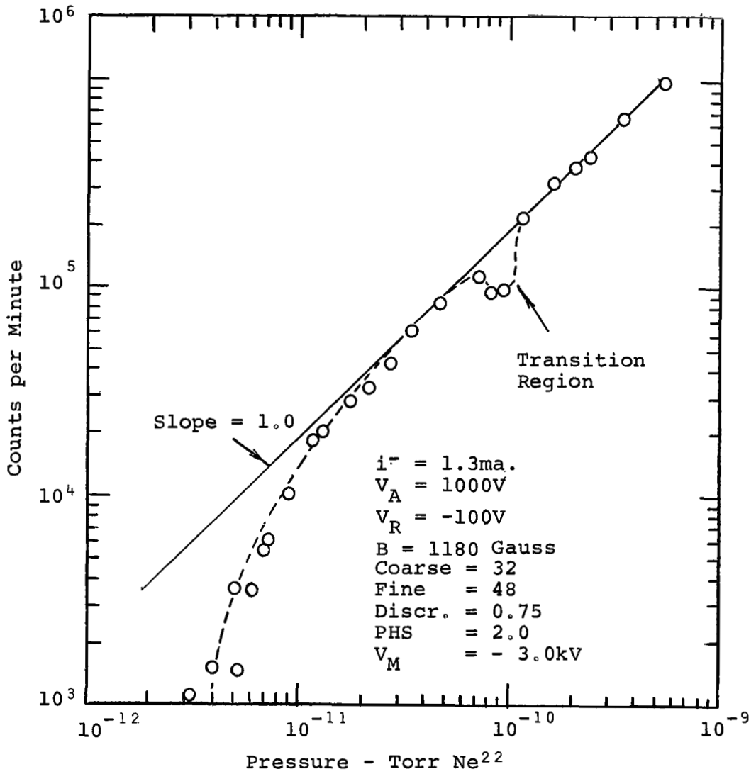
Fig. 35 Counting rate vs. Pressure Ne^{20} & Ne^{22} .
