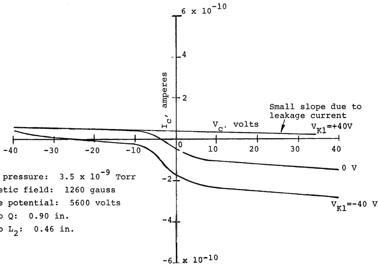
Figure B-19.- Ion and electron energy spectra at focusing potential for position 3:
