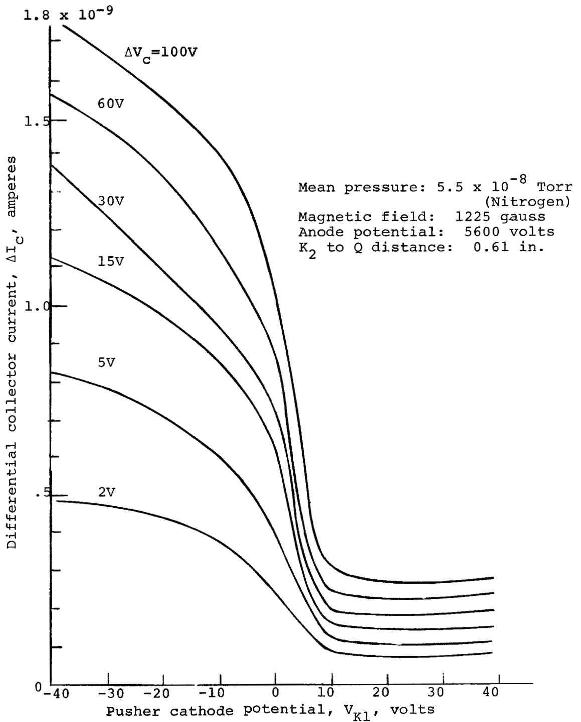
Figure B-9.— Differential collector current vs. pusher cathode potential for selected intervals of collector potential
