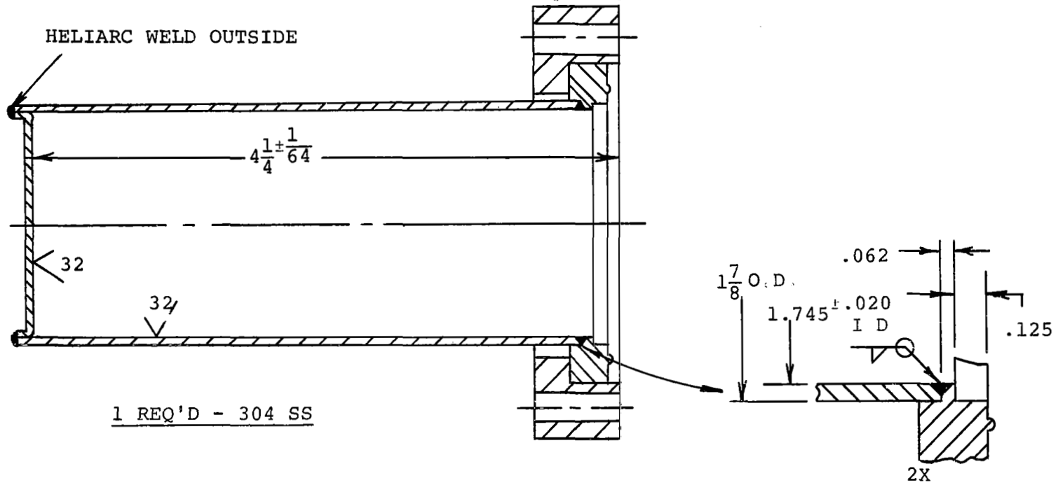
Fig. 51 CCIS Housing
