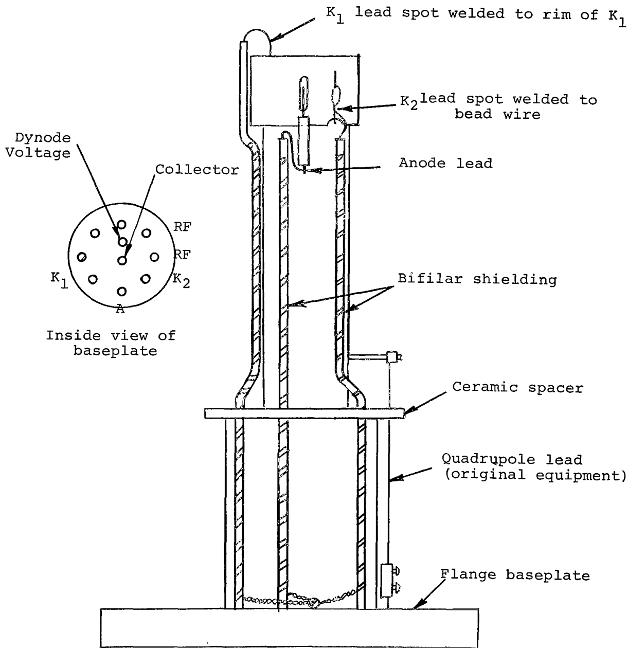
Figure 38 - Lead Assembly
