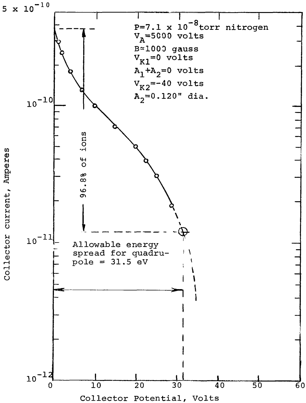
Figure A-10.— Unfocused ion energy distribution at ion collector
