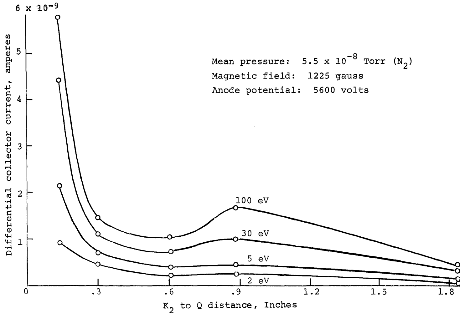
Figure B-12.- Differential collector current vs. distance for selected energy intervals, for V_{K1} = zero volts
