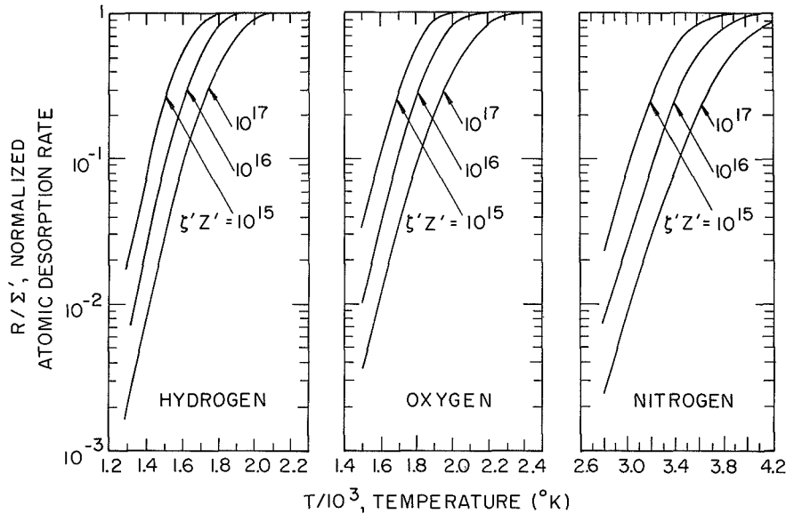
Fig. 2. Theoretical prediction of the degree of dissociation of H_2 , O_2 , and N_2 by a catalyst at temperature T. Z' is the rate at which molecules impinge upon the surface, \zeta' is the equilibration probability, R is the rate at which atoms leave the surface, and \Sigma' is the maximum possible value of R , i. e., \Sigma' = 2\zeta'Z' .
