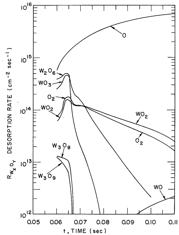
Fig. 22. Theoretical flash-desorption curves for the reaction of oxygen with a tungsten surface. (Conditions are identical to those for Fig. 21, but included here are the results for all of the major species, and the time scale has been enlarged for clarity.)
