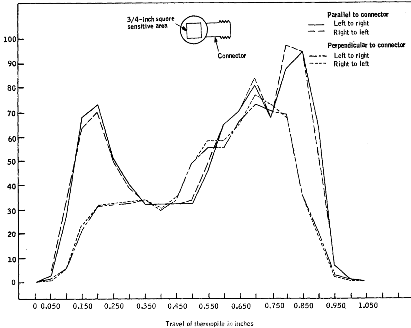
Figure 11. Spatial Sensitivity of Detector for 0.093-Inch Diameter Beam
