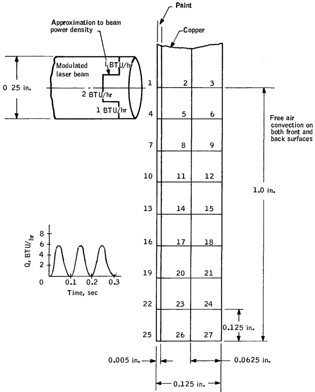
Figure A1. Geometry of Thermal Analysis
