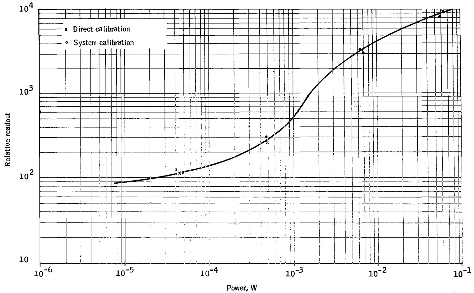
Figure 15. Calibration Curve
