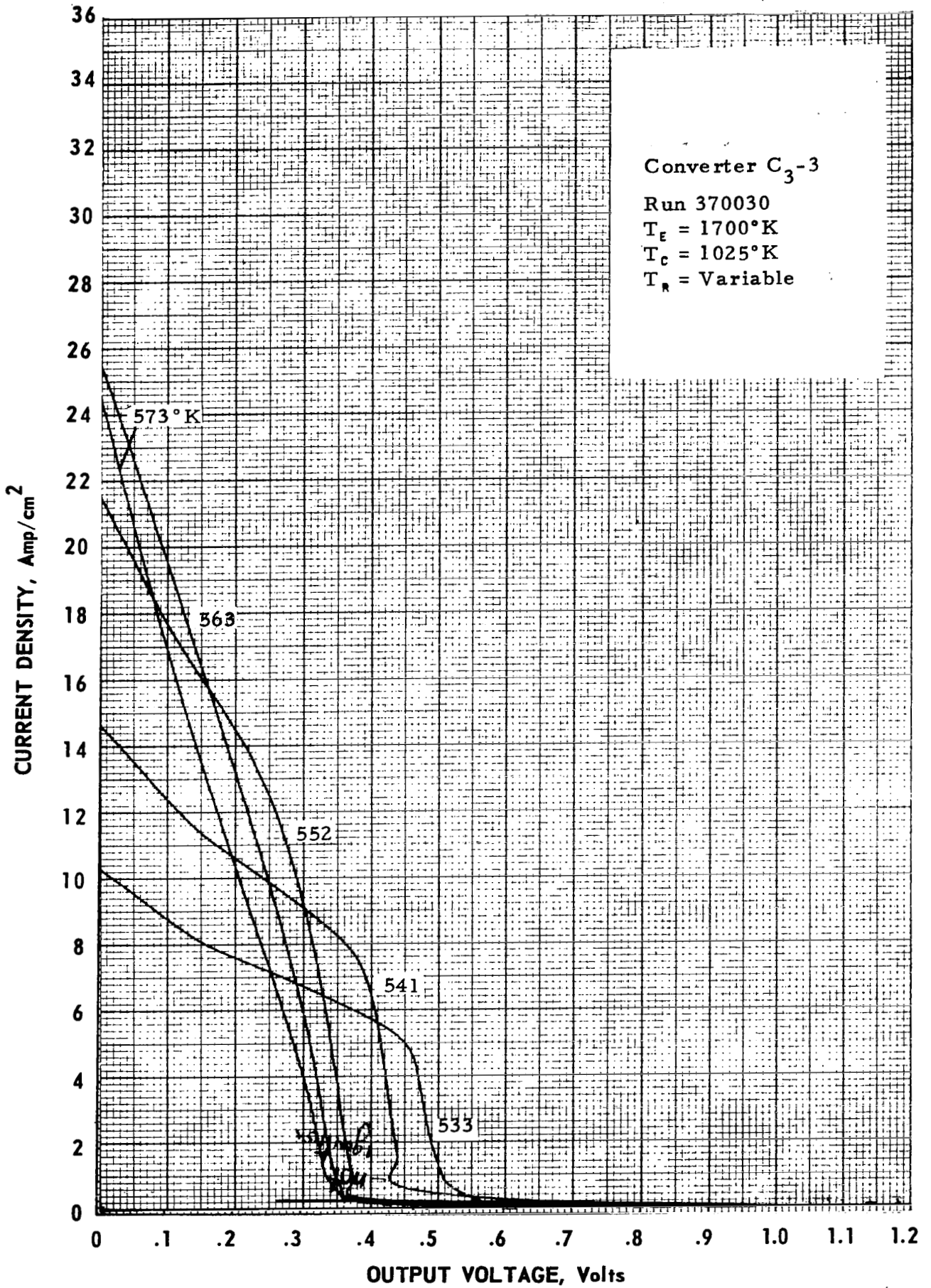
Figure C-16. Cesium Temperature Family of Converter C 3 -3 at T E = 1700°K.
