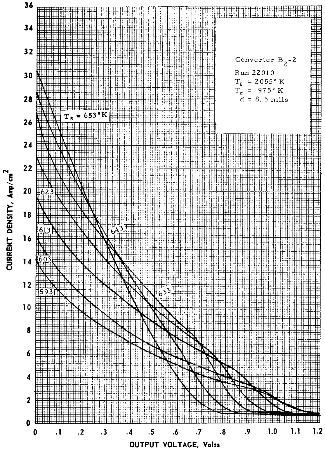
Figure B-4 Cesium-Temperature Family of Converter B 2 -2 at T e = 2055° K.
