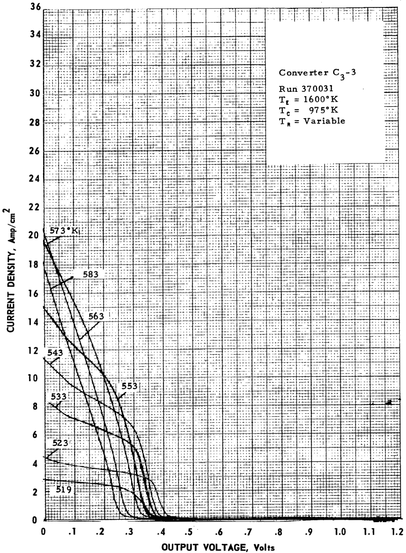
Figure C-15. Cesium Temperature Family of Converter C 3 -3 at T e = 1600°K.
