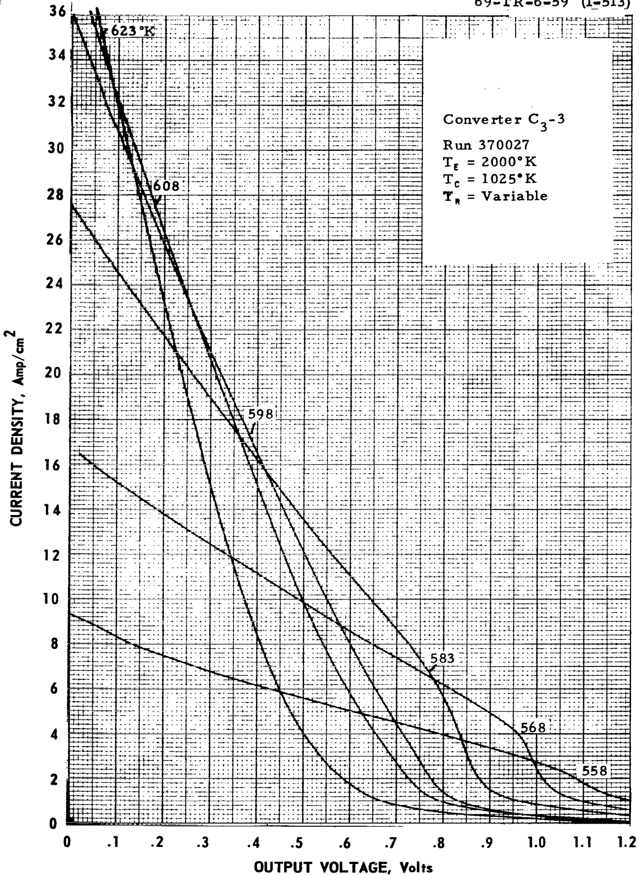
Figure C-19. Cesium Temperature Family of Converter C 3 -3 at T E = 2000°K.
