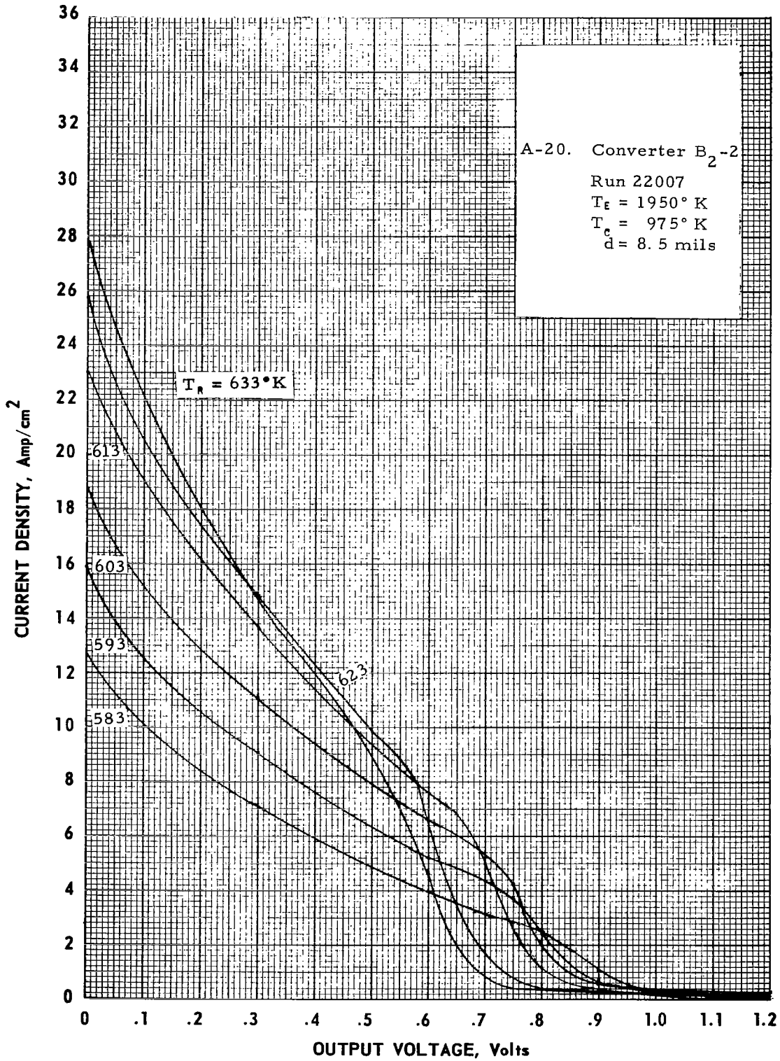
Figure B-3 Cesium-Temperature Family of Converter B 2 -2 at T g = 1950° K
