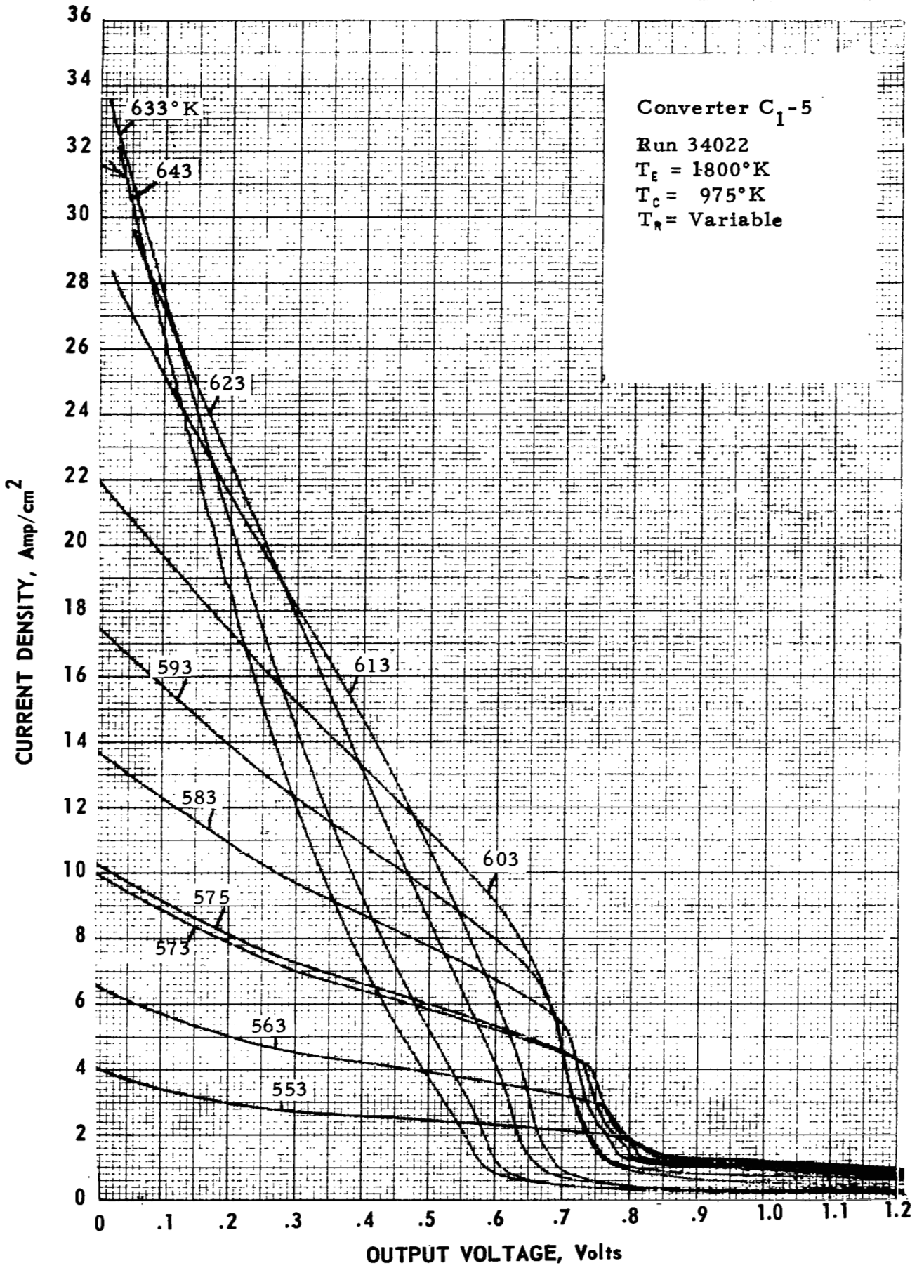
Figure C-8. Cesium Temperature Family of Converter C 1 -5 at T E = 1800°K.
