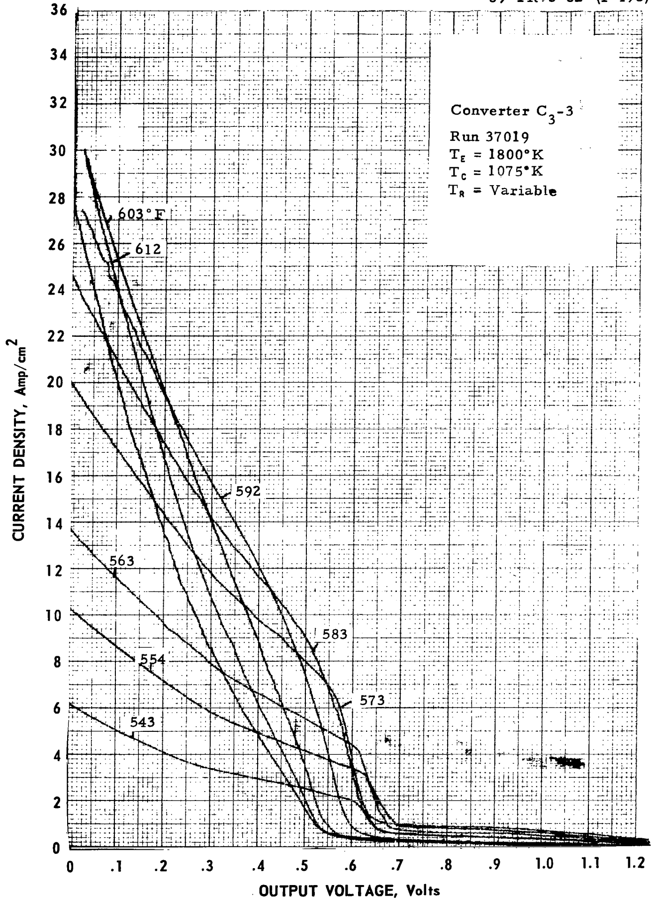
Figure B-24. Cesium Temperature Family of Converter C_3-3 at T_E = 1800^\circ K .
