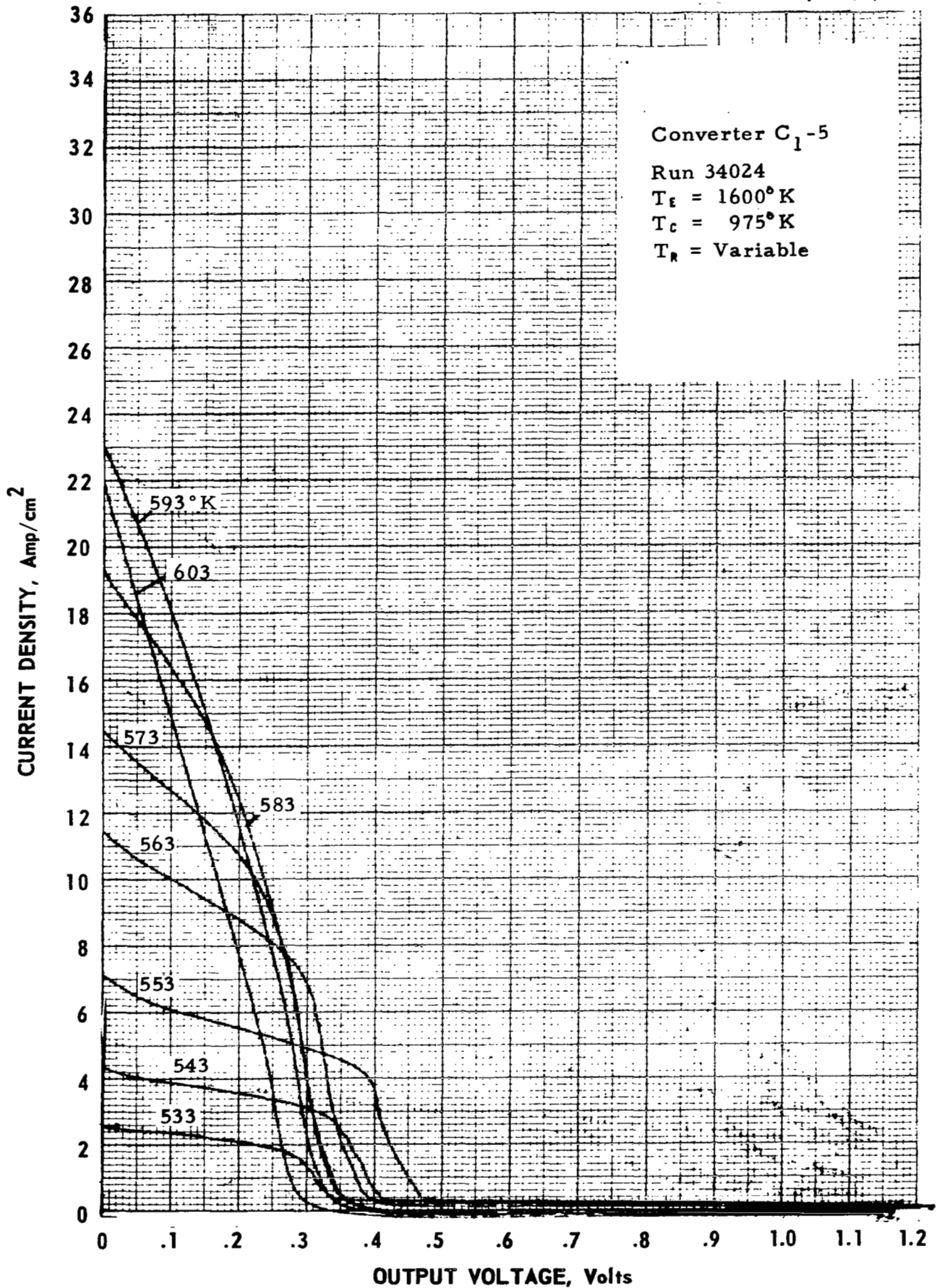
Figure C-6. Cesium Temperature Family of Converter C 1 -5 at T E = 1600°K.
