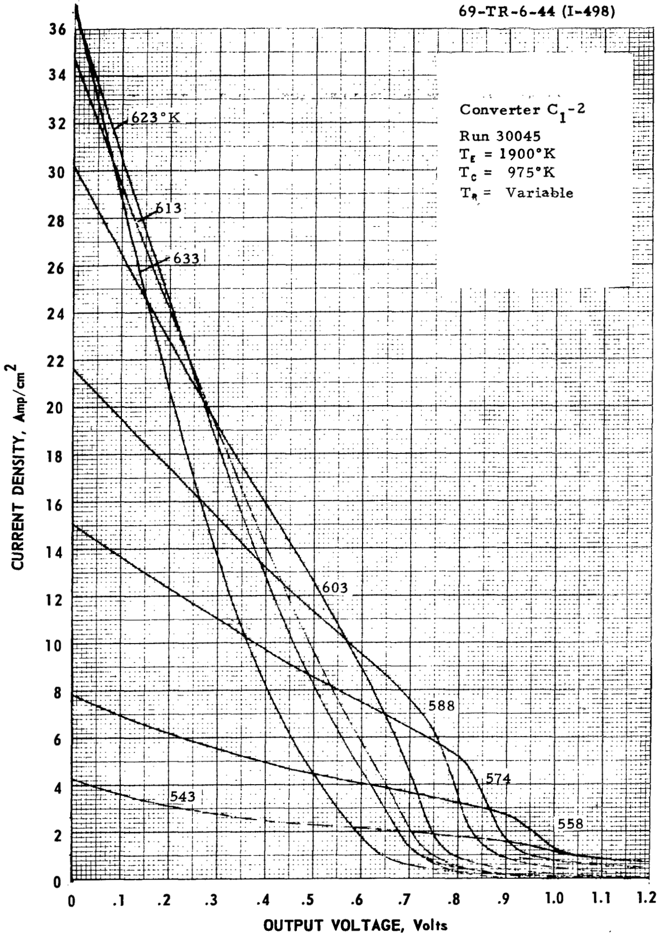
Figure C-4. Cesium Temperature Family of Converter C 1 -2 at T g = 1900°K.
