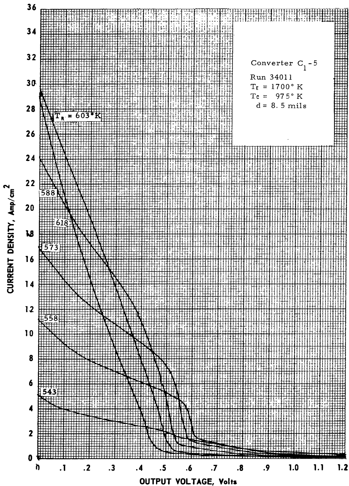
Figure B-18. Cesium-Temperature Family of Converter C 1 -5 at T E = 1700° K B-18
