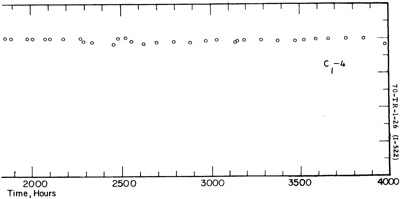
t Data for Converter C 1 -4 at T E = 1950° K.
