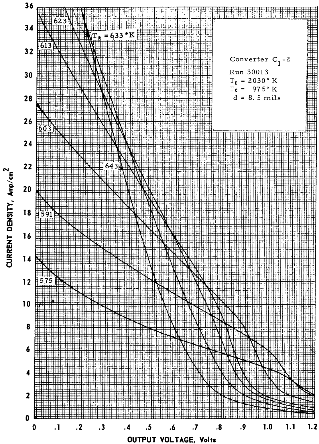
Figure B-12. Cesium-Temperature Family of Converter C_1-2 at T_e = 2030^\circ\text{K} .
