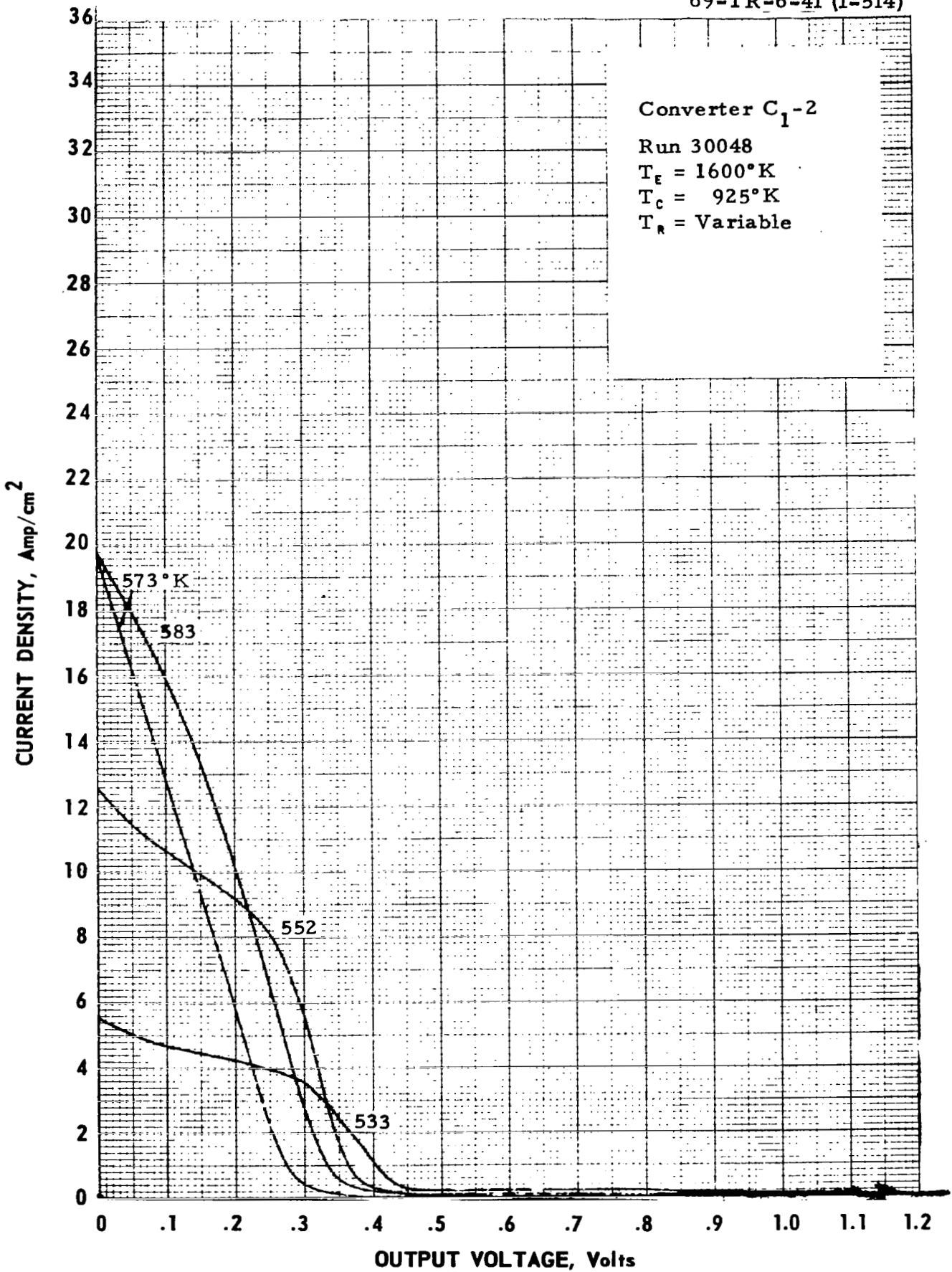
Figure C-1. Cesium Temperature Family of Converter C 1 -2 at T E = 1600°K. C-1
