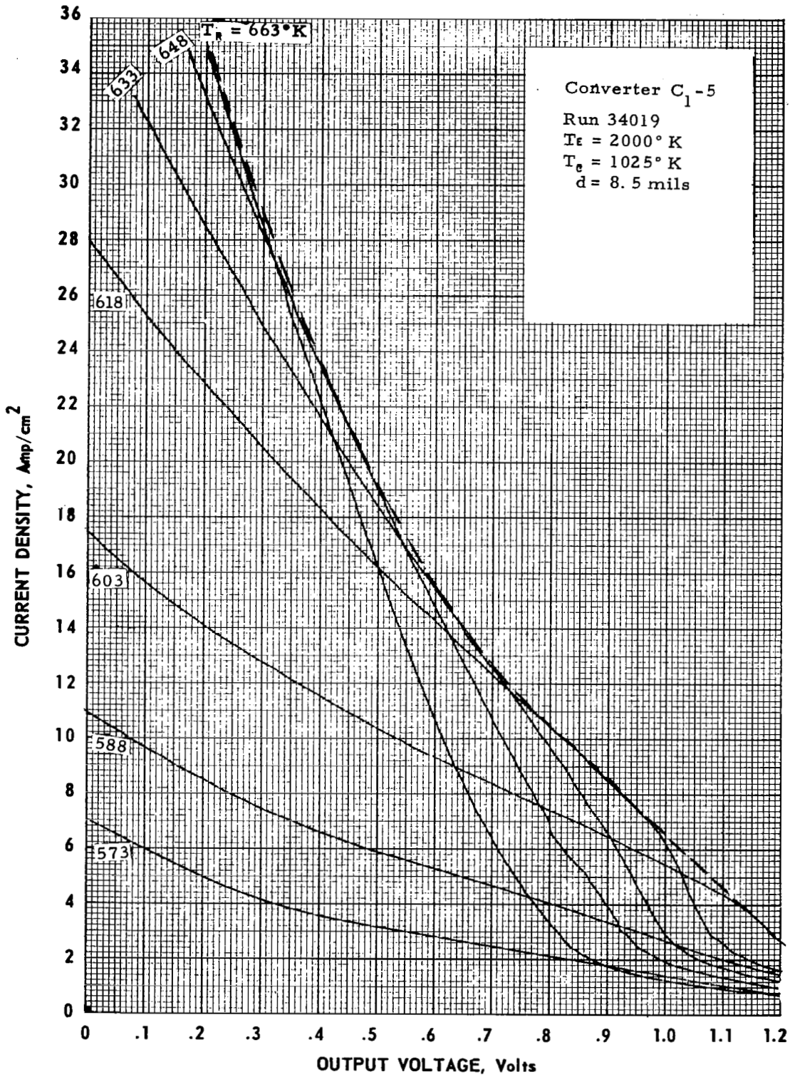
Figure B-21. Cesium-Temperature Family of Converter C 1 -5 at T E = 2000° K.
