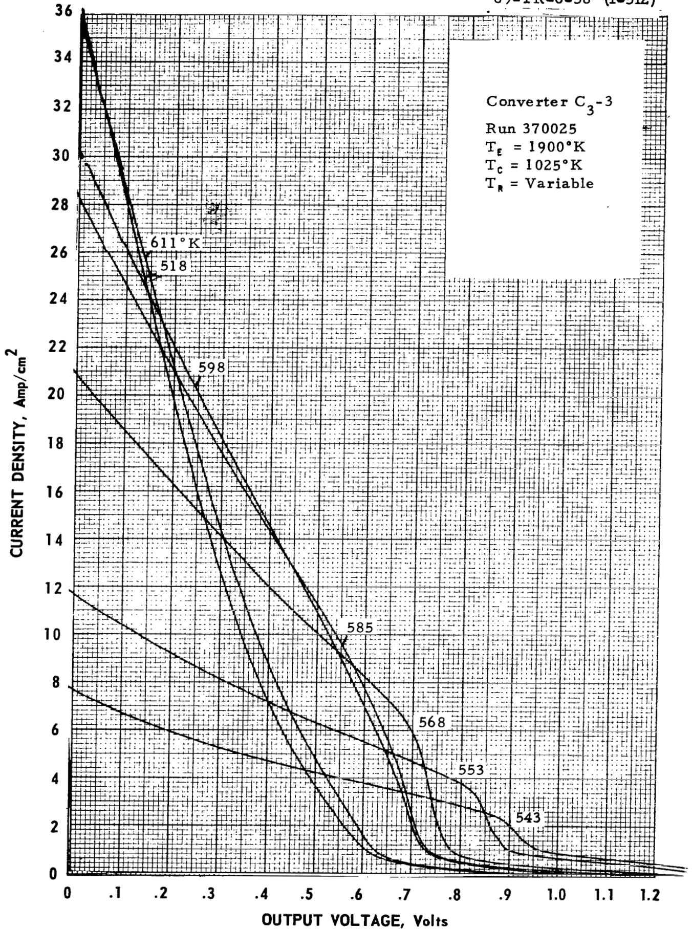
Figure C-18. Cesium Temperature Family of Converter C 3 -3 at T e = 1900°K.
