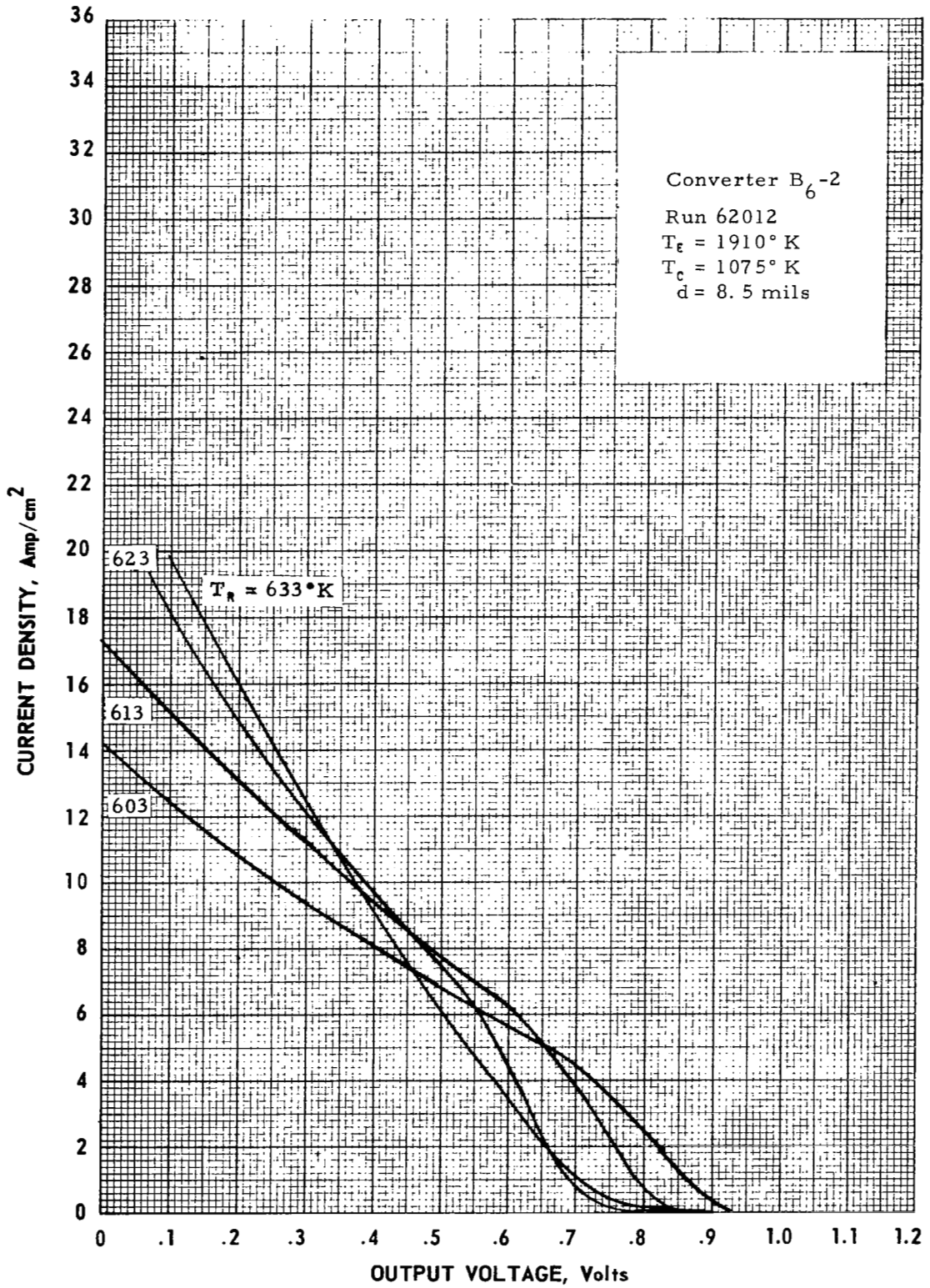
Figure B-8. Cesium-Temperature Family of Converter B 6 -2 at T e = 1910° K.
