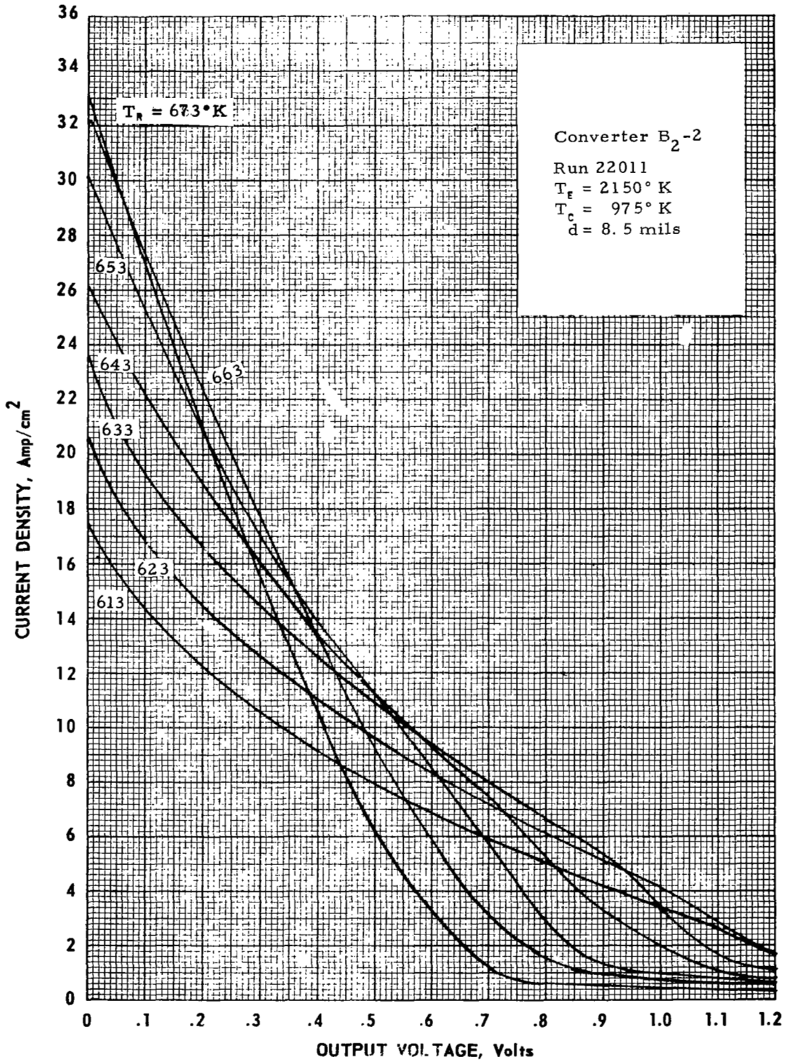
Figure B-5 Cesium-Temperature Family of Converter B 2 -2 at T_E = 2150^\circ K .
