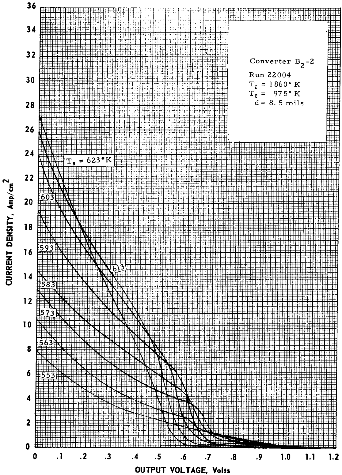
Figure B-2 Cesium-Temperature Family of Converter B 2 -2 at T E = 1860°K.
