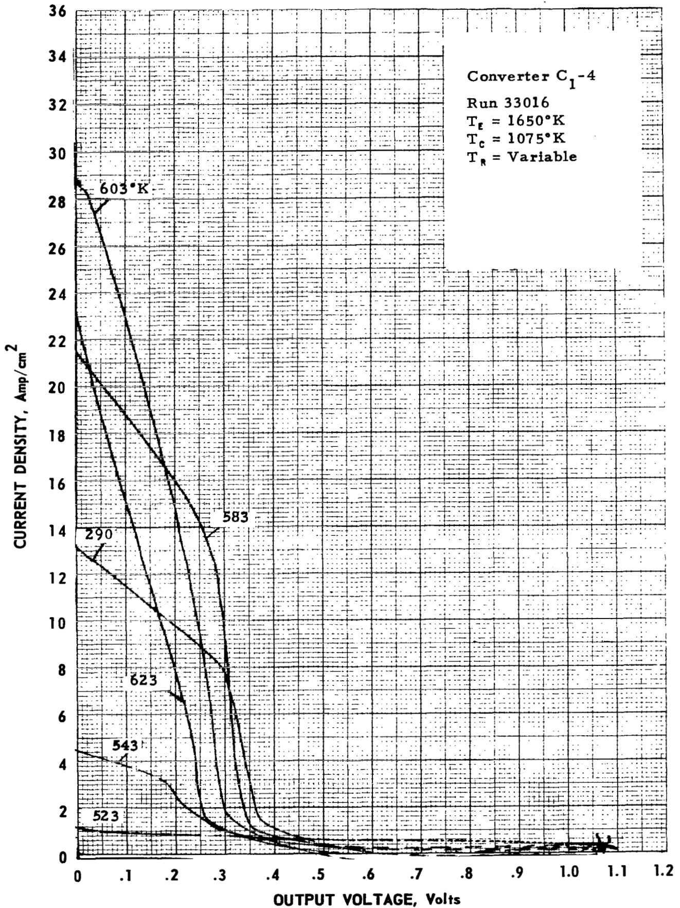
Figure C-11. Cesium Temperature Family of Converter C 1 -4 at T g = 1650°K.
