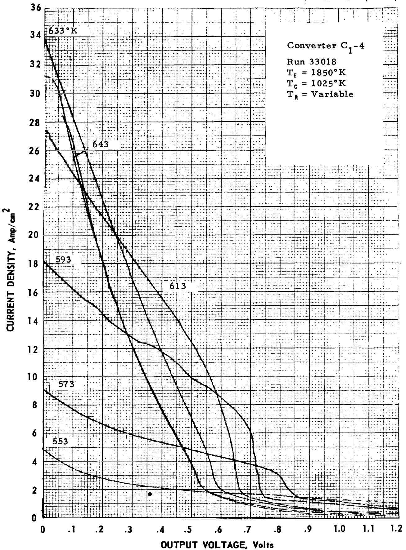
Figure C-13. Cesium Temperature Family of Converter C 1 -4 at T g = 1850°K.
