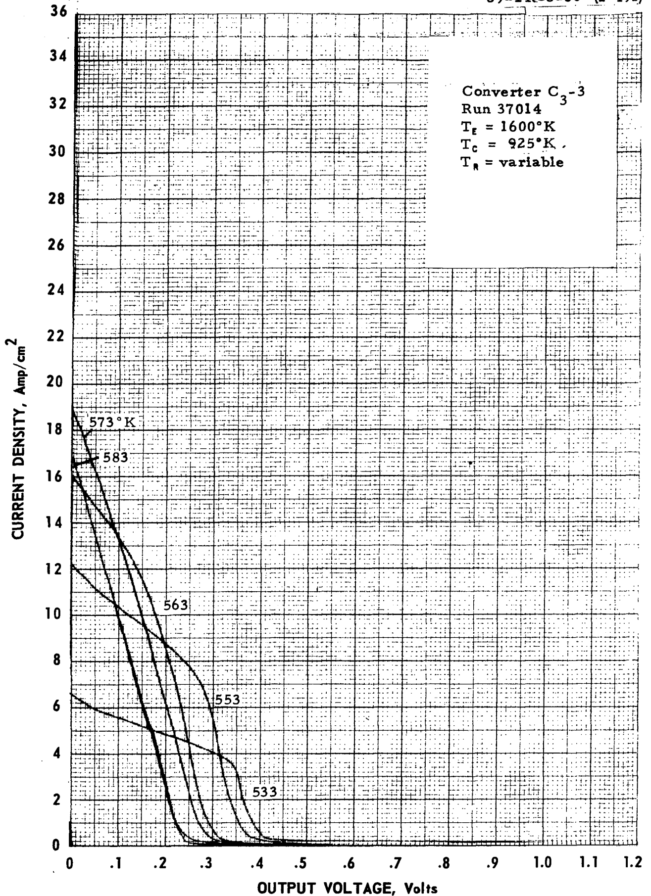
Figure B-22. Cesium Temperature Family of Converter C 3 -3 at T e = 1600°K.
