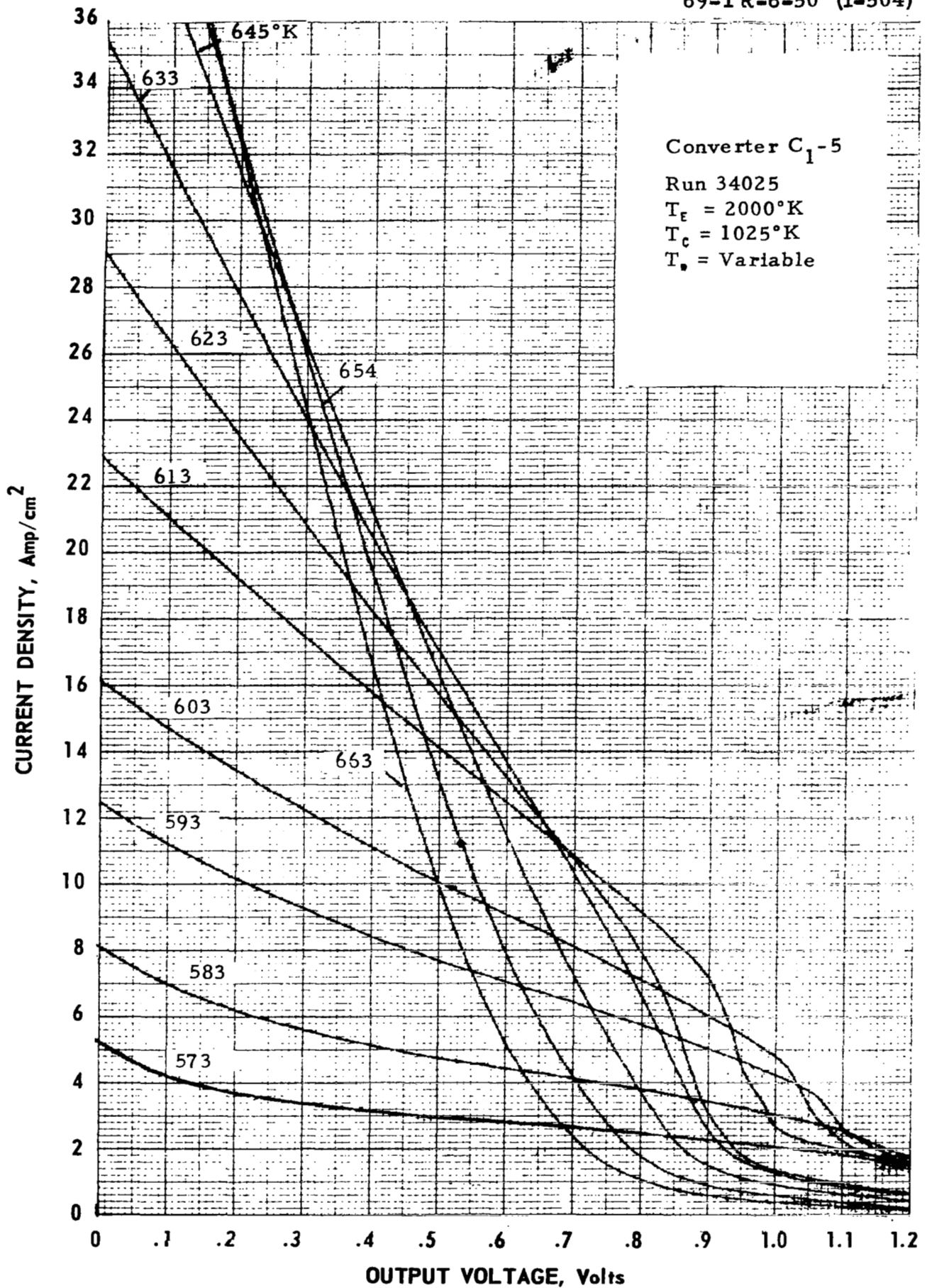
Figure C-10. Cesium Temperature Family of Converter C 1 -5 at T E = 2000°K.
