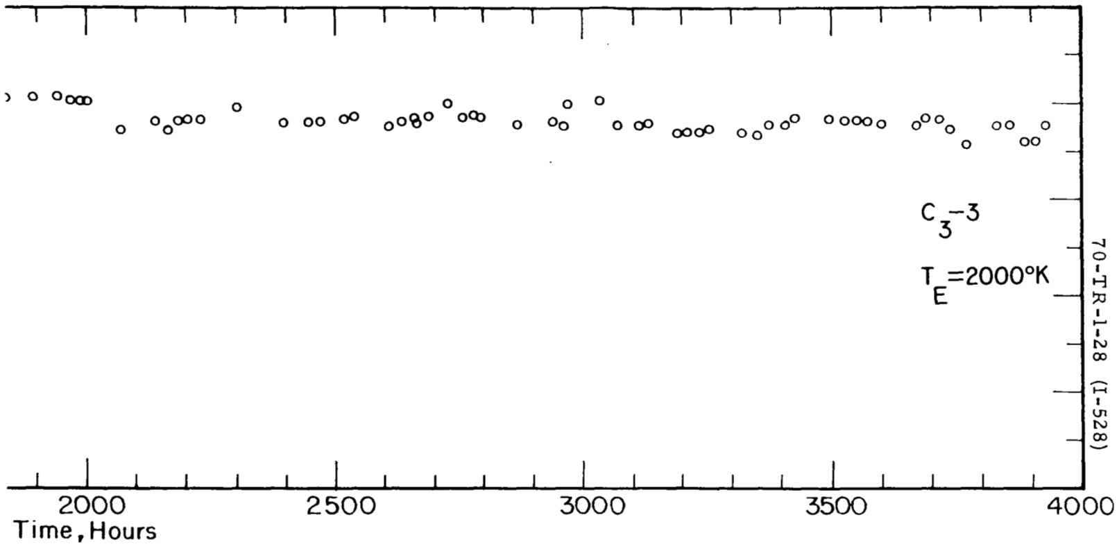
Data for Converter C_3-3 at T_E = 2000^\circ K .
