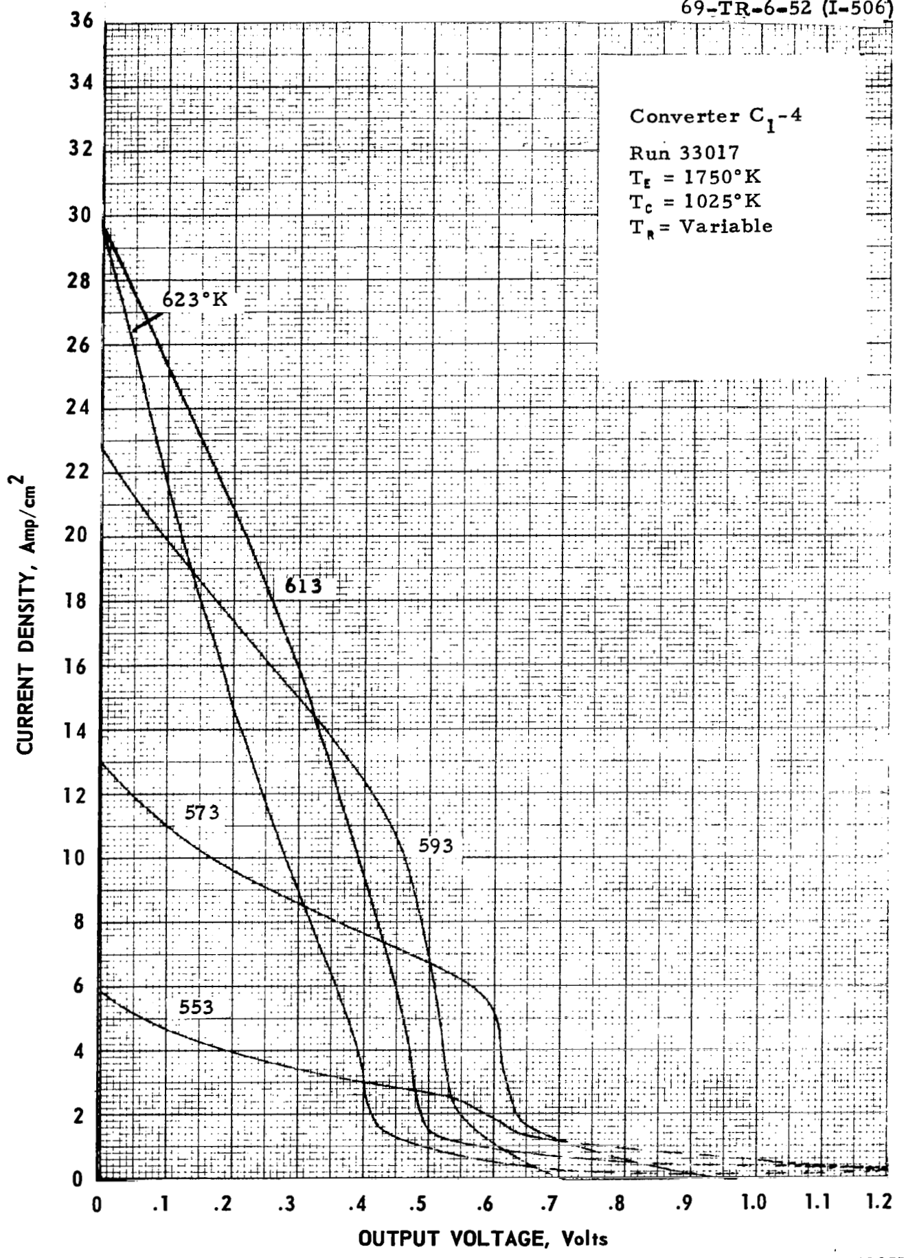
Figure C-12. Cesium Temperature Family of Converter C 1 -4 at T e = 1750°K. C-12
