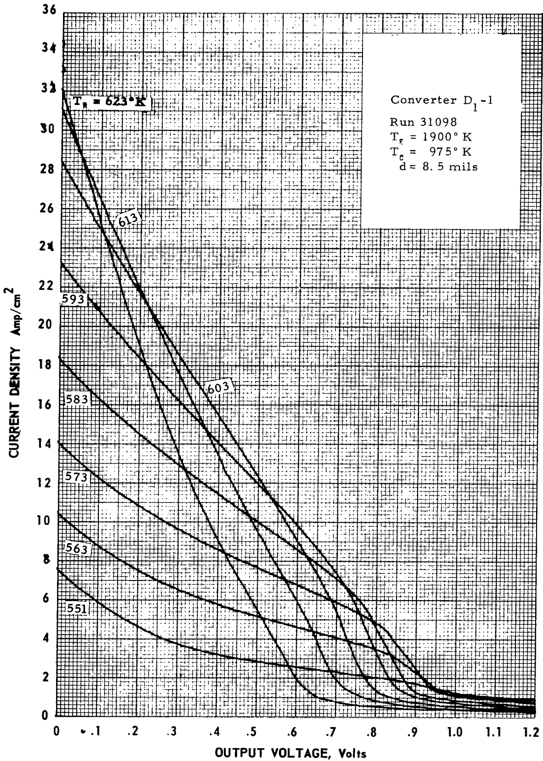
Figure B-30. Cesium-Temperature Family of Converter D_1-1 at T_g = 1900^\circ\text{K} .
