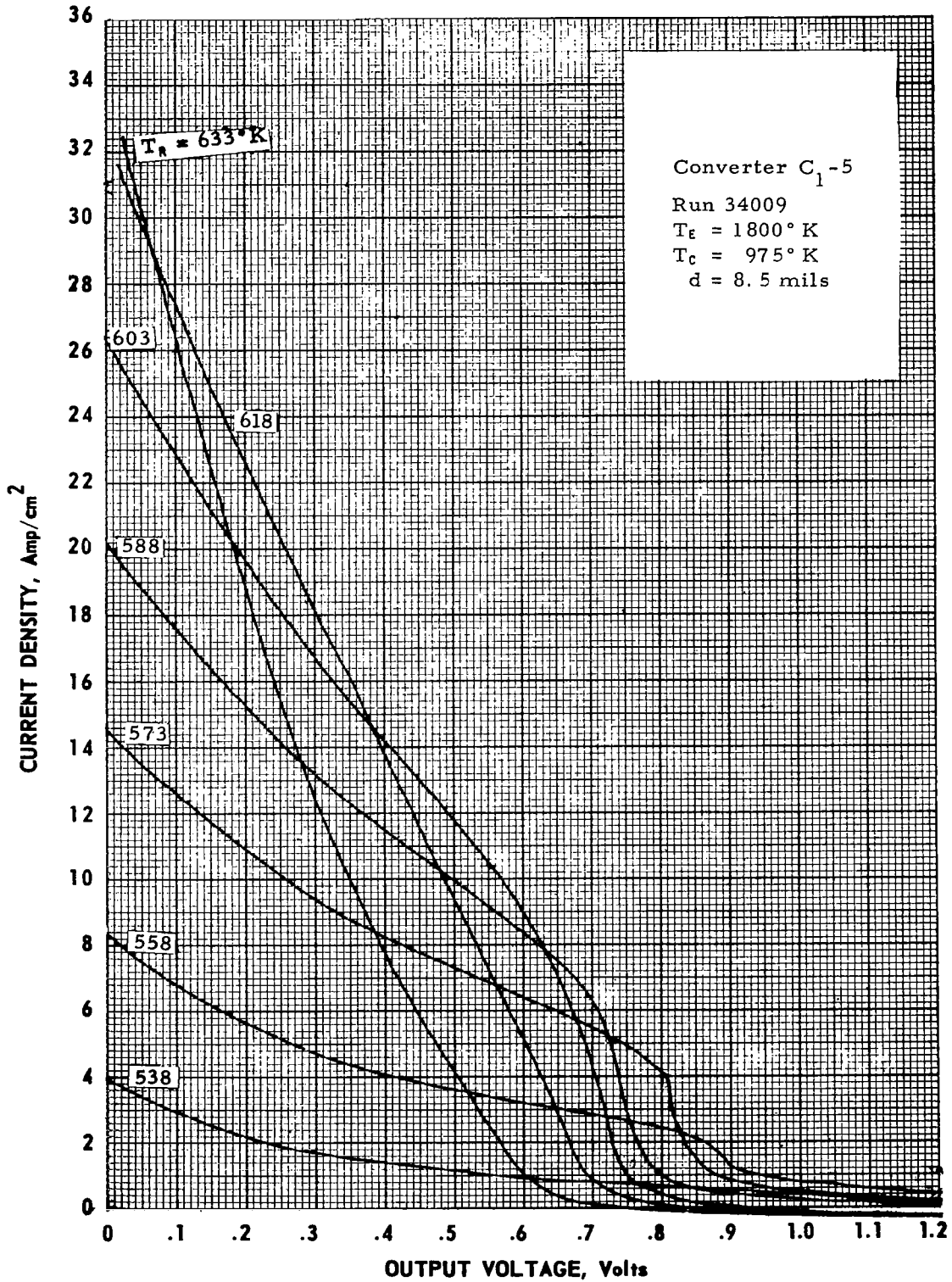
Figure B-19. Cesium-Temperature Family of Converter C 1 -5 at T E = 1800° K.
