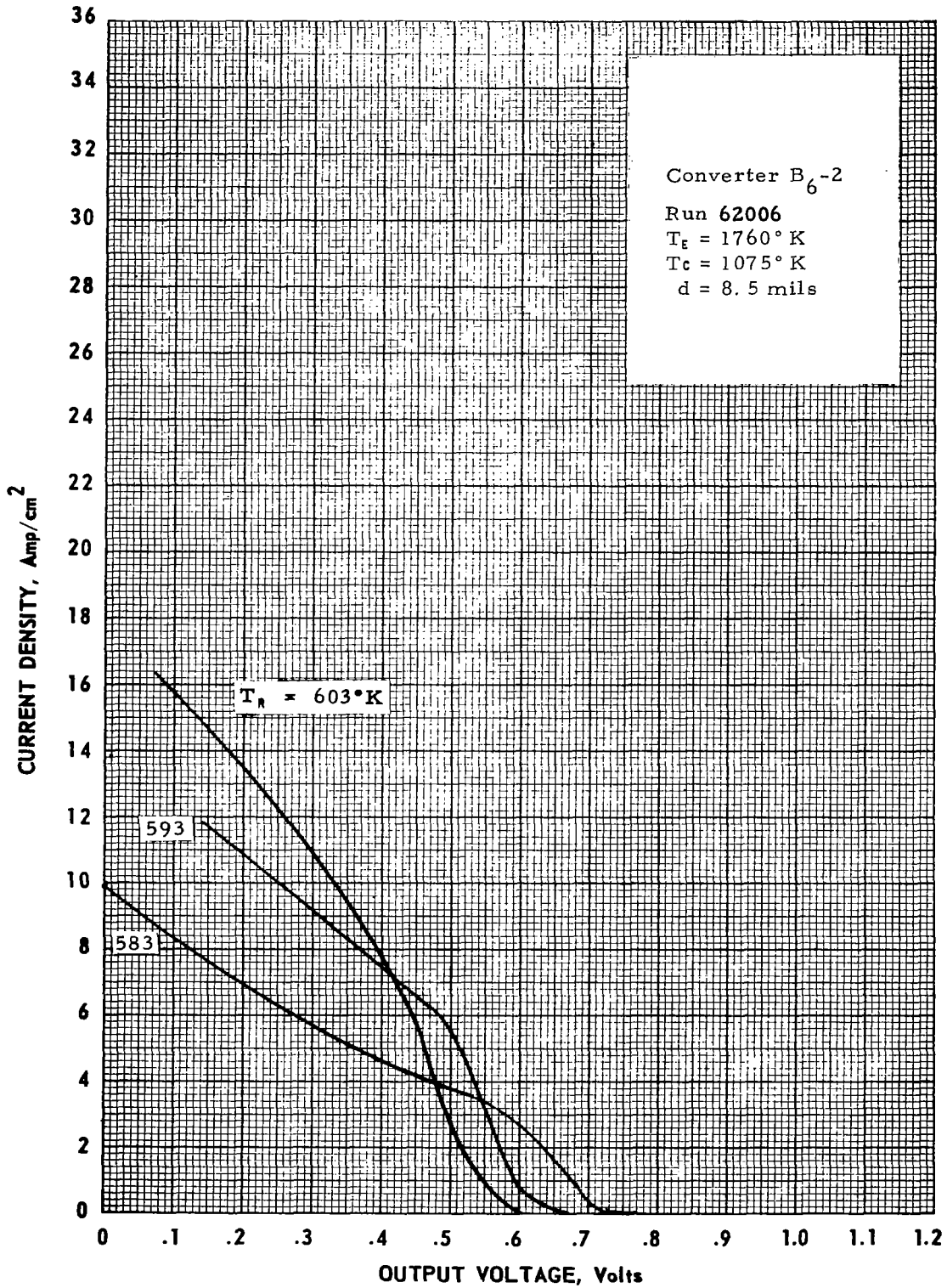
Figure B-7. Cesium-Temperature Family of Converter B 6 -2 at T E = 1760° K.
