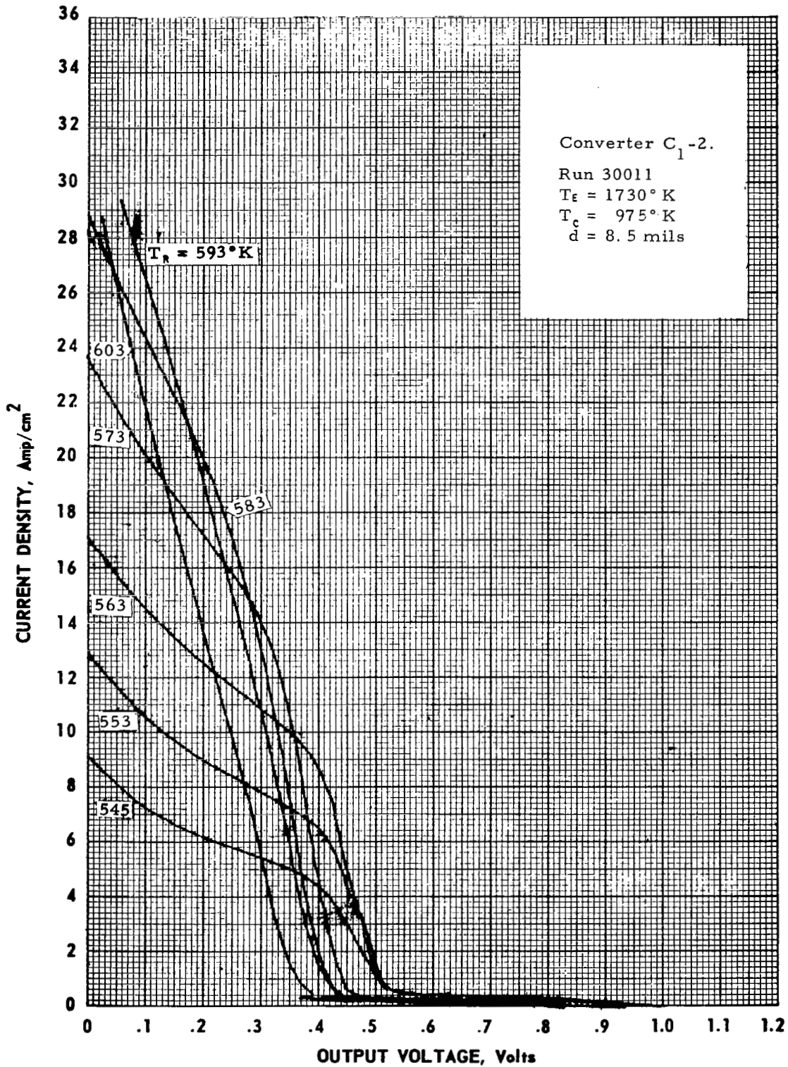
Figure B-9. Cesium-Temperature Family of Converter C 1 -2 at T E = 1730° K.
