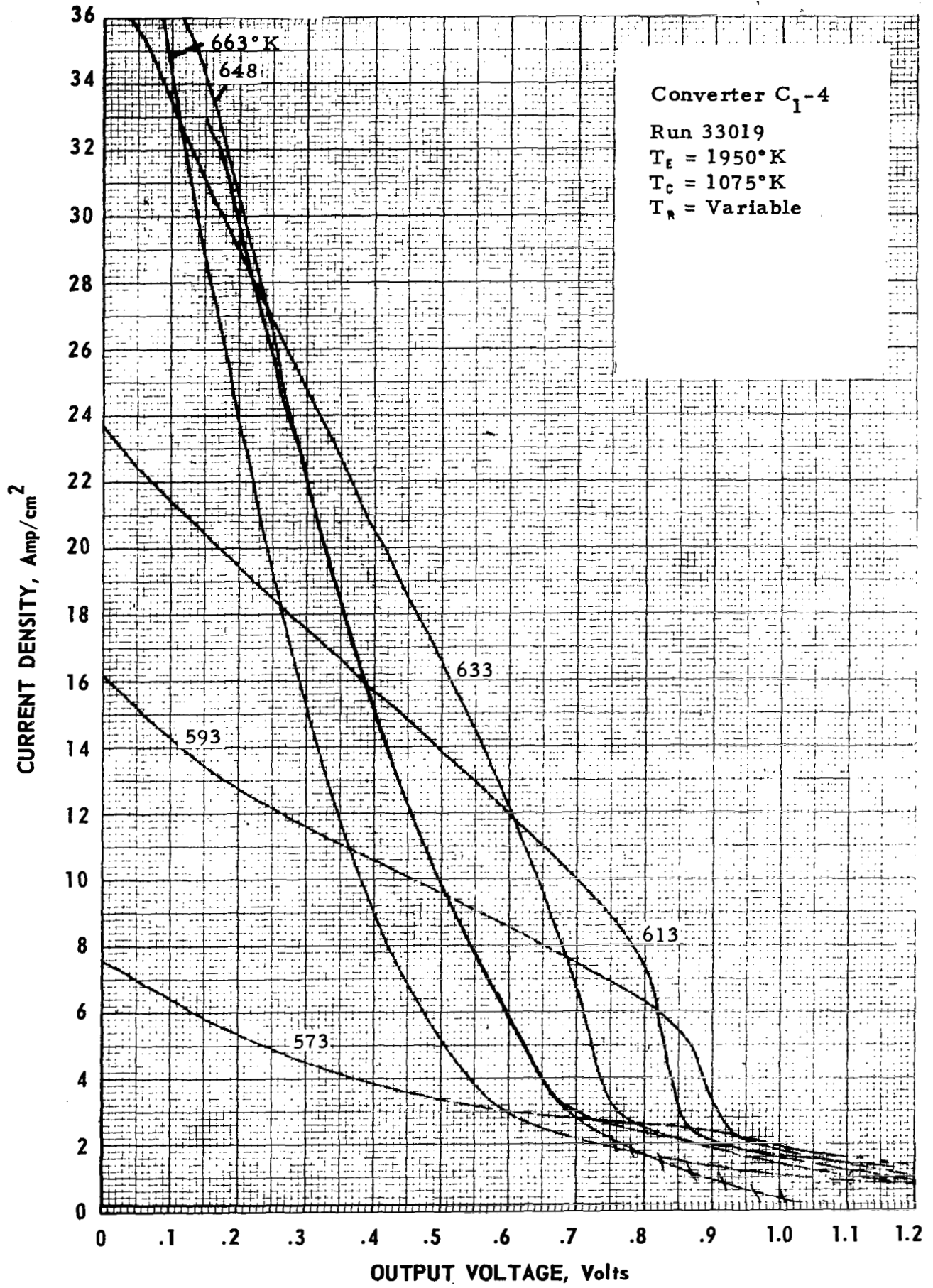
Figure C-14. Cesium Temperature Family of Converter C 1 -4 at T E = 1950°K.
