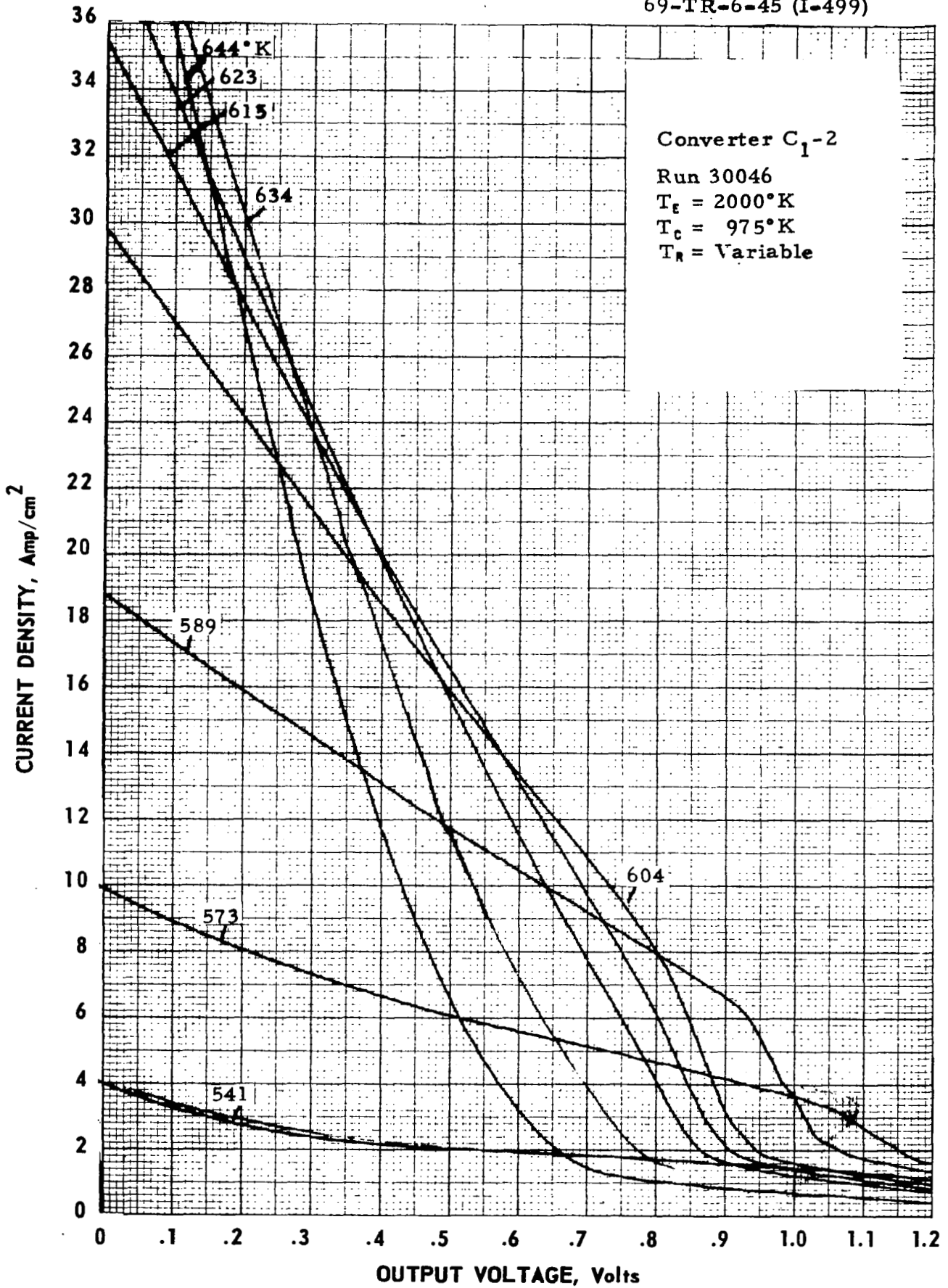
Figure C-5. Cesium Temperature Family of Converter C 1 -2 at T E = 2000°K.
