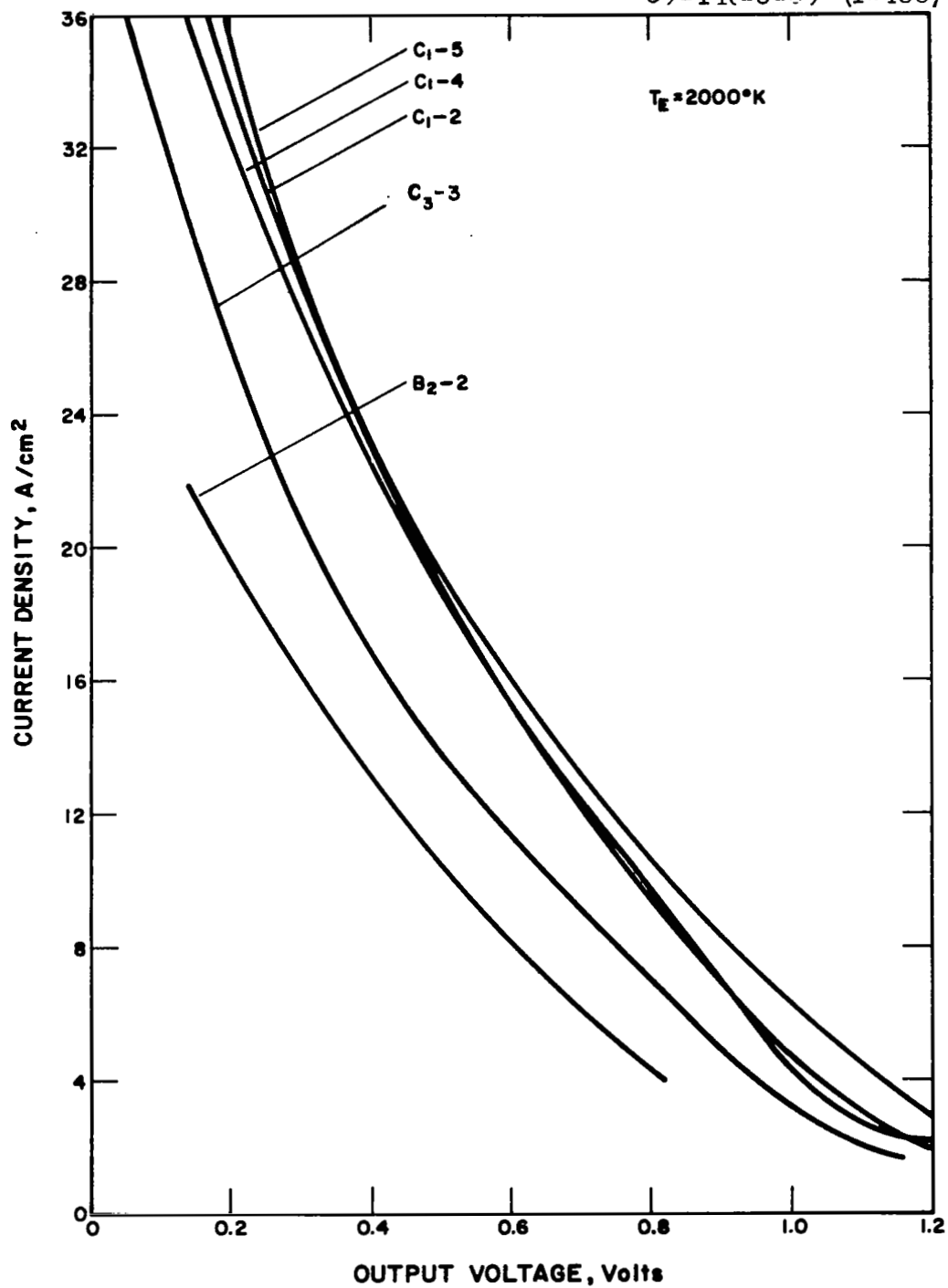
Figure VI-12. Comparison of Optimized Cesium-Temperature Envelopes at T_e = 2000^\circ\text{K} .
