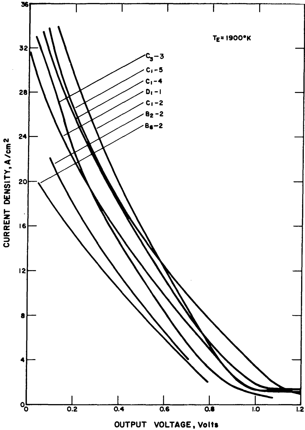
Figure VI-11. Comparison of Optimized Cesium-Temperature Envelopes at T E = 1900°K.
