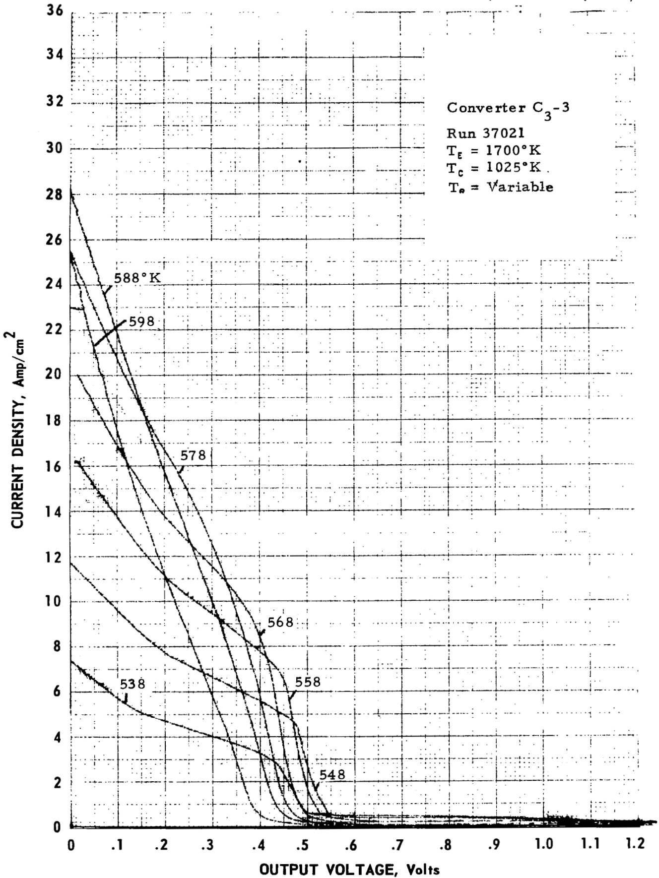
Figure B-23. Cesium Temperature Family of Converter C 3 -3 at T E = 1700°K. B-23
