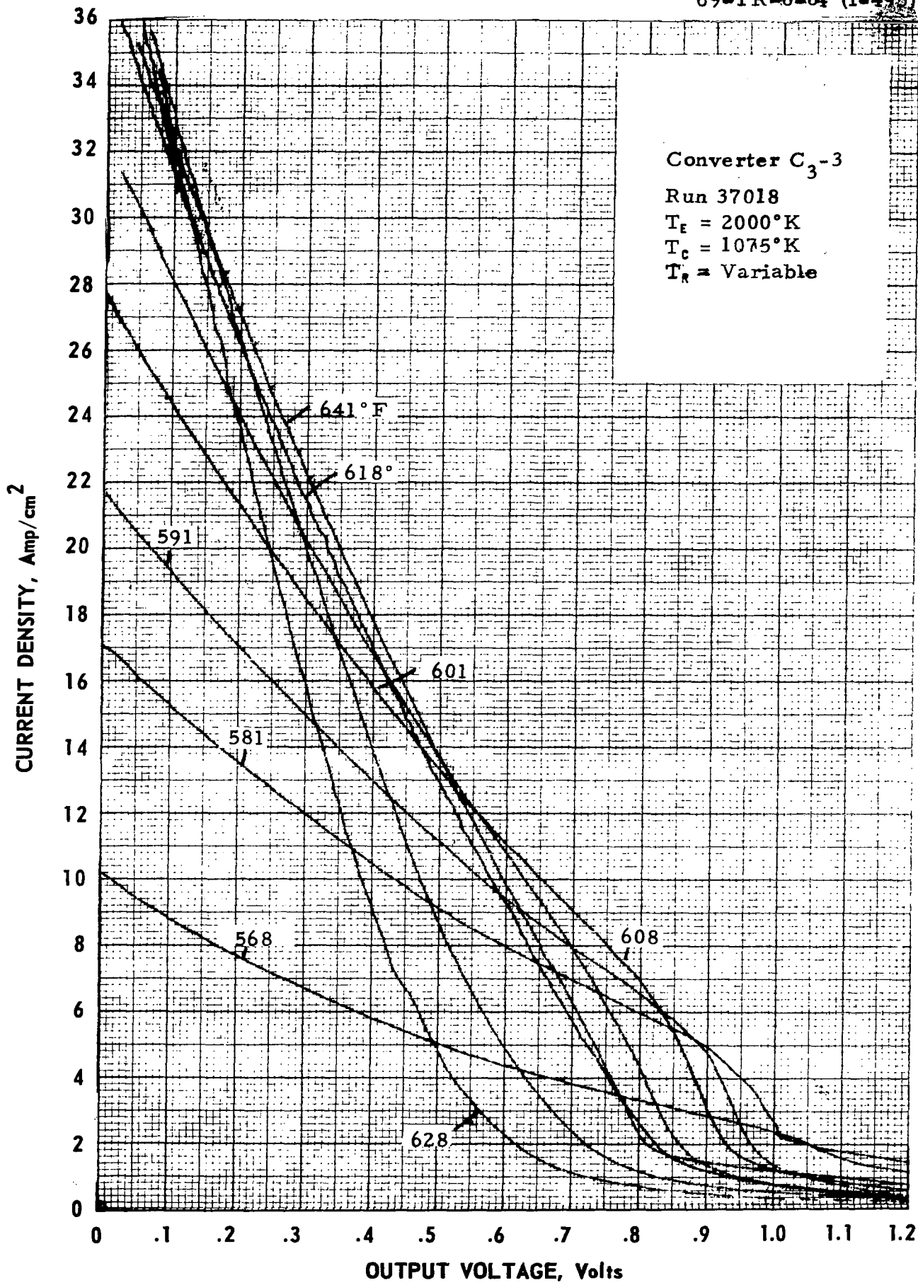
Figure B-26. Cesium Temperature Family of Converter C 3 -3 at T E = 2000°K.
