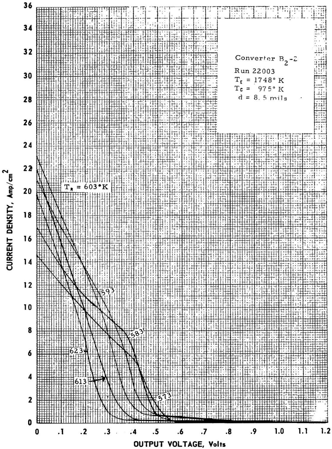
Figure B-1 Cesium-Temperature Family of Converter B 2 -2 at T E = 1748° K
