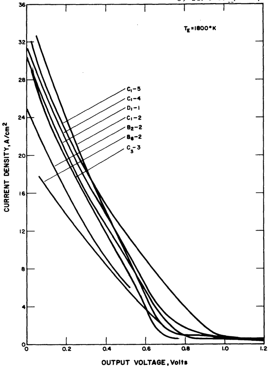
Figure VI-10 Comparison of Optimized Cesium-Temperature Envelopes at T_E = 1800^\circ\text{K} .
