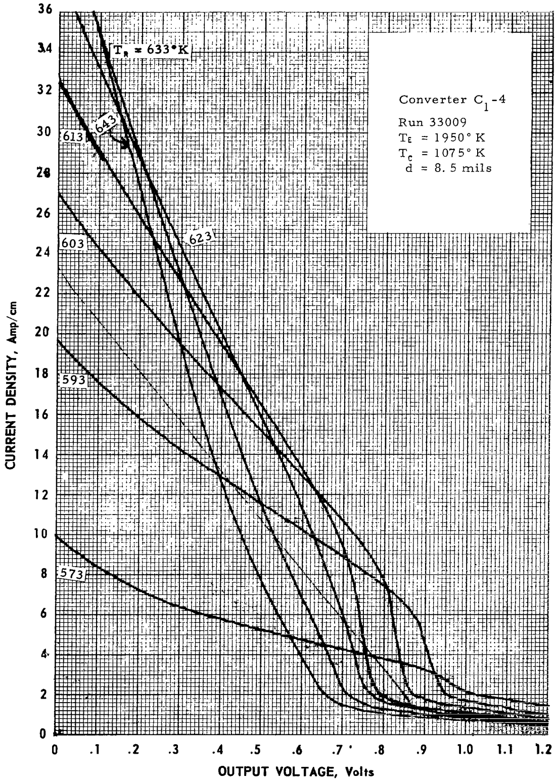
Figure B-16 Cesium-Temperature Family of Converter C 1 -4 at T E = 1950° K.
