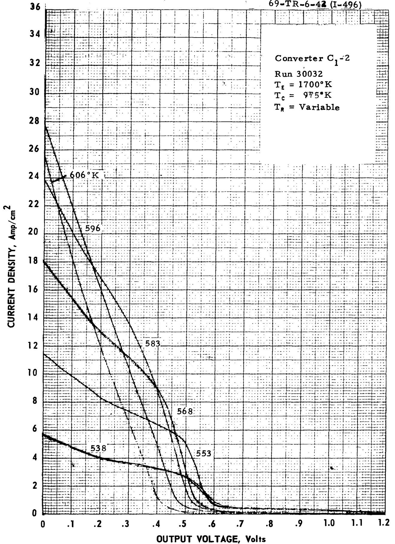
Figure C-2. Cesium Temperature Family of Converter C_1-2 at T_E = 1700^\circ\text{K} .
