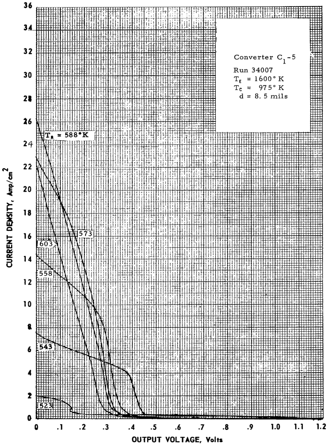
Figure B-17. Cesium-Temperature Family of Converter C 1 -5 at T E = 1600° K.
