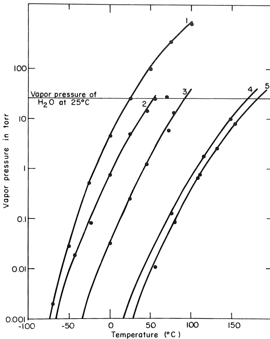
Figure 4. Points along curves 2, 3, 4, and 5 represent the measured vapor-pressure values for the Cartersville, Georgia, sample. Curve 2 was first measured, and subsequently the system was vacuum pumped for a number of hours. The resulting vapor-pressure curve is given by curve 3, reflecting a decrease in the sorbate volume. In a similar fashion, curves 4 and 5 were obtained. Curve 1 is the equilibrium vapor-pressure curve of liquid water and ice, at temperatures above and below 0°C, respectively. Curve 1 was measured with our apparatus and is in excellent agreement with standard, tabulated values.
