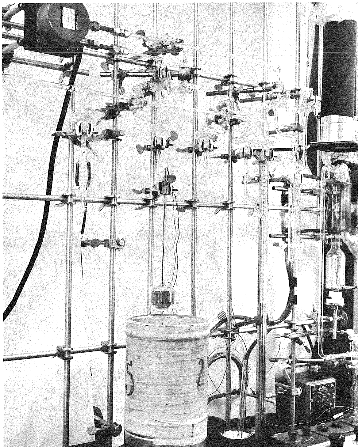
Figure 3. Photograph of the actual apparatus. Compare with the schematic diagram given in Figure 2.
