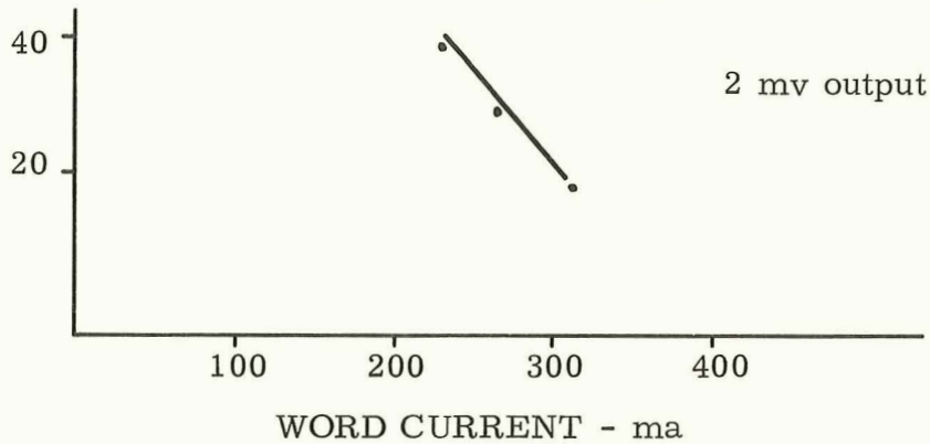
FIGURE 3-11. OPERATING POINTS FOR 2 MIL PLATED WIRE
