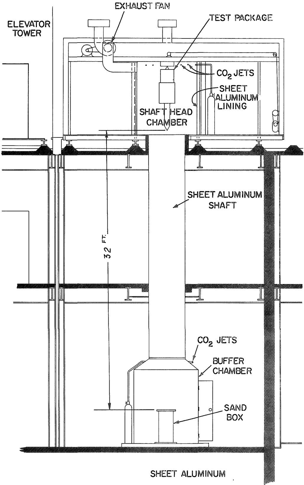
Figure 56. Drop tower—elevation.
