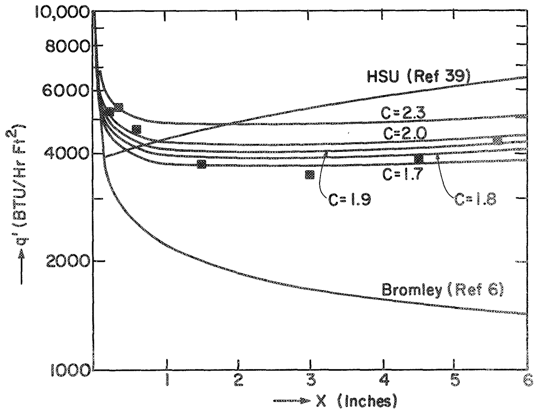
Figure 24. Effect of height on heat flux—film boiling. LH_2 . \Delta T = 100^\circ R .
