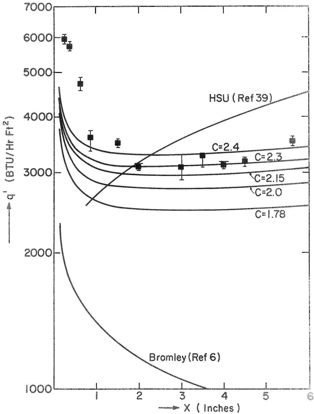
Figure 20. Effect of height on heat flux—film boiling. LN 2 . \Delta T = 100^\circ R .
