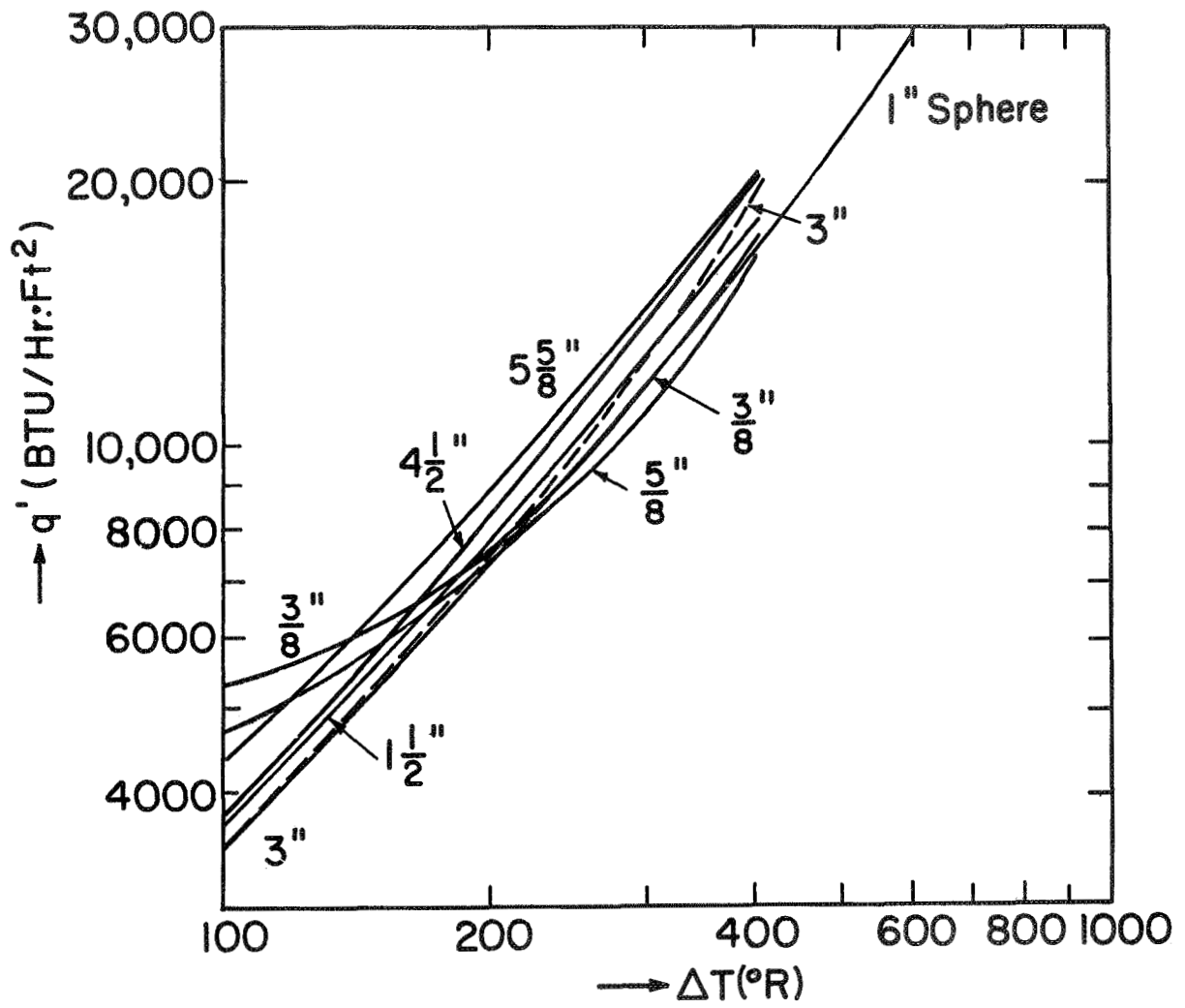
Figure 42. Effect of \Delta T on heat flux. LH 2 .
