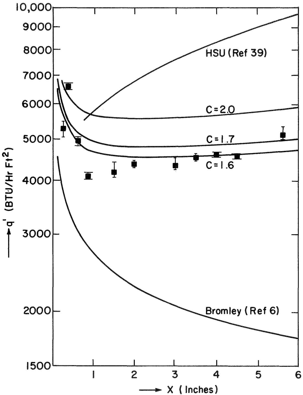
Figure 19. Effect of height on heat flux—film boiling. LN 2 . \Delta T = 204^\circ R .
