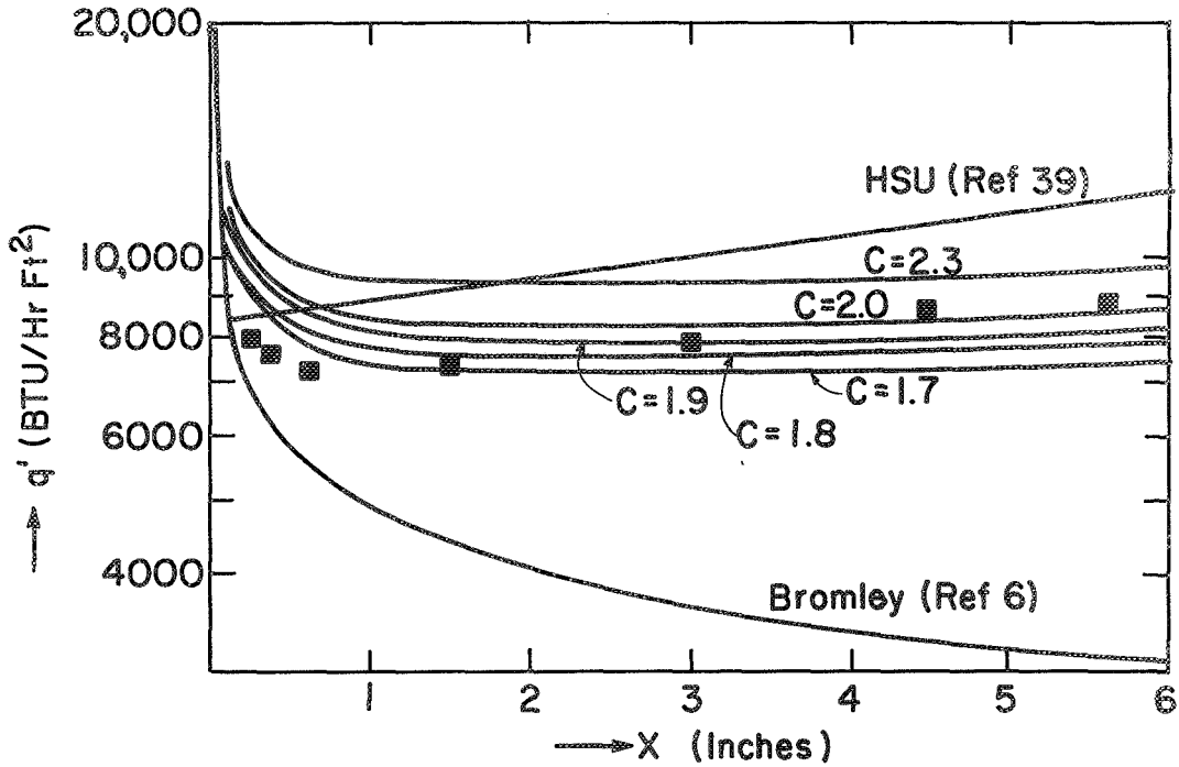
Figure 23. Effect of height on heat flux—film boiling. LH_2 . \Delta T = 200^\circ R .
