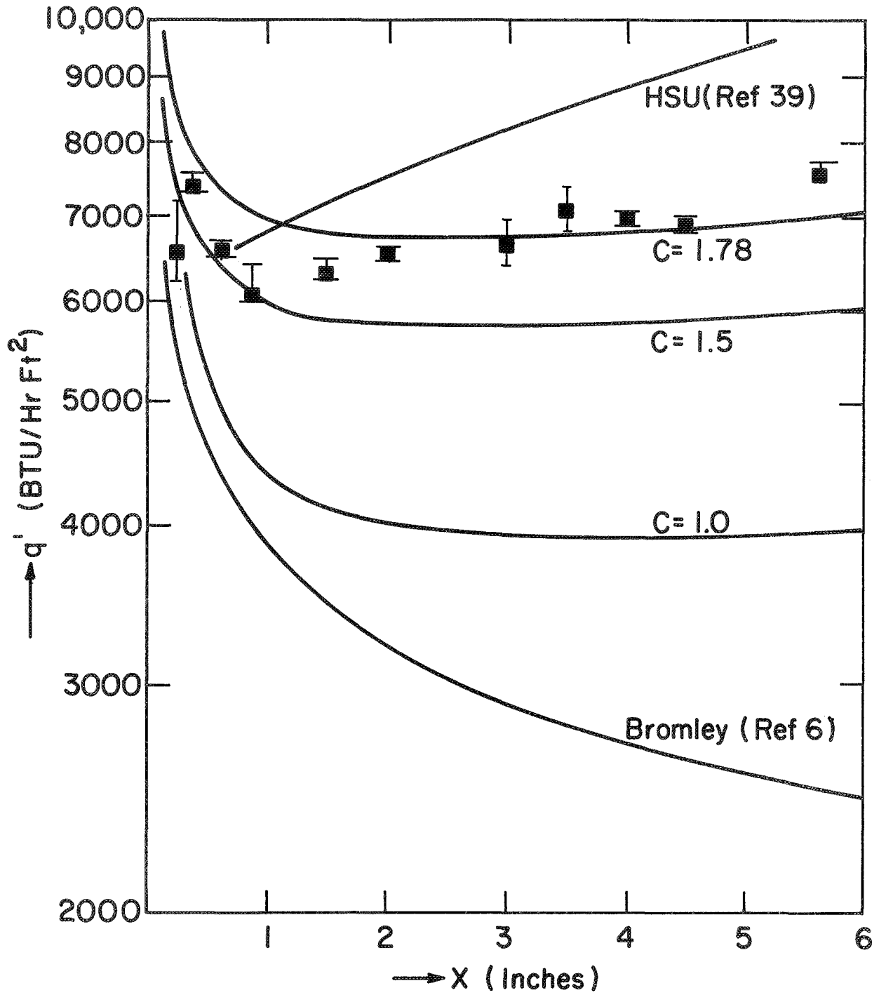
Figure 17. Effect of height on heat flux—film boiling. LN 2 . \Delta T = 315^\circ\text{R} .
