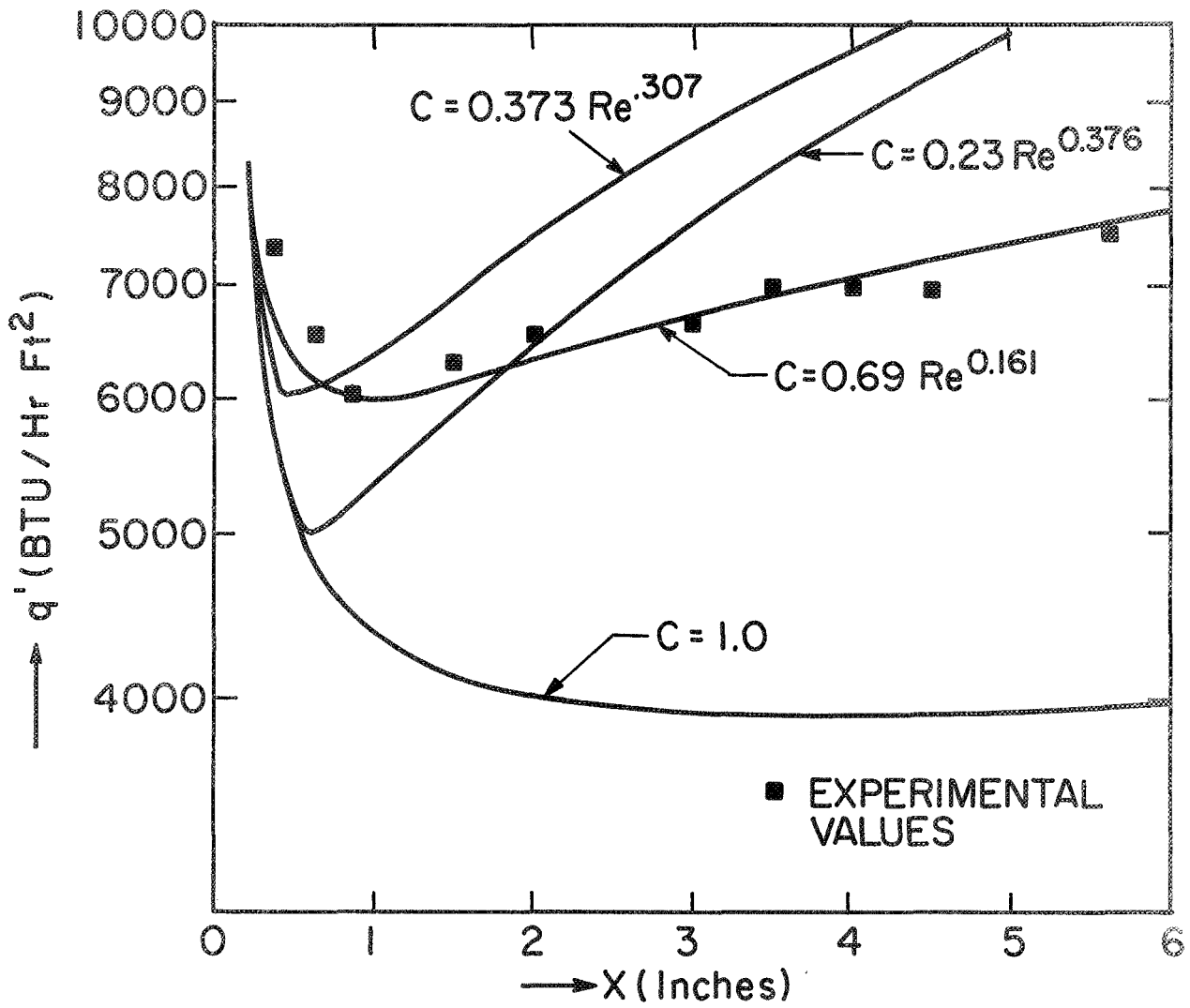
Figure 53. Effect of varying C with x . LN_2 . \Delta T = 315^\circ R .
