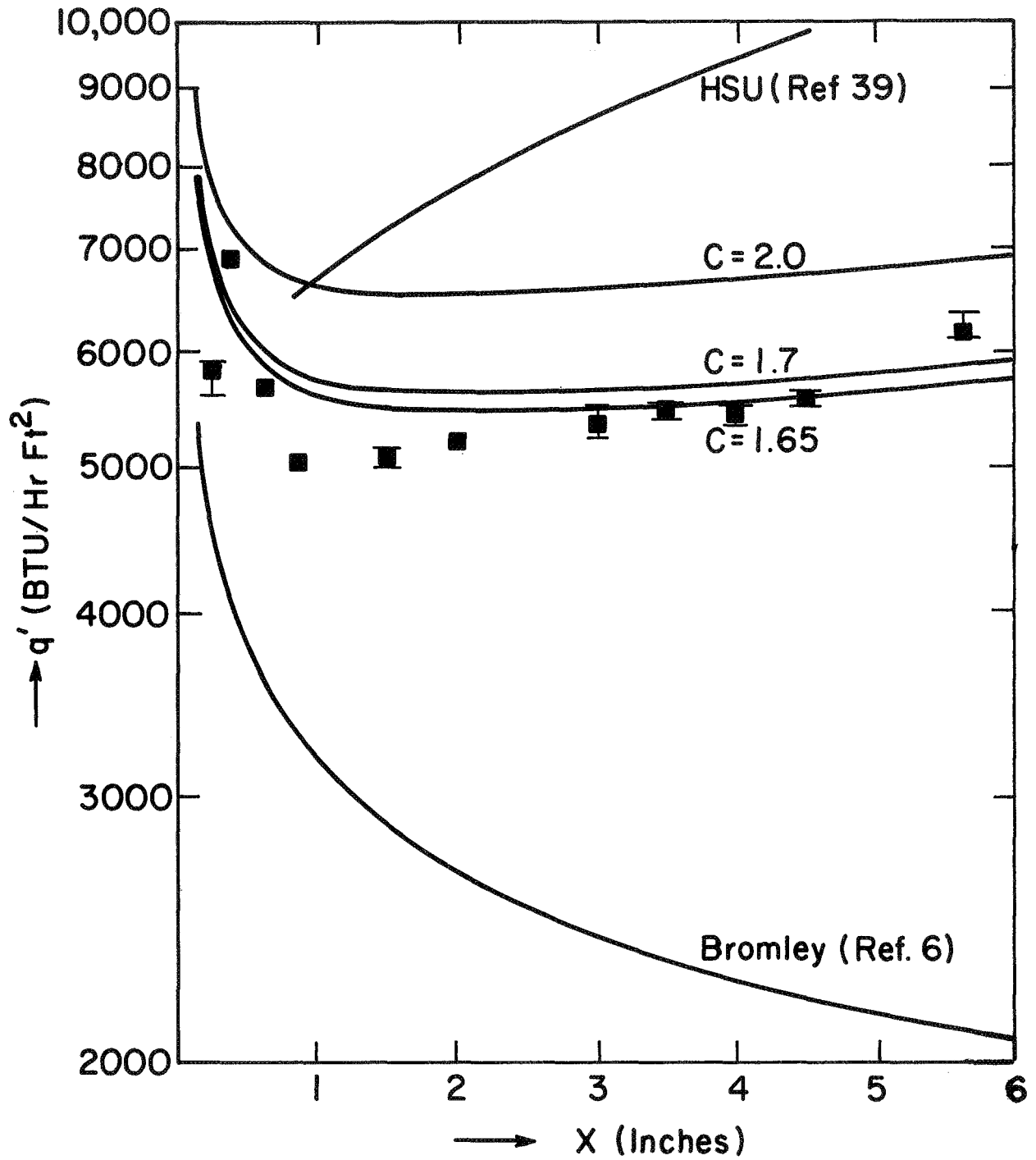
Figure 18. Effect of height on heat flux—film boiling. LN 2 . \Delta T = 251^\circ\text{R} .
