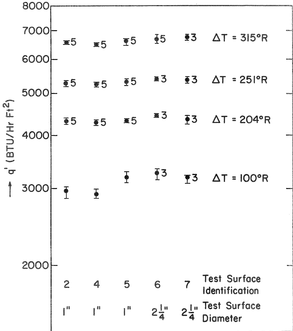
Figure 16. Comparison of heat flux—1 in. dia and 2-1/4 in. dia heating surfaces.
