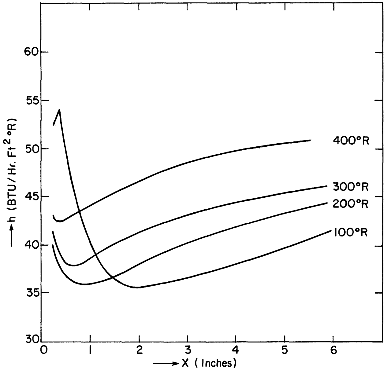
Figure 40. Effect of height on heat transfer coefficient. LH 2 .
