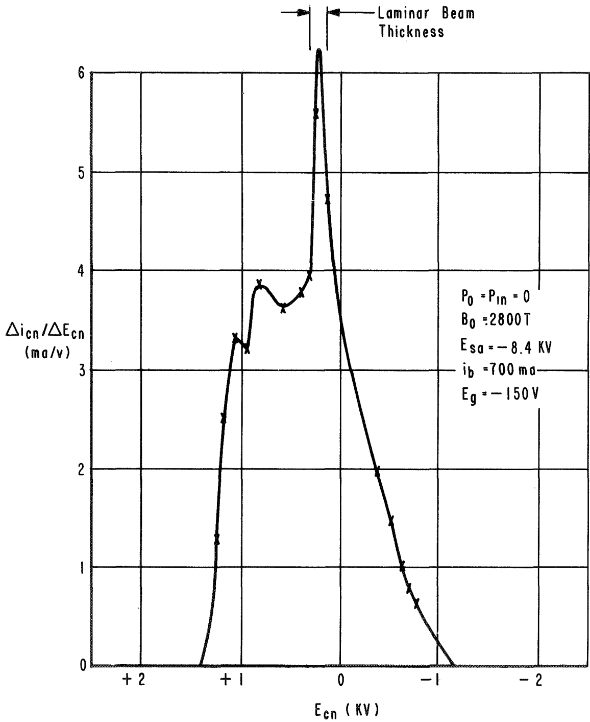
Exp. No. 2A016114 - Beam Potential Profile D283
