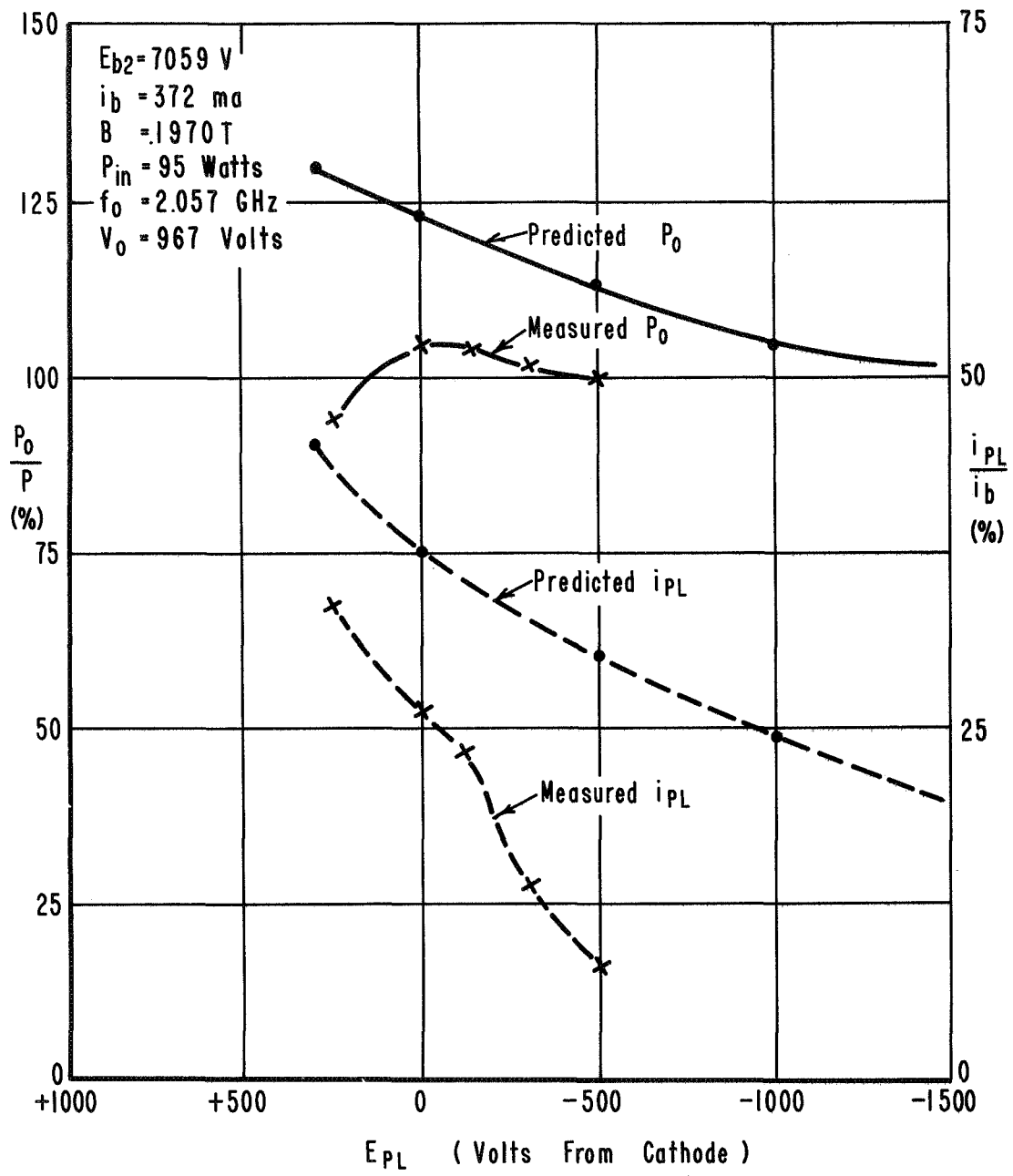
Normalized Output Power And Potential Limiting Current VS. Potential Limiting Voltage. D263
