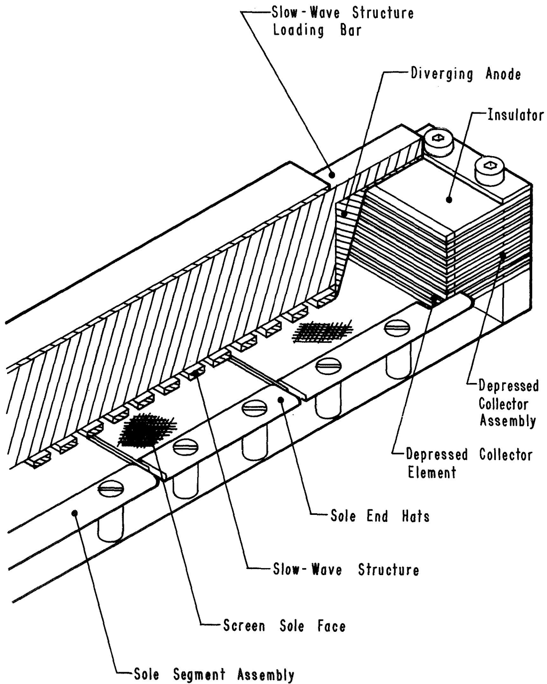
Experimental Amplifier
