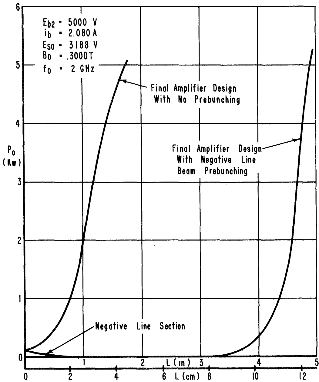
Negative Line Beam Prebunching Output Power VS. Interaction Length. D258
