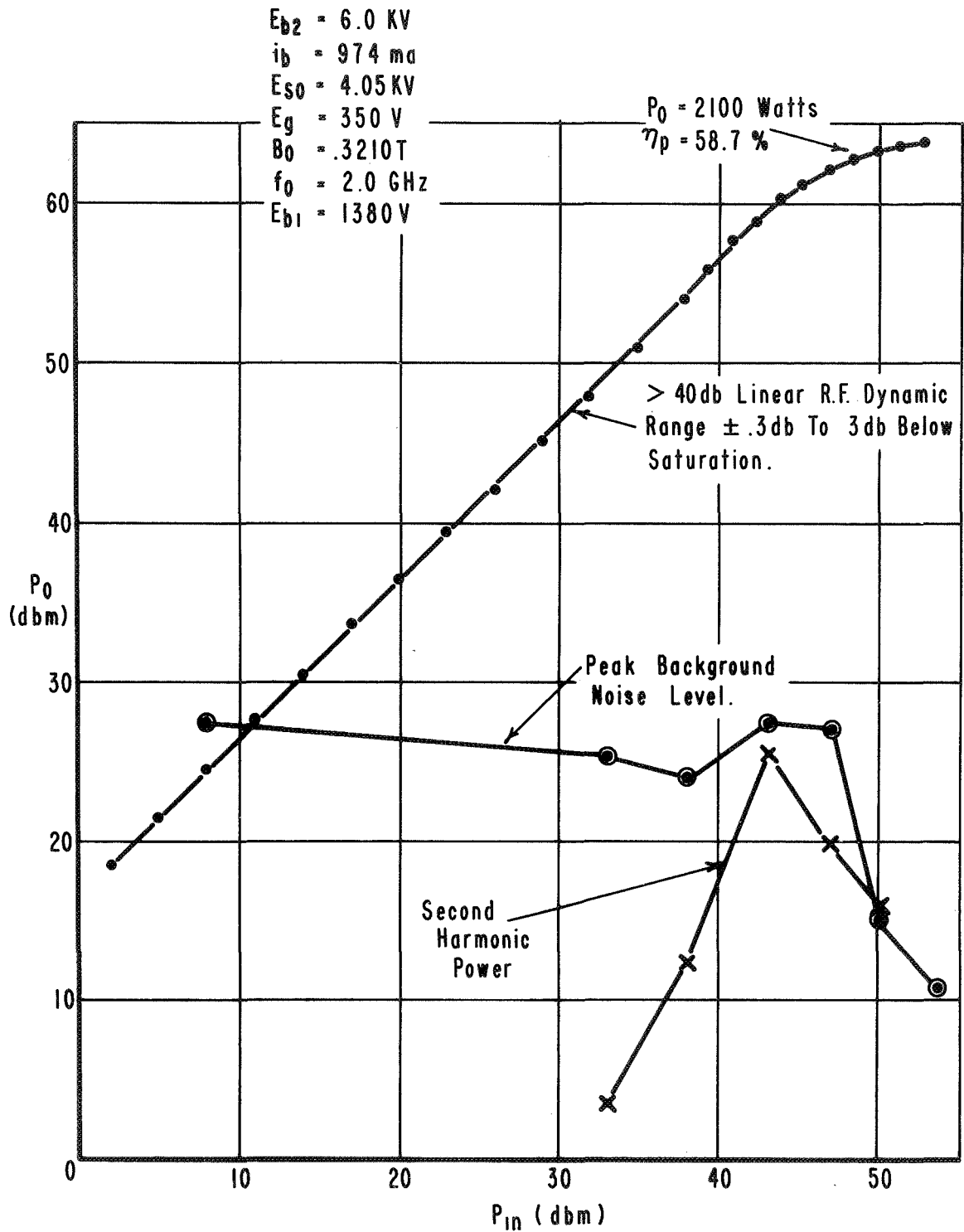
Exp. No. 2A016114 - RF Dynamic Range
