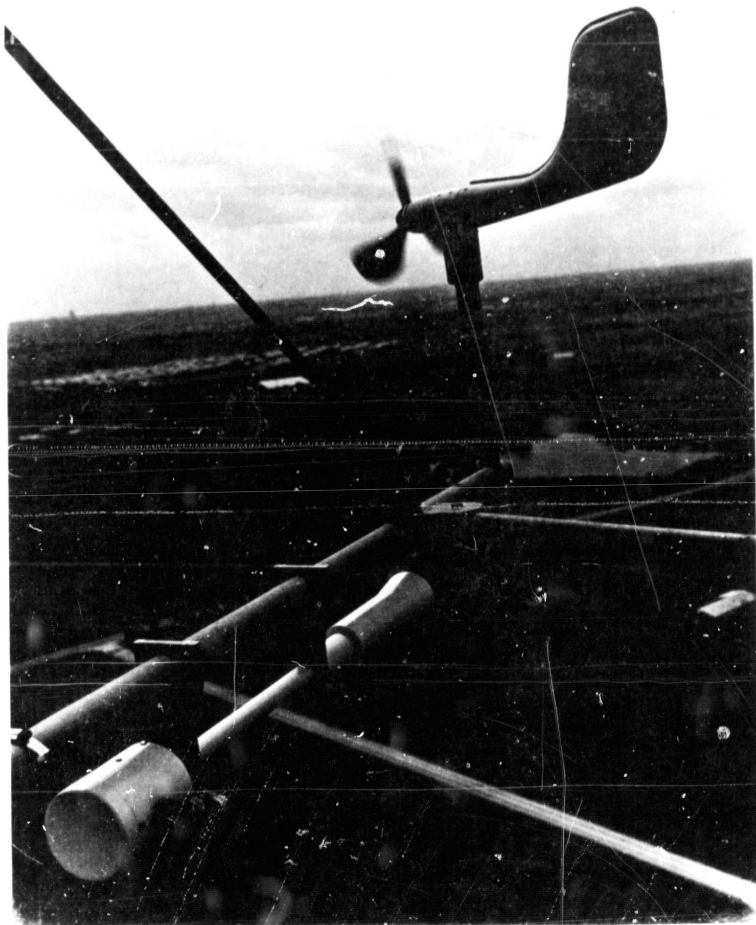
Figure 6. Aerovane wind transmitter and Climet aspirated radiation shield containing thermistor temperature sensor, mounted on tower instrument boom. View to southwest.
