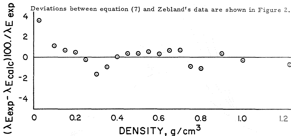
Figure 2. Deviation between thermal conductivity for O 2 from equation (7) and Ziebland and Burton (1955).
