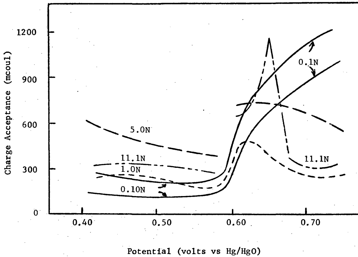
Fig. 24--Charge acceptance vs applied potential for potentiostatic oxidations at 0° C.
