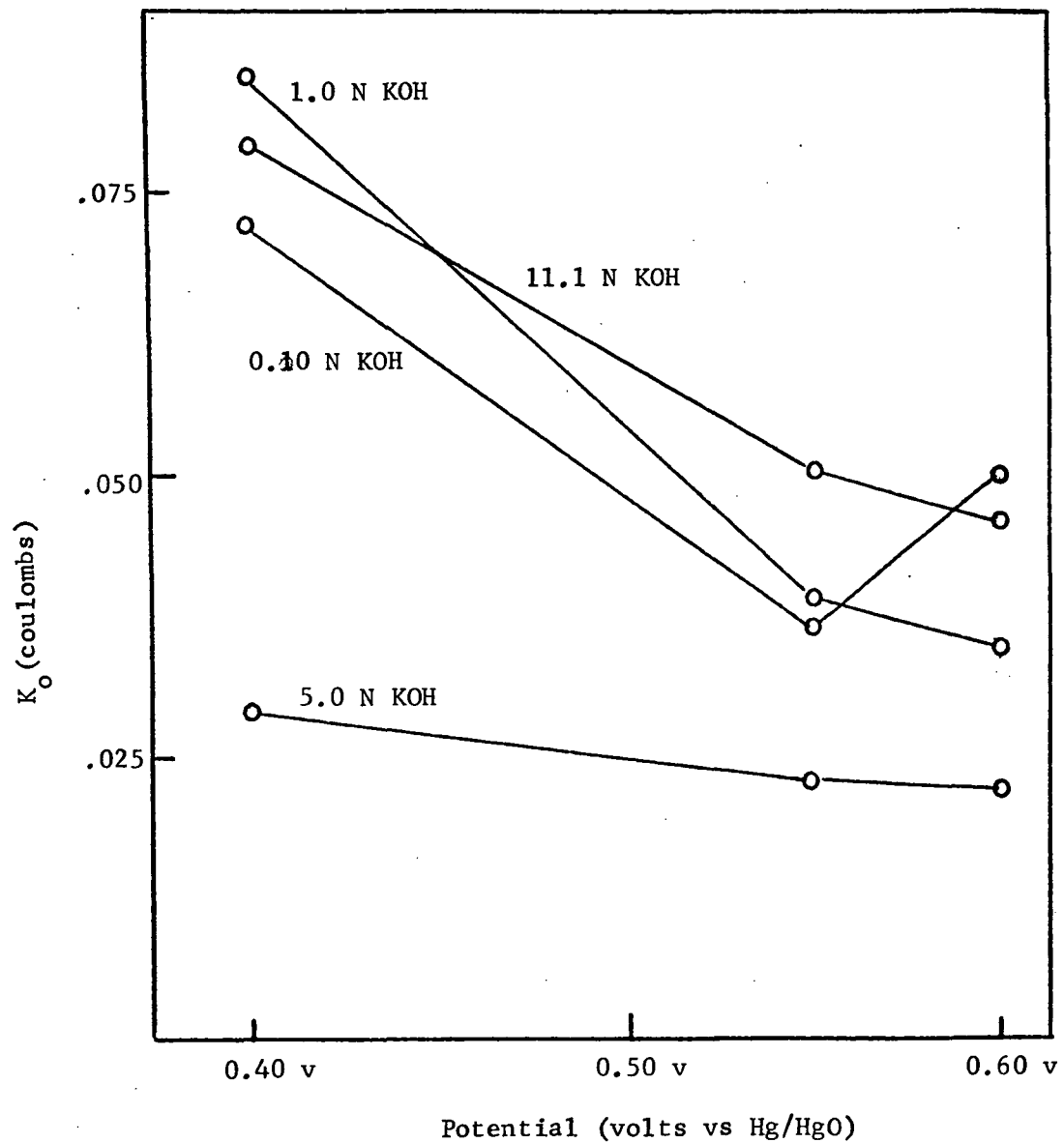
Fig. 31-- Plot of K_0 vs applied potential for oxidations in various hydroxide ion concentrations at 25°C.
