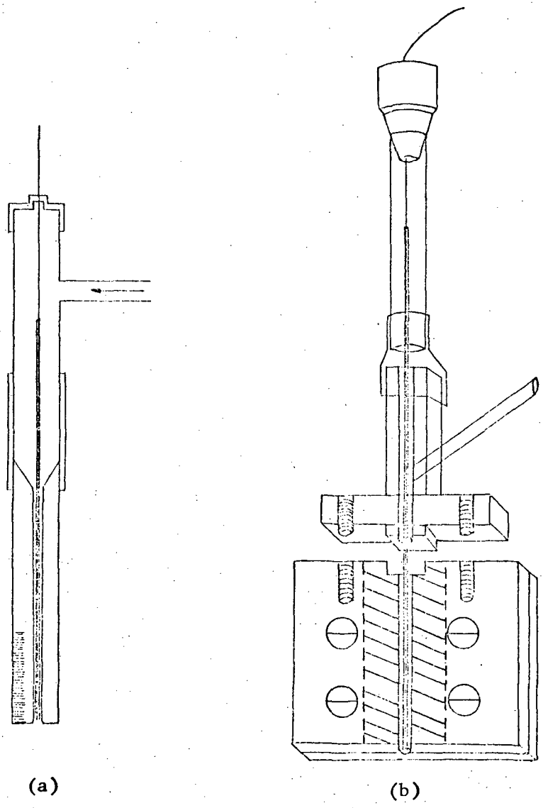
Figure 17. Model-pore electrodes
