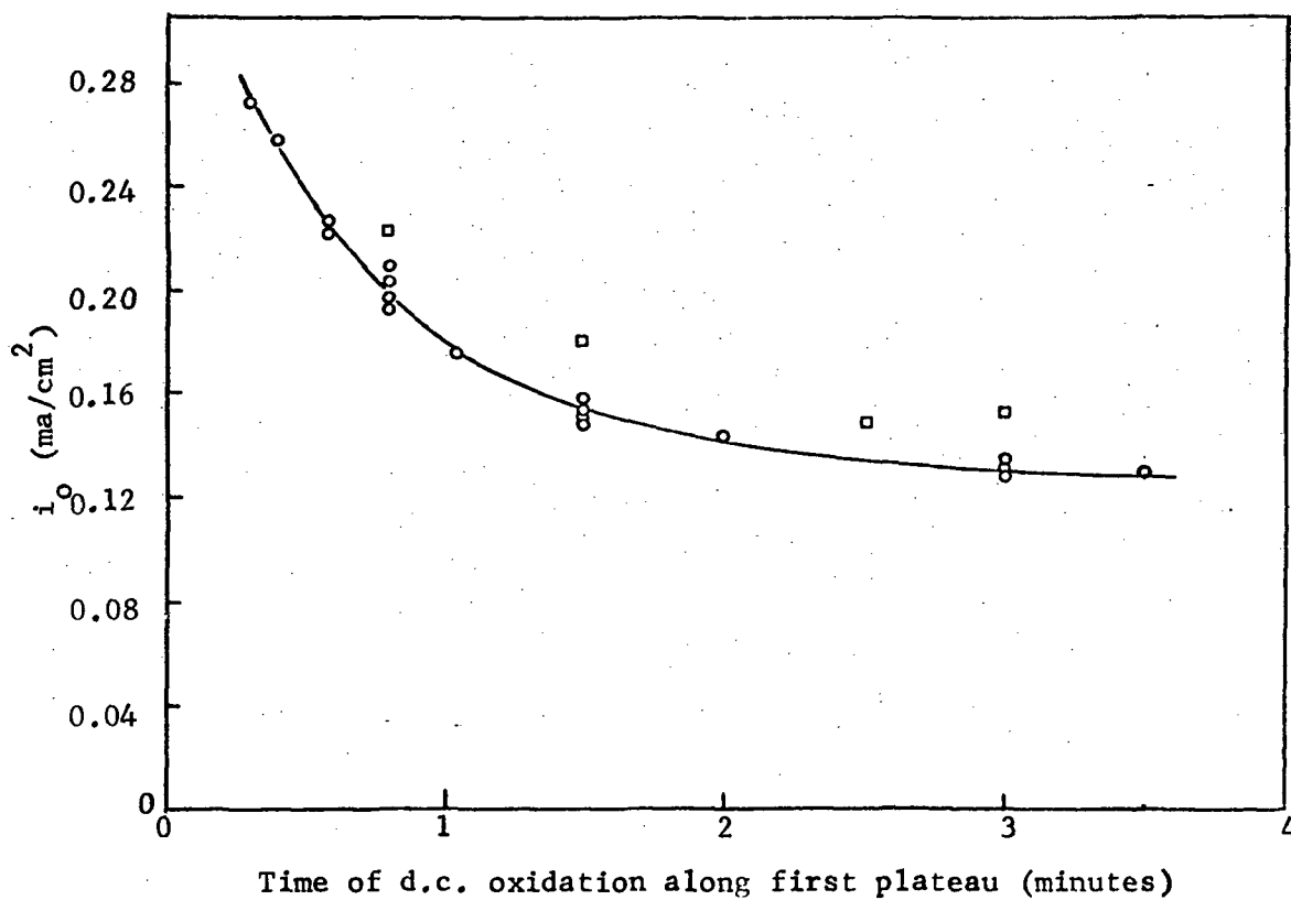
Fig. 10--Plot of i versus time of oxidation along first plateau. Square wave current density 0.412 \text{ ma/cm}^2 . Total first plateau length 4.0 minutes. \square = points calculated from c.c.s. measurements taken before oscilloscope trace had stabilized. \circ = points calculated after stabilization.
