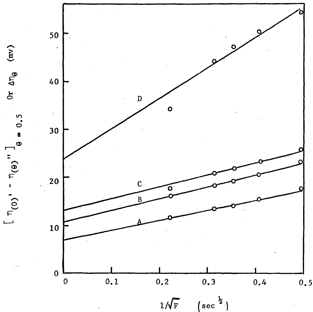
Fig. 3--Determination of i_0 at \theta = 0.5 for the \text{Ag-Ag}(\text{NH}_3)_2^+ System. Concentration of ammonia: 14.7 M. Current density i_A = 3.14 \times 10^{-4} amp/cm 2 . Concentration of \text{Ag}(\text{NH}_3)_2^+ ( C_{\text{ox}^0} ) A- 2.5 \times 10^{-1} M; B- 2.5 \times 10^{-2} M; C- 2.5 \times 10^{-3} M; D- 2.5 \times 10^{-4} M. Calculated i_0 values: A- 1.17 ma/cm 2 ; B- 0.73; C- 0.63; D- 0.34.
