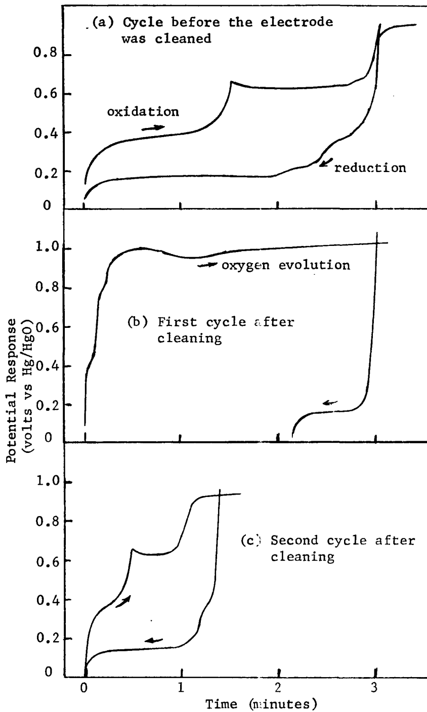
Figure 45 Galvanostatic Oxidation of a Silver Wire Electrode at 0^{\circ}\text{C} . Saturated with \text{O}_2 and \text{Ag}_2\text{O} Electrolyte Concentration 0.10\text{ N KOH} Current Density 1.8\text{ ma/cm}^2
