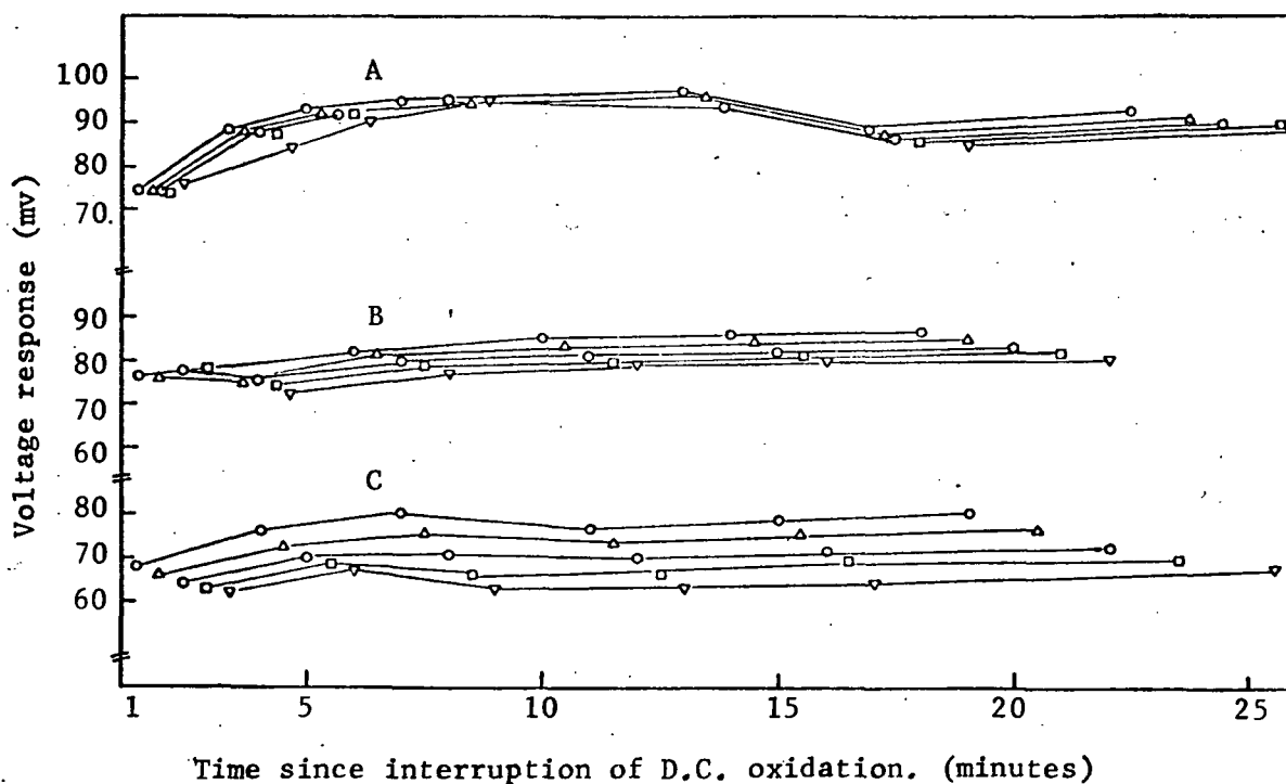
Fig. 12--Plot of electrode voltage response versus time since interruption of d.c. oxidation for five different frequencies.
