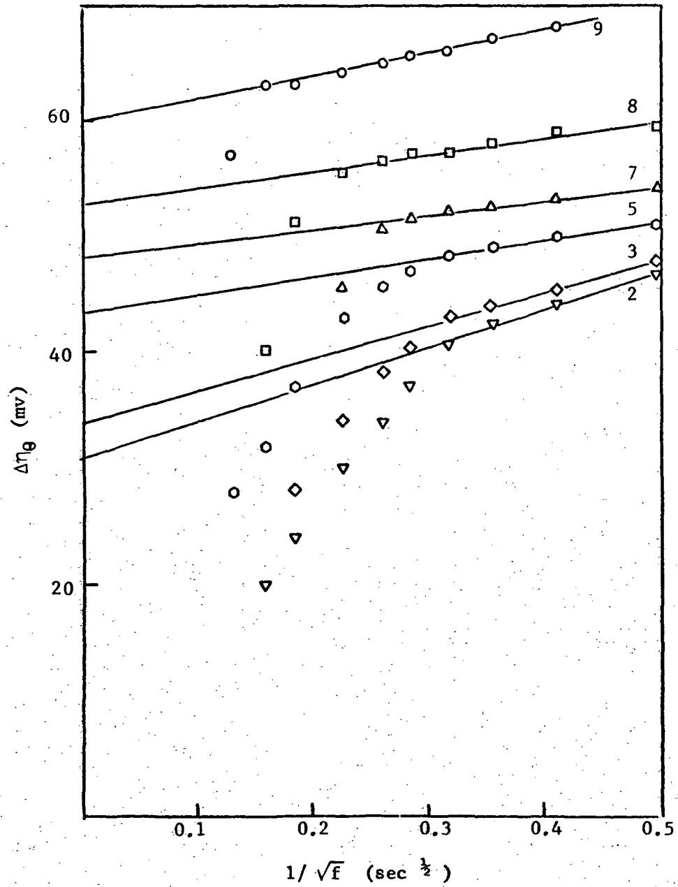
Fig. 8--Typical plots of c.c.s. measurements on the Ag-Ag 2 O system. The run numbers correspond to numbers given in Figure 9.
