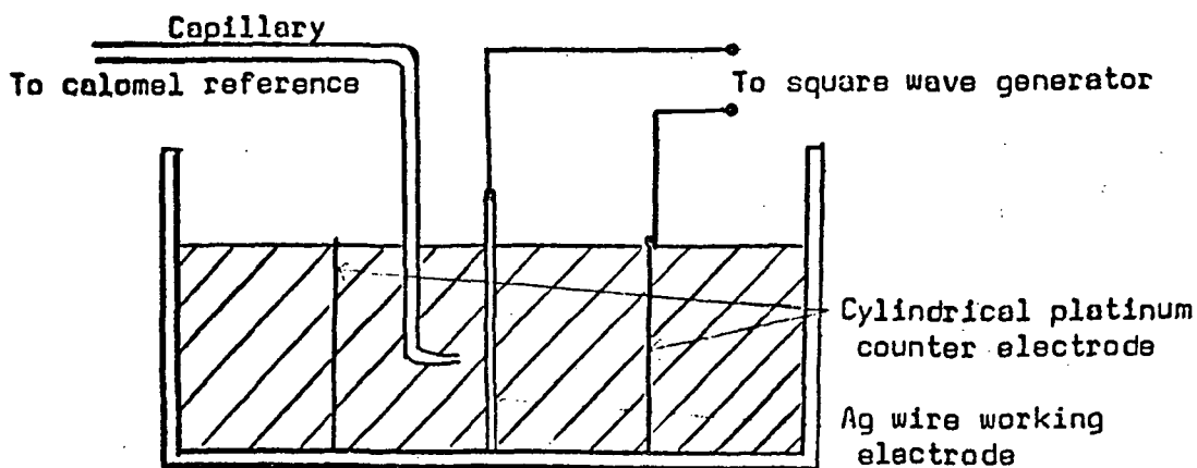
Fig. 1 ---Modified c.c.s. apparatus. a) circuit diagram b) cell diagram.
