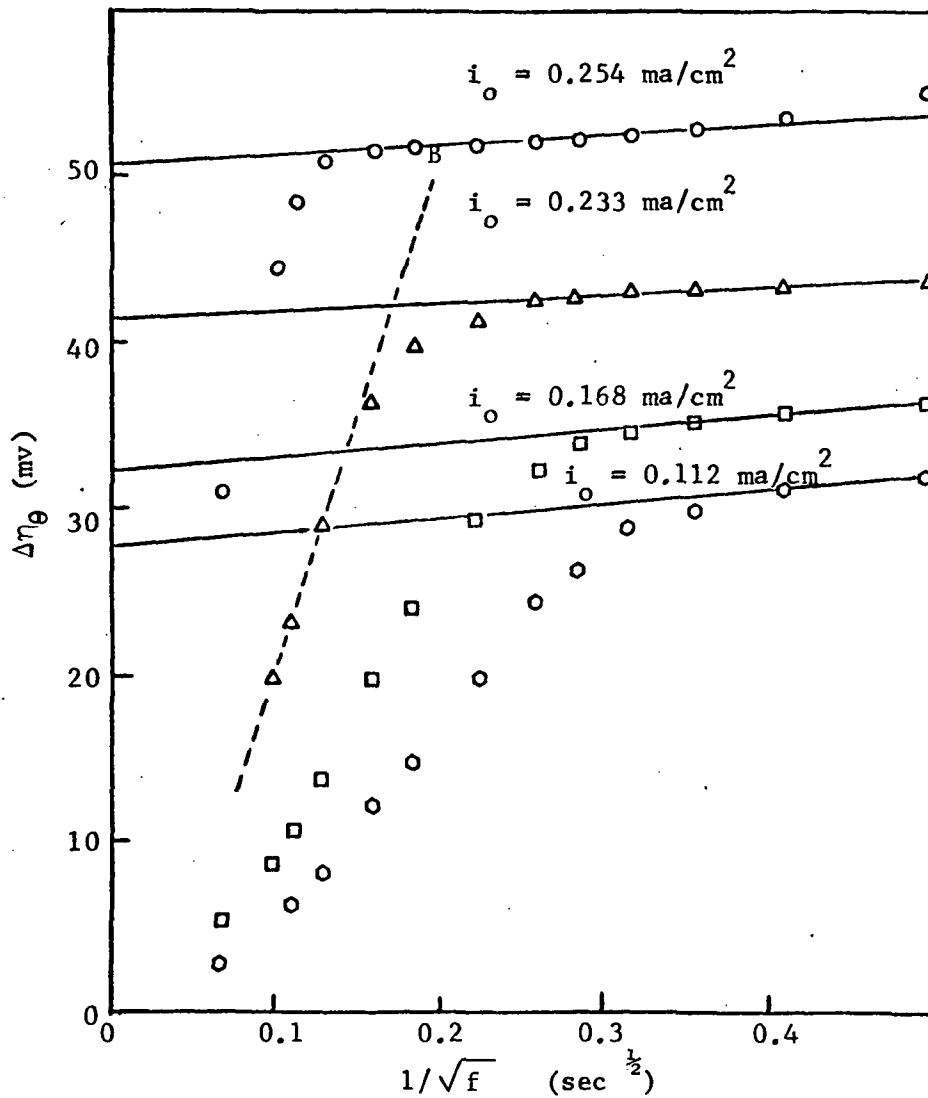
Fig. 6--C.C.S. Measurements of the \text{Ag-Ag}(\text{NH}_3)_2^+ System
