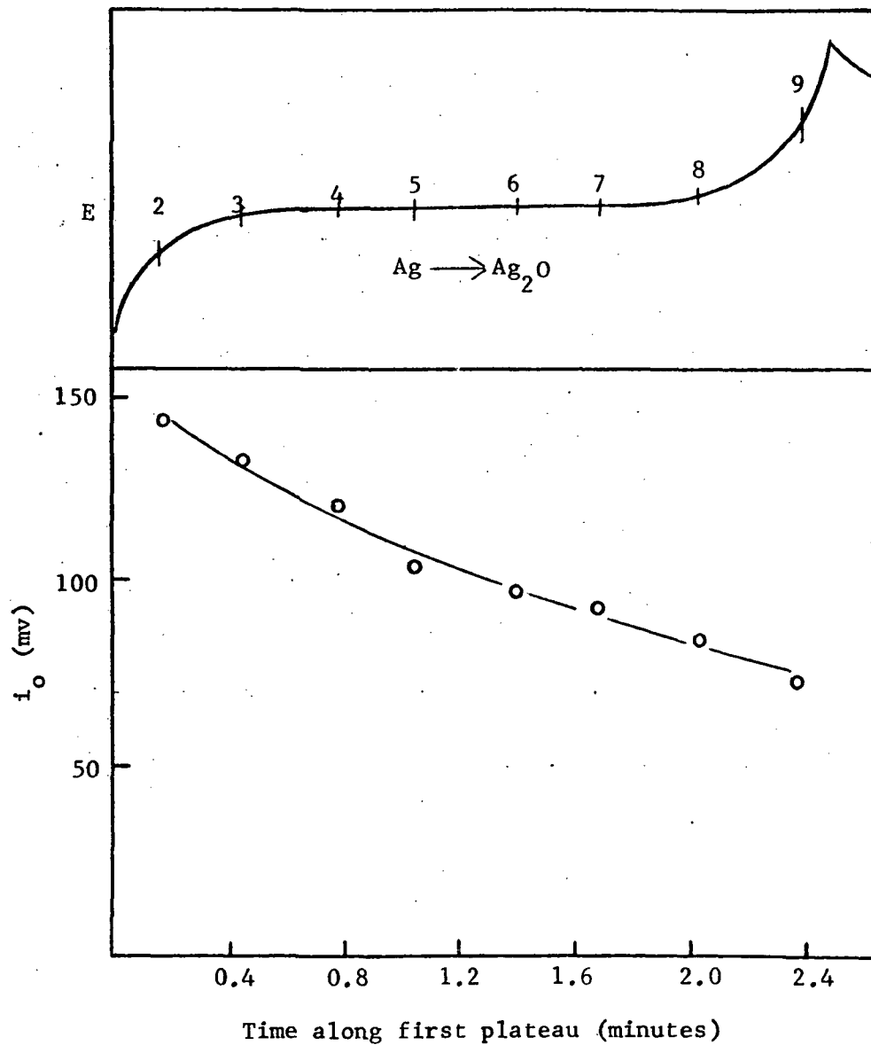
Fig. 9--Plot of i_0 versus time along first oxidation plateau, with corresponding points marked on the potential-time curve. The numbers correspond to interruptions in the d.c. charging when the i_0 measurements were made.
