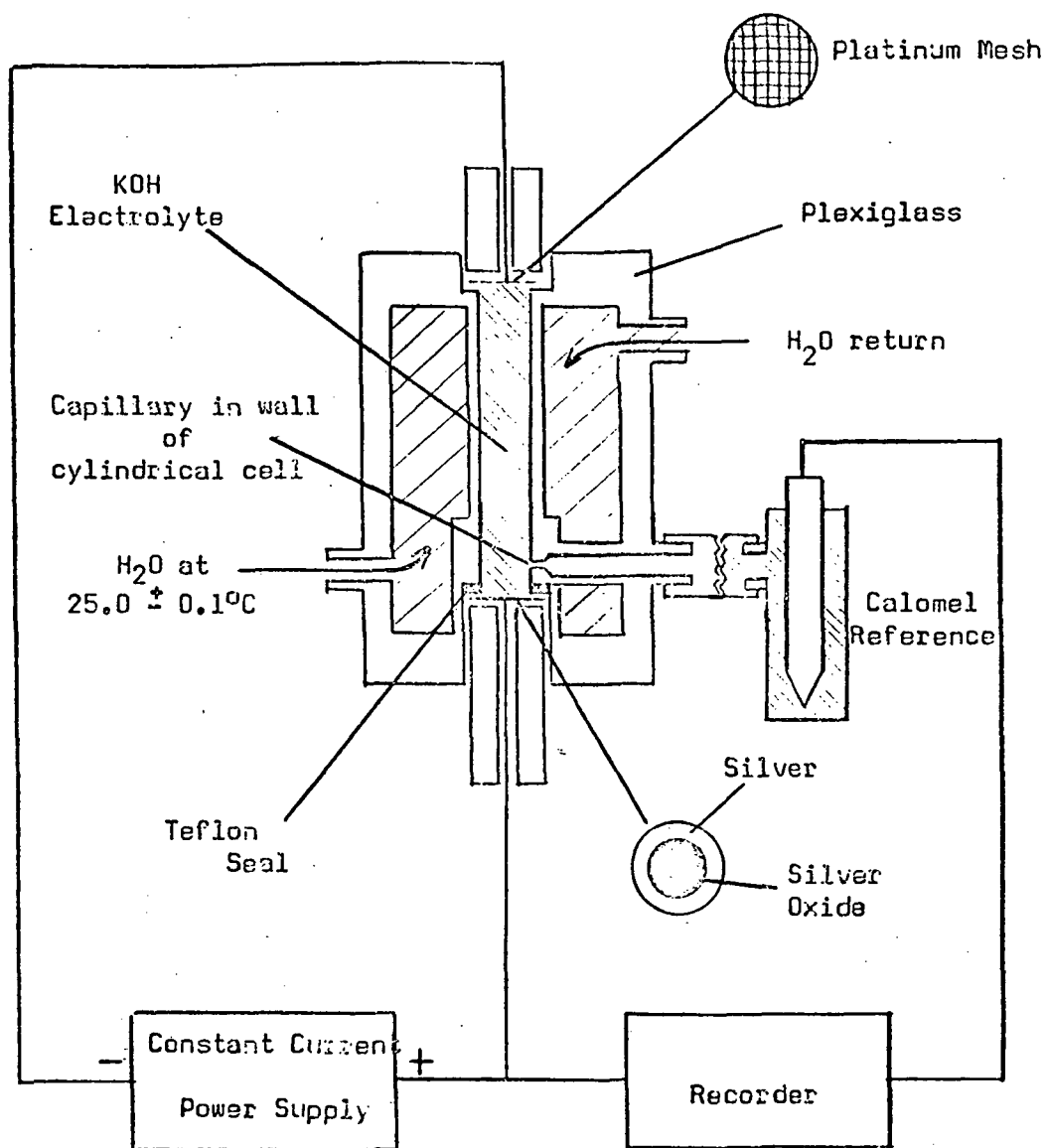
Fig. 13.--Apparatus for charge acceptance data from which the values of the ratio, i = Q_H / Q_{total} , were determined.
