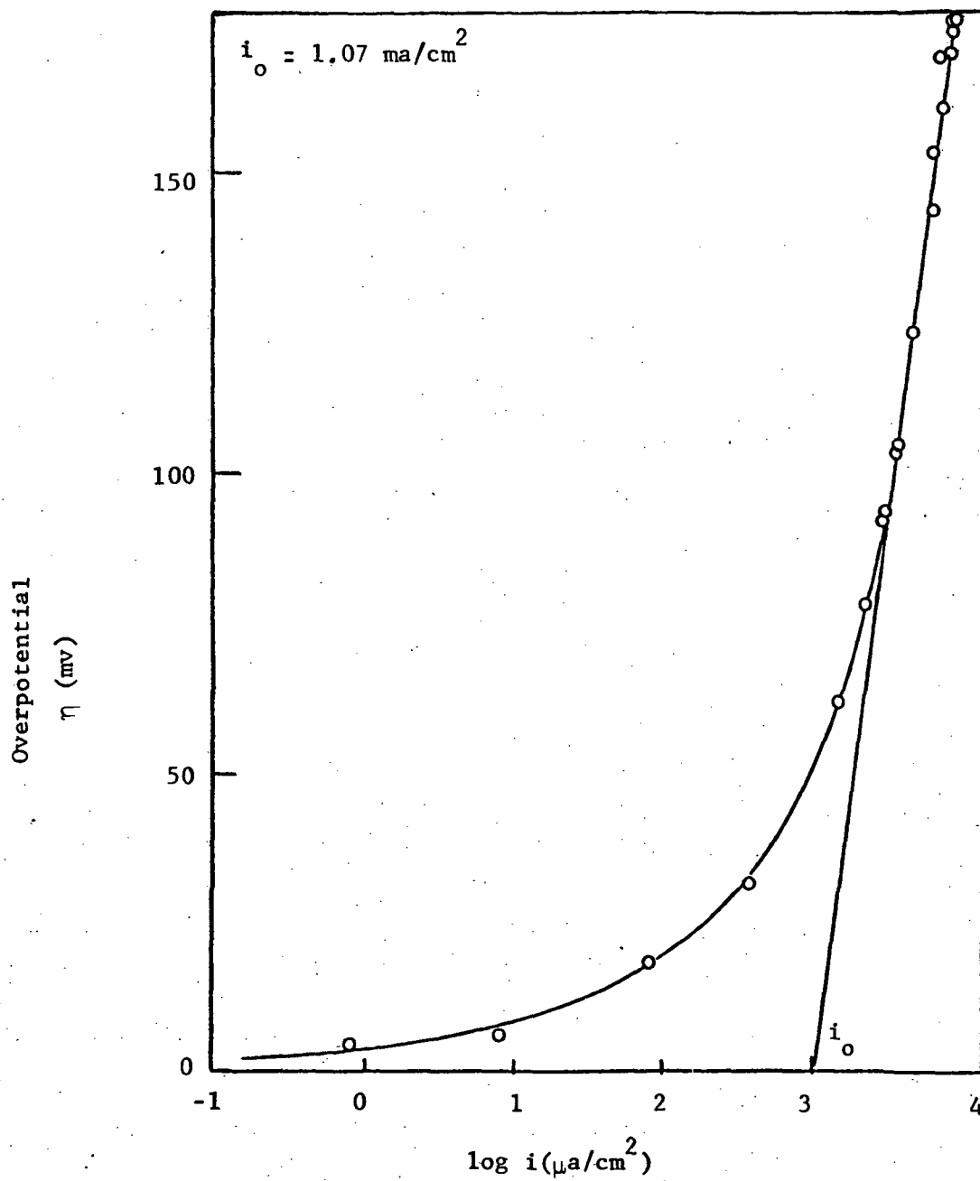
Fig. 5 --Tafel plot of galvanostatic polarization data for determination of i_0 .
