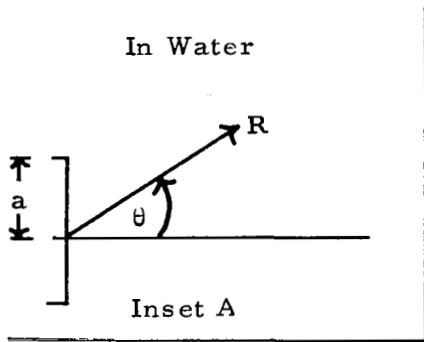
Insert A: Defines Coordinate System for Initial Wave from Transducer
