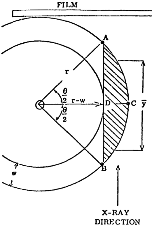
Figure 24. Geometry of Bond Line Separation
