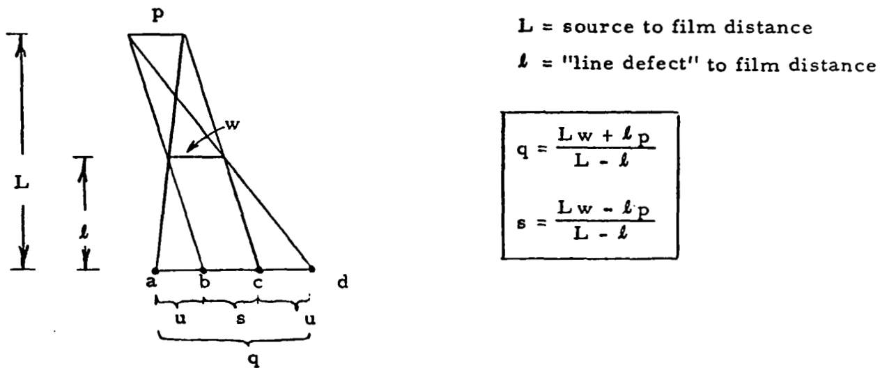
Figure 8. Geometric Unsharpness
