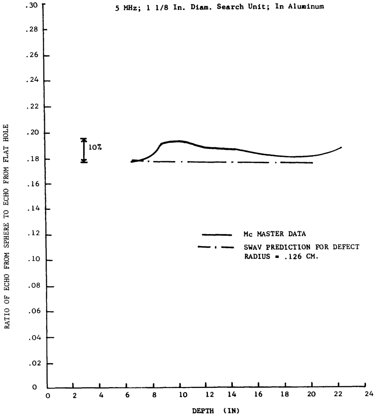
Figure 34. Echo Ratio vs. Distance - Contact Test
