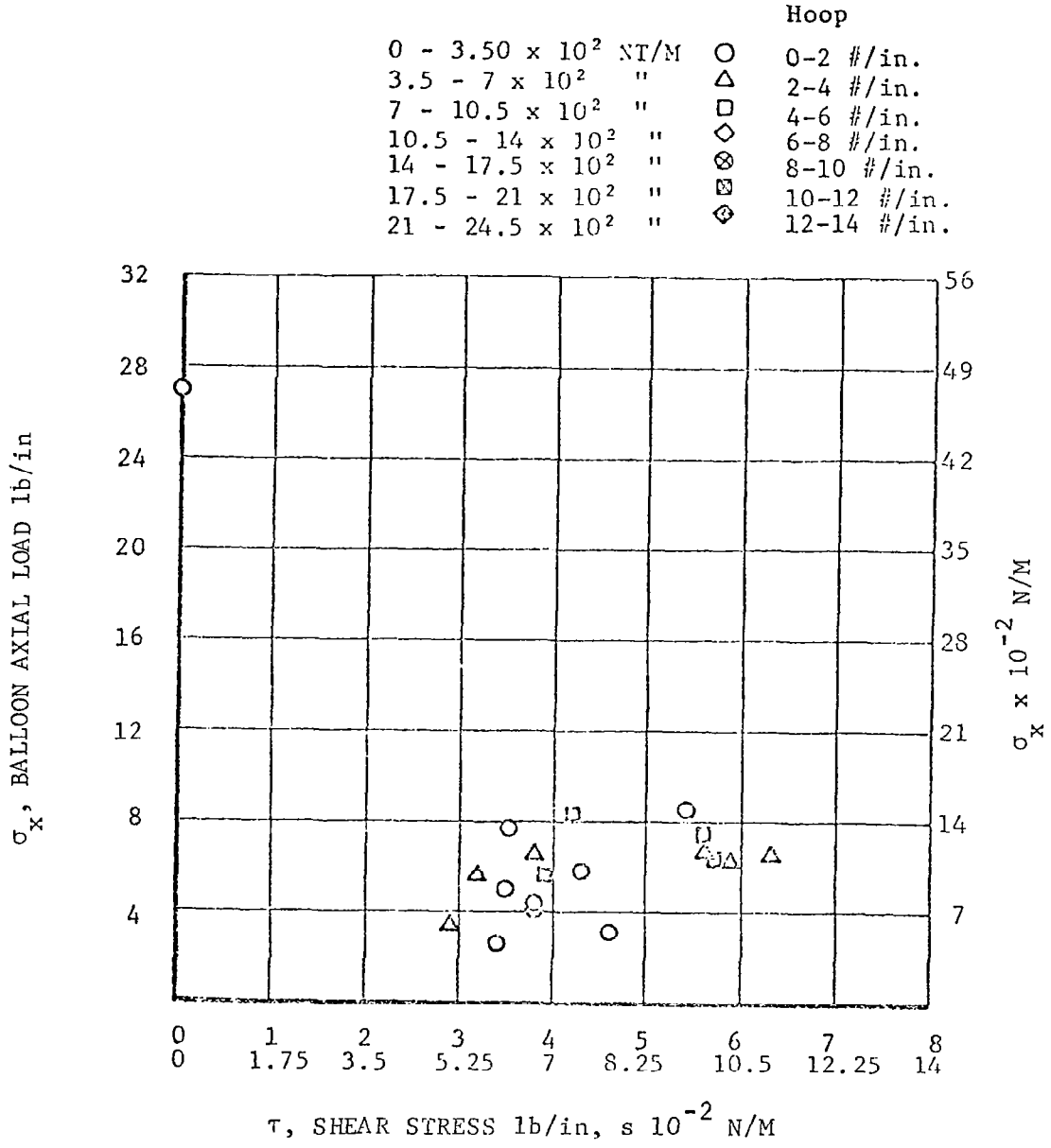
FIGURE 14 45° FTL MATERIAL ROLLER COATED YARNS
