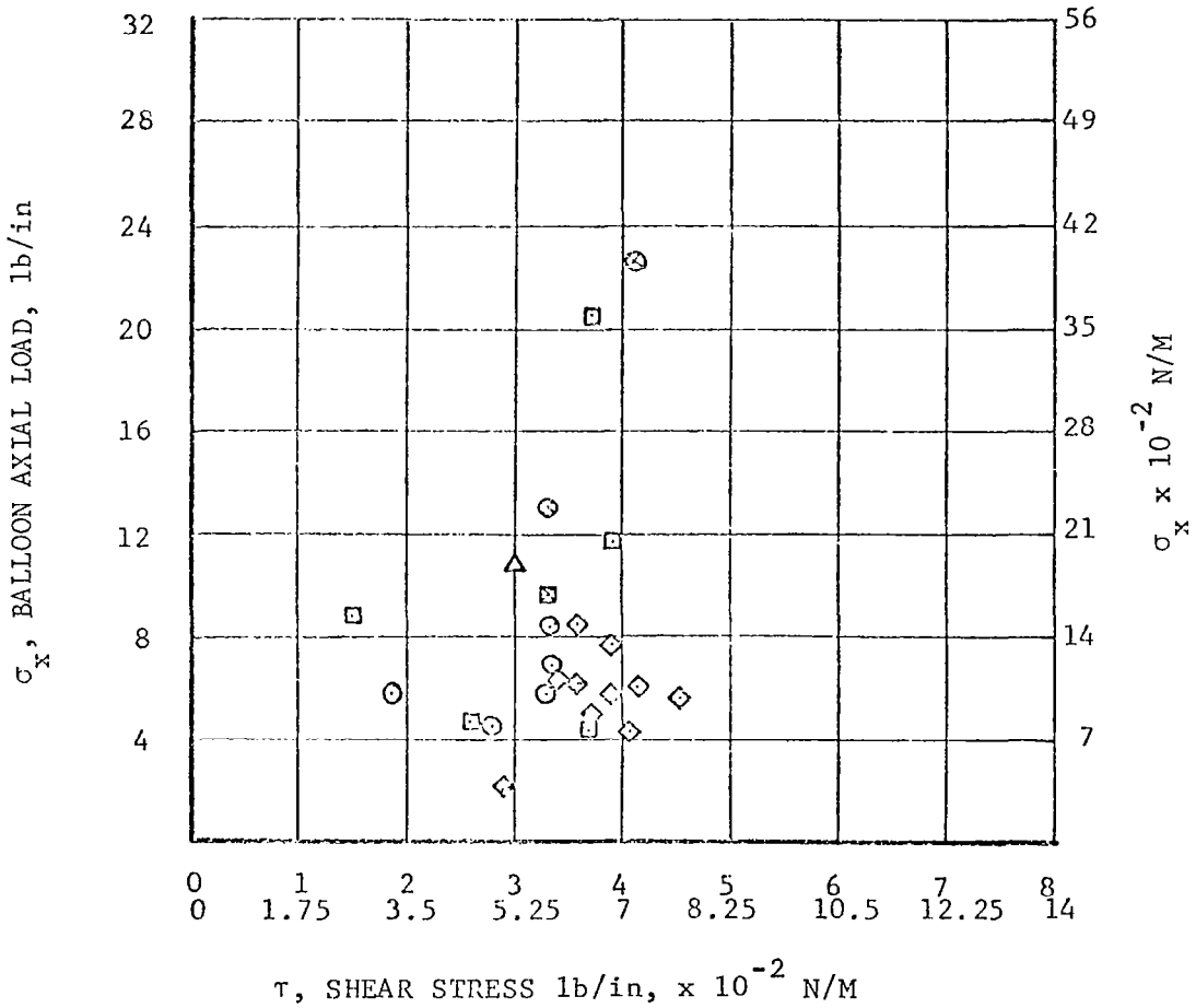
FIGURE 13 82° FTL MATERIAL ROLLER COATED YARN GT-111-4X MATERIAL
