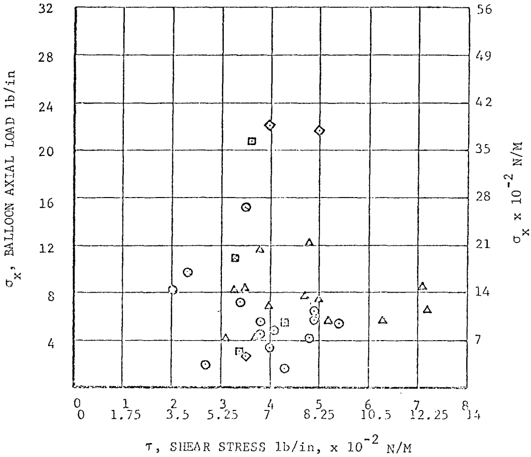
FIGURE 12 LENO WOVEN MESH MATERIAL PRECOATED MYLAR GT-11 MATERIAL
