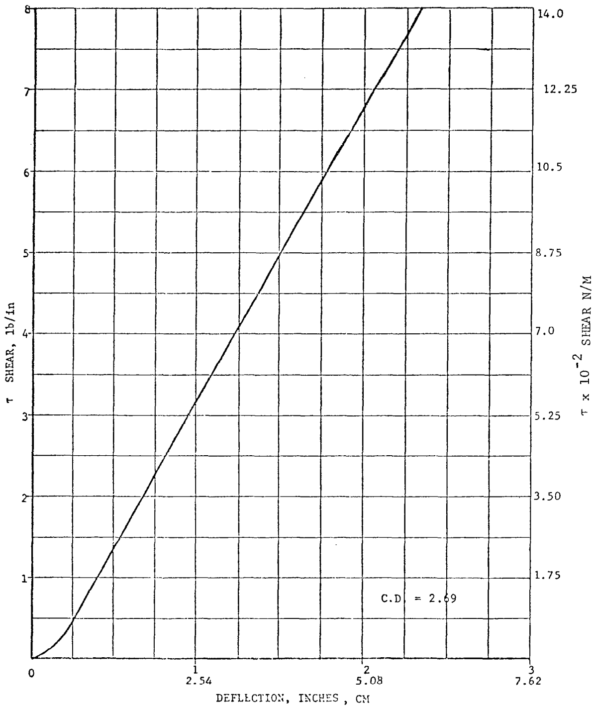
FIGURE 10 TORQUE CALIBRATION
