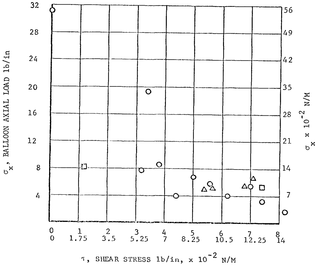
FIGURE 15 60° FTL MATERIAL - ROLLER COATED YARNS
