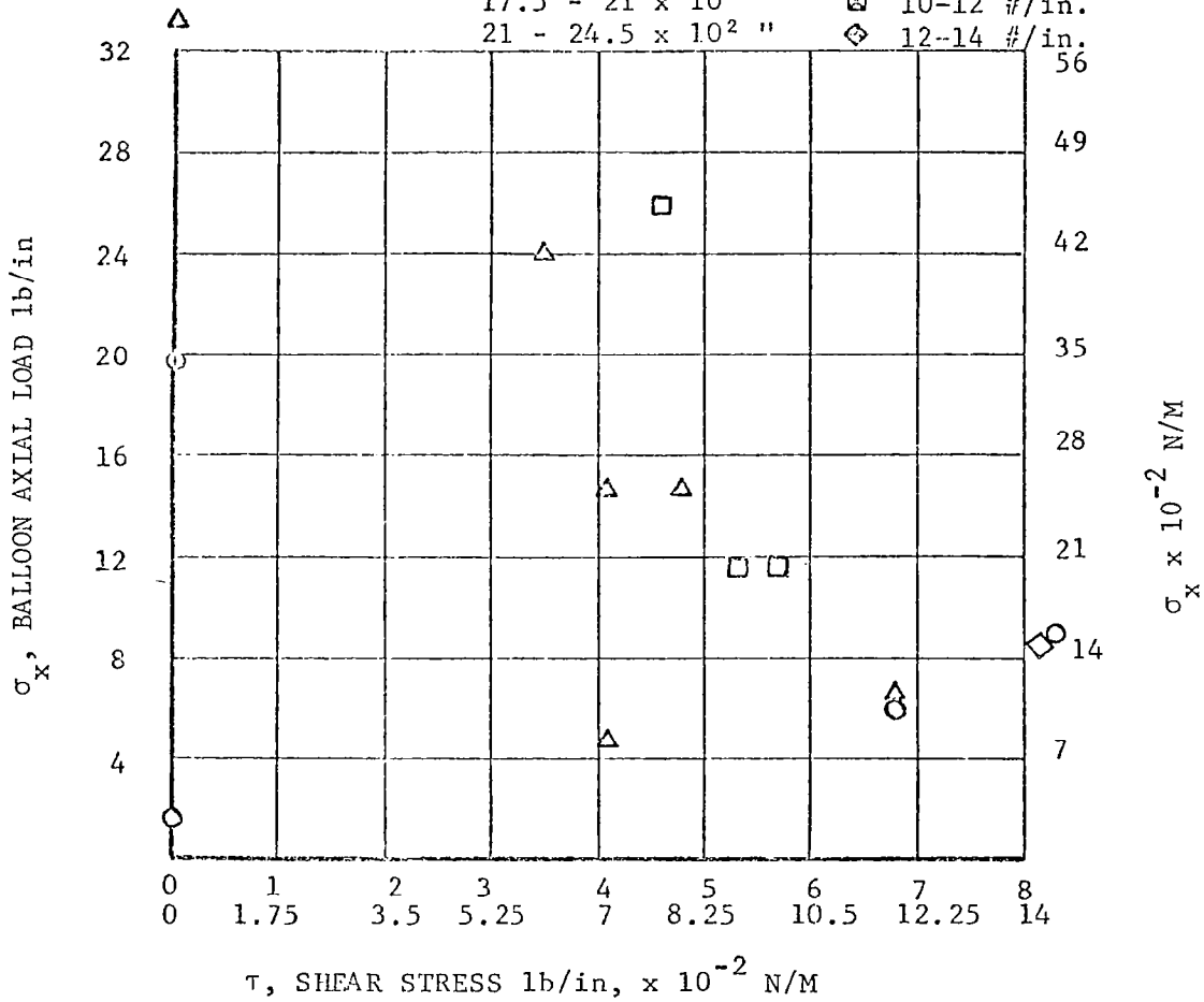
FIGURE 17 60° FTL MATERIAL - PRECOATED MYLAR POST COATED LAMINATE
