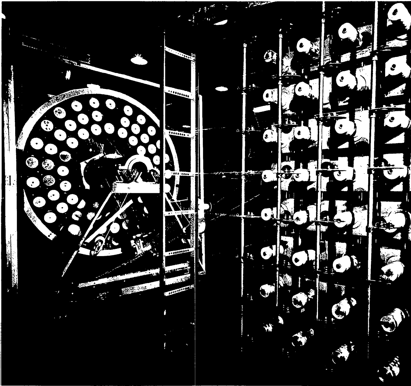
FIGURE 21, YARN DISPENSING DRUM AND CREEL SYS
